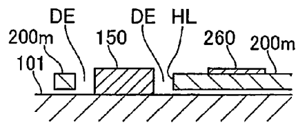
B-B CROSS SECTION
