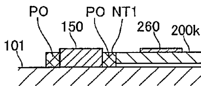
C-C CROSS SECTION
