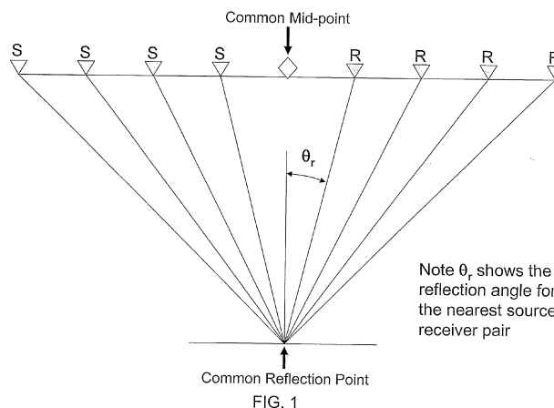
Schematic Diagram of a "CMP" Gather of Traces
