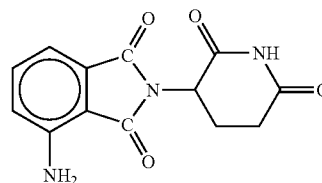
1,3-dioxo-2-(2,6-dioxopiperidin-3-yl)-4-aminoisoindoline; and
