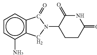
1-oxo-2-(2,6-dioxopiperidin-3-yl)-4-aminoisoindoline;
