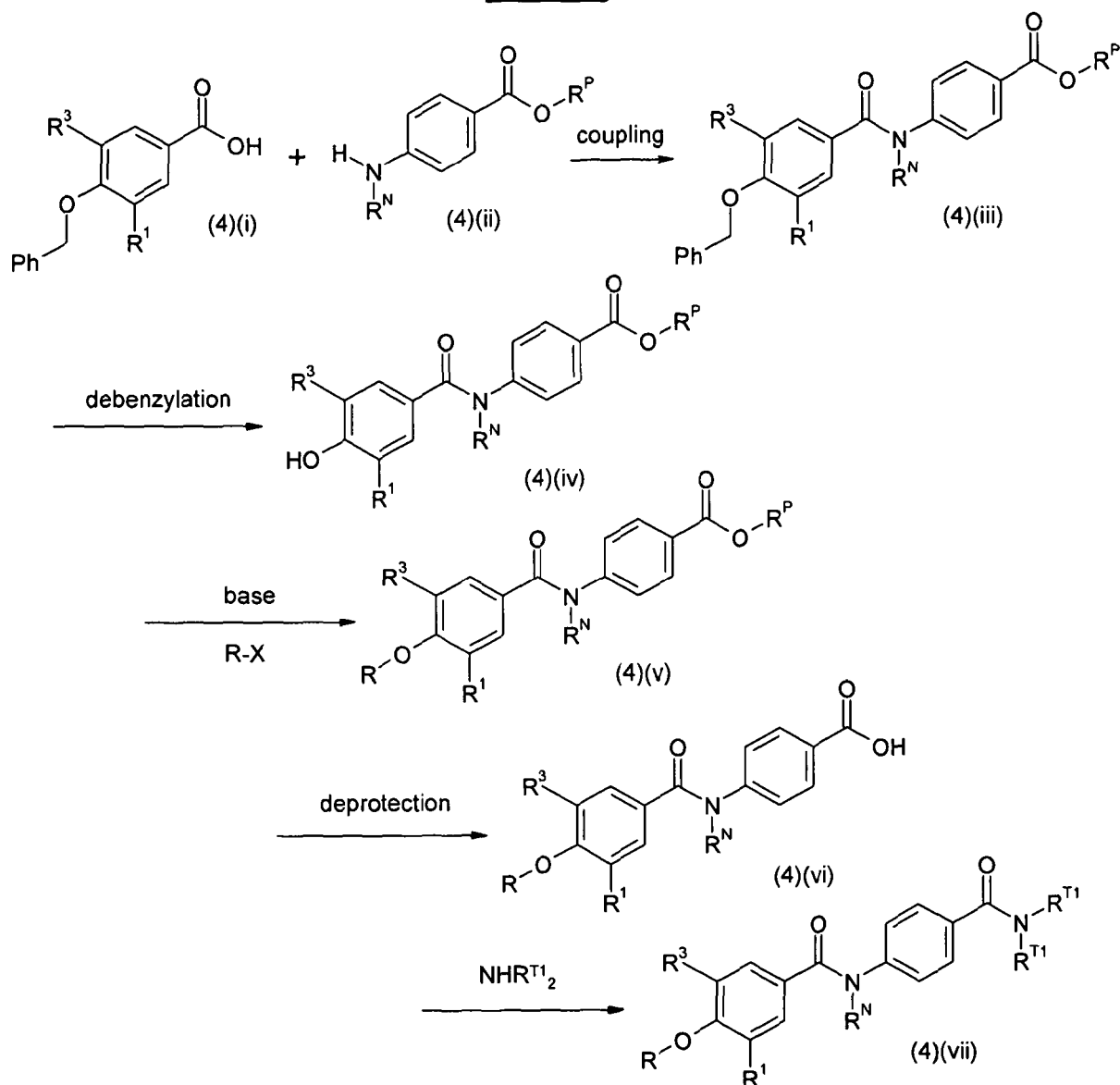
Scheme 4
