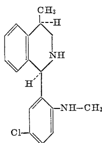
"cis" (as racemic mixture)
