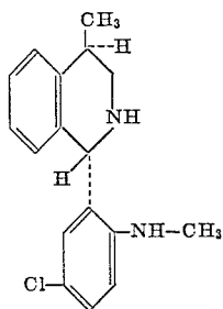
"trans" (as racemic mixture)
