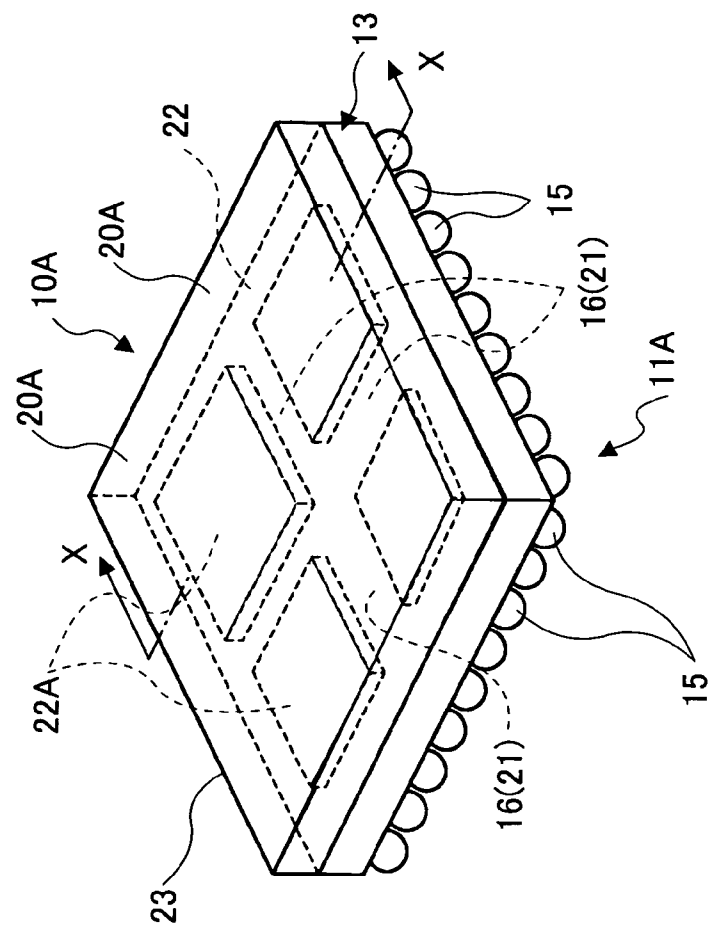
12A SEMICONDUCTOR DEVICE UNIT
