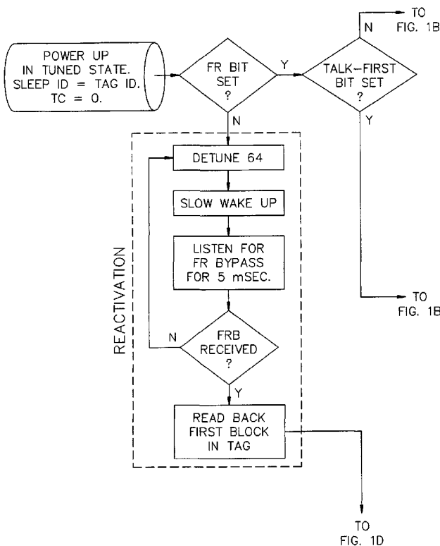
ANTI-COLLISION FLOWCHART
