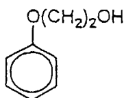
(Ab-3) Antiseptic
