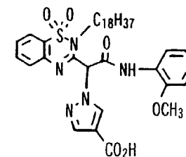
Coupler (129)
