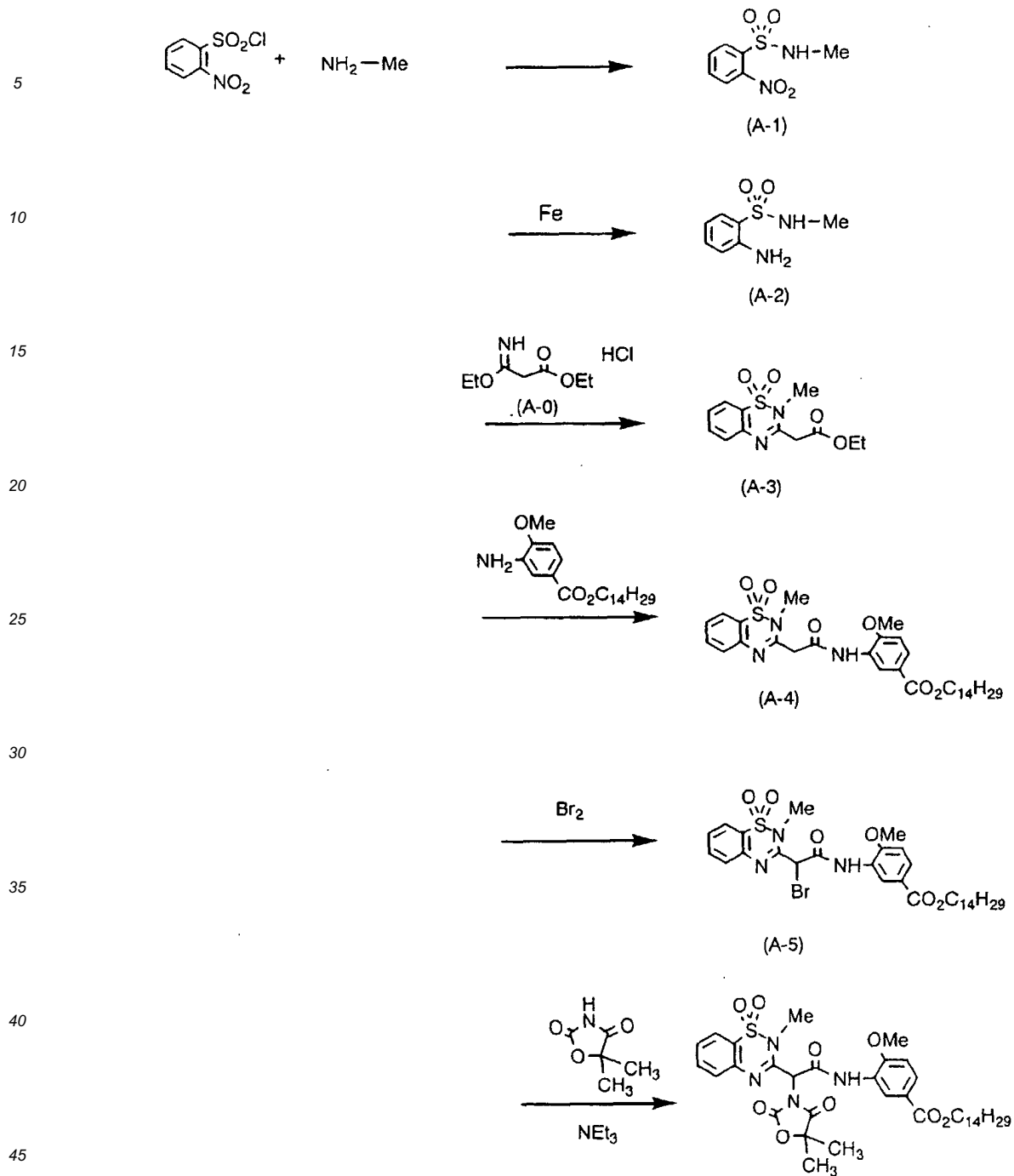
Coupler (1)
