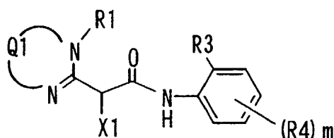
formula (I-2)
