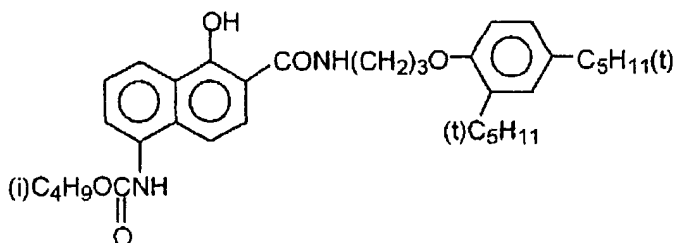
ExC-4
