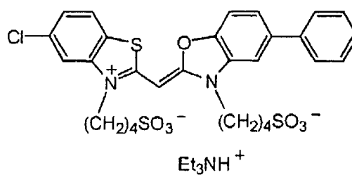
Sensitizing dye 10
