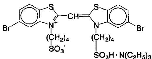
Spectral sensitizing dye-2
