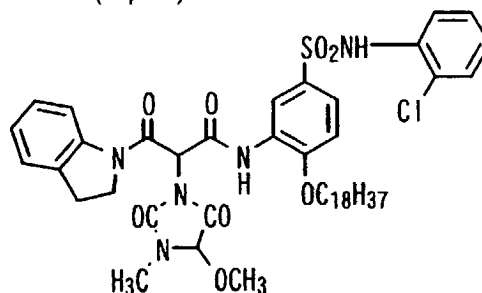
Dye for comparison (Cp-1)
