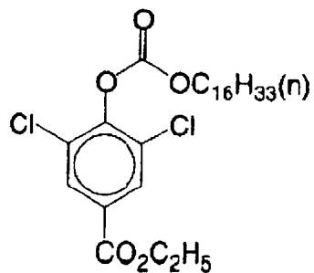
30 (C p d - 9) Color-image stabilizer
