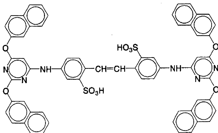
(Compound I)
