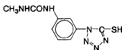
Mercapto compound-2
