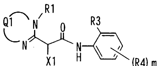
formula (I-2)
