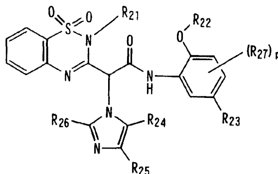
formula (IIB)
