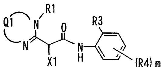
formula (I-2)
