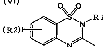
formula (VI)
