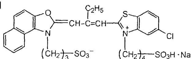
Sensitizing dye 1
