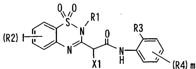
formula (II-2)
