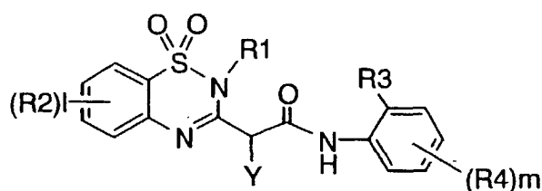
formula (II)
