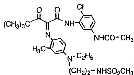
VR-1 A model of a dye for comparison (CD-1)
