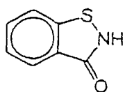
(Ab-1) Antiseptic
