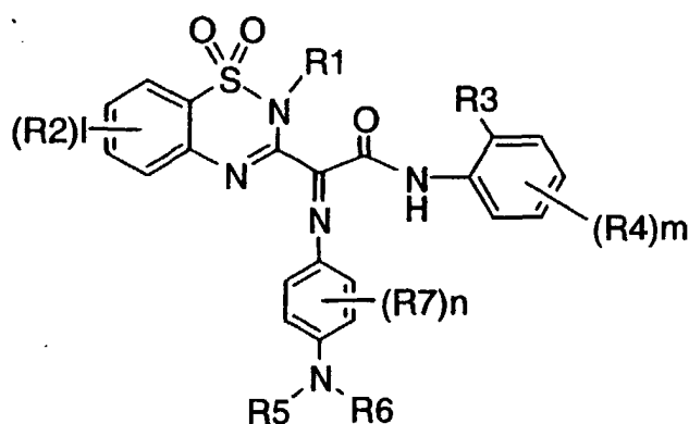
formula (III)
