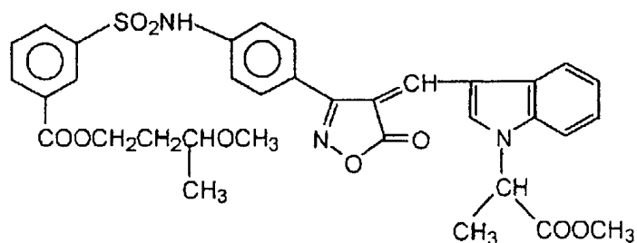
ExF-6
