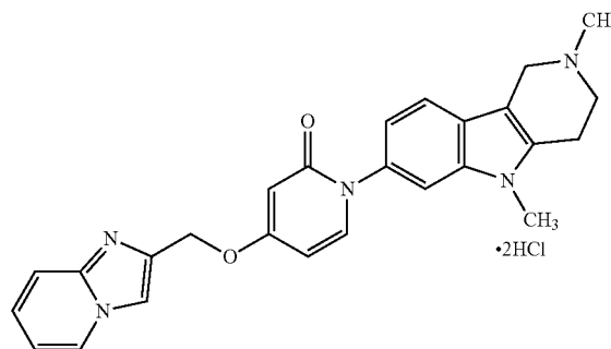
Chemical Formula: C 26 H 27 Cl 2 N 5 O 2 Exact Mass: 511.15 Molecular Weight: 512.43
