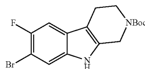
Chemical Formula: C 16 H 18 BrFN 2 O 2 Exact Mass: 368.05 Molecular Weight: 369.23
