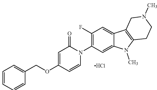
Chemical Formula: C 25 H 25 ClFN 3 O 2 Exact Mass: 453.16 Molecular Weight: 453.94
