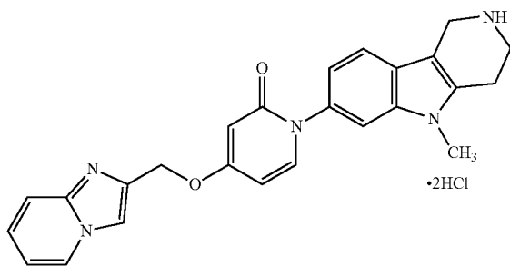
Chemical Formula: C 25 H 25 Cl 2 N 5 O 2 Exact Mass: 497.14 Molecular Weight: 498.40
