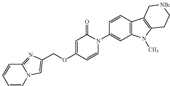
Chemical Formula: \text{C}_{30}\text{H}_{31}\text{N}_5\text{O}_4 Exact Mass: 525.24 Molecular Weight: 525.60
