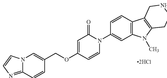
Chemical Formula: \text{C}_{25}\text{H}_{25}\text{Cl}_2\text{N}_5\text{O}_2 Exact Mass: 497.14 Molecular Weight: 498.40
