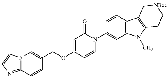
Chemical Formula: \text{C}_{30}\text{H}_{31}\text{N}_5\text{O}_4 Exact Mass: 525.24 Molecular Weight: 525.60
