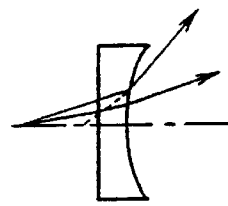
FIG. 68(E) PLANO-CONVEX ( PLANO-CONCAVE ) CYLINDRICAL LENS
