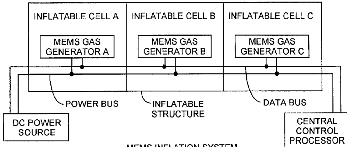
MEMS INFLATION SYSTEM
