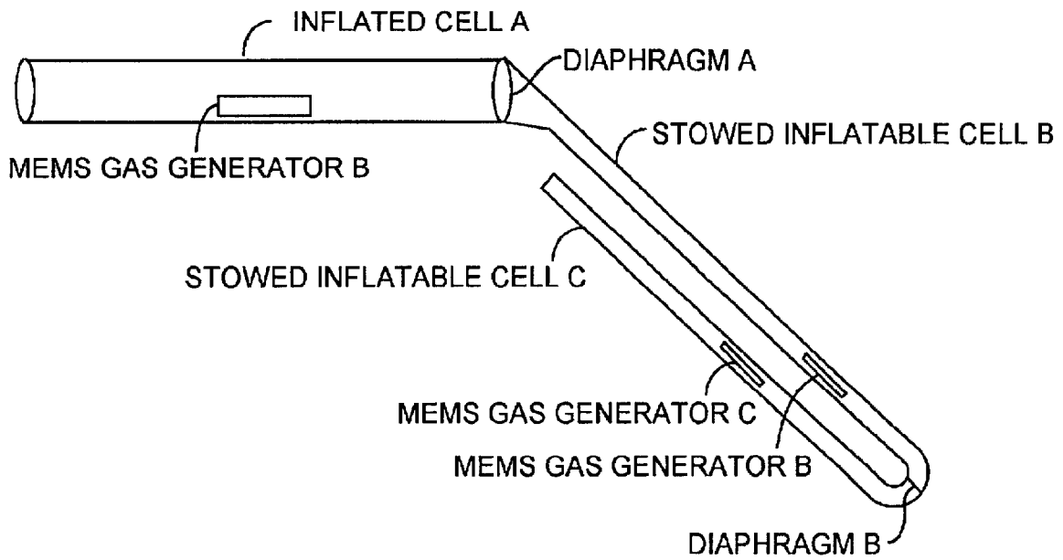
INFLATING INFLATABLE STRUCTURE
