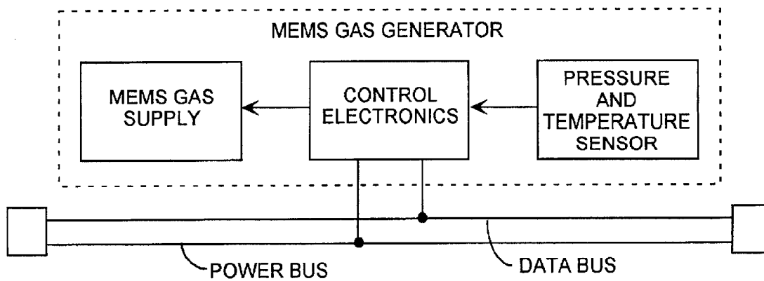
MEMS GAS GENERATOR
