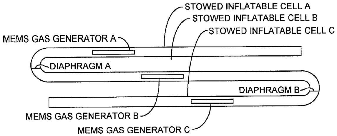
STOWED INFLATABLE STRUCTURE
