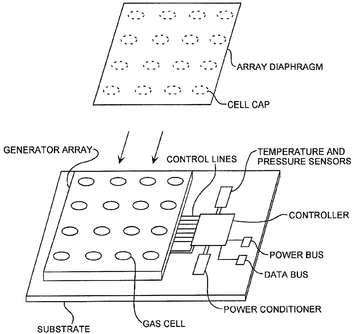
MEMS GAS GENERATOR
