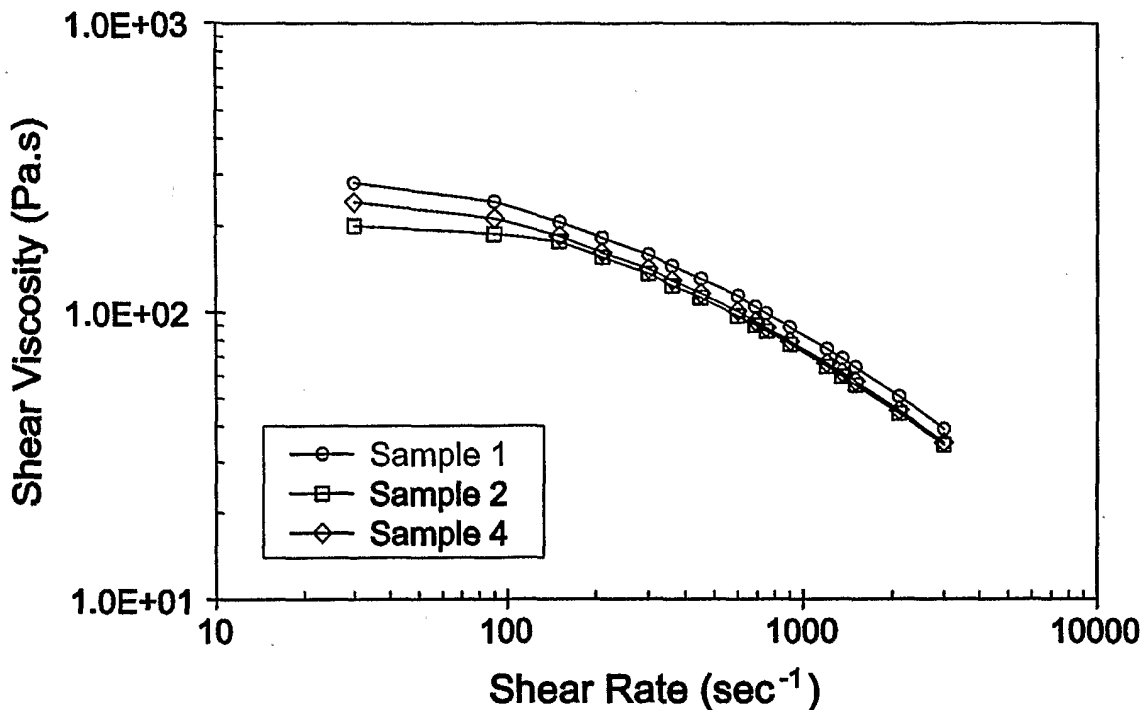
Fig. 11 Shear Viscosity of Plasticized Metallocene Propylene Homopolymers
