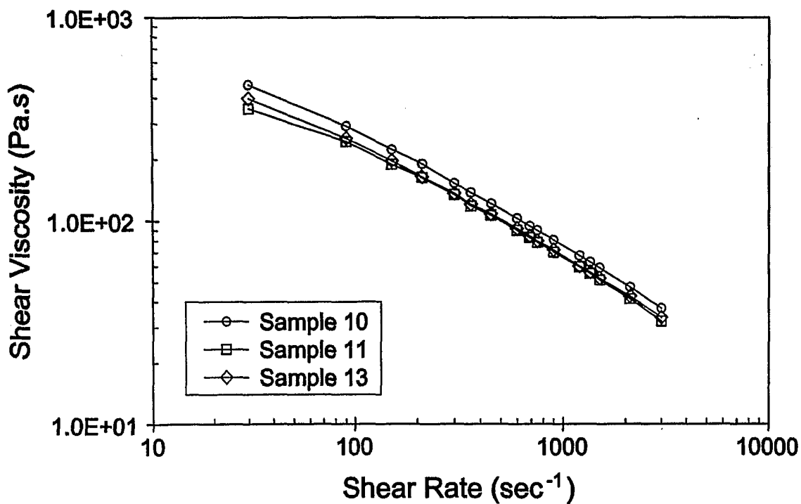
Fig. 12 Shear Viscosity of Plasticized Propylene Random Copolymers
