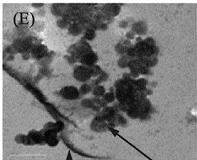
Outer surface Entrapped virus FIGURE . 2E
