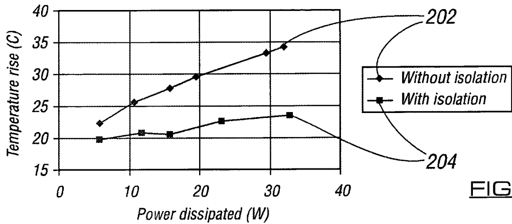
Temperature rise of HDD motor versus power dissipated
