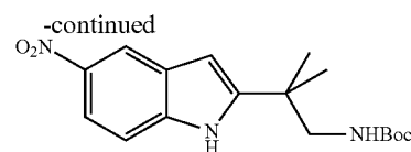
tert-Butyl 2-methyl-2-(5-nitro-1H-indol-2-yl)propylcarbamate
