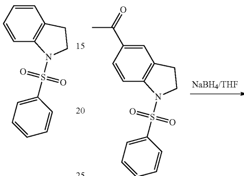
1-(Phenylsulfonyl)indoline
