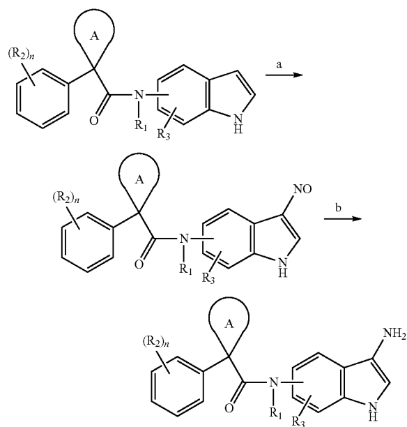
Scheme 34
