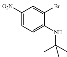
(2-Bromo-4-nitro-phenyl)-tert-butyl-amine
