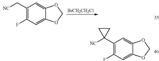
1-(6-Fluoro-benzo[1,3]dioxol-5-yl)-cyclopropanecarbonitrile
