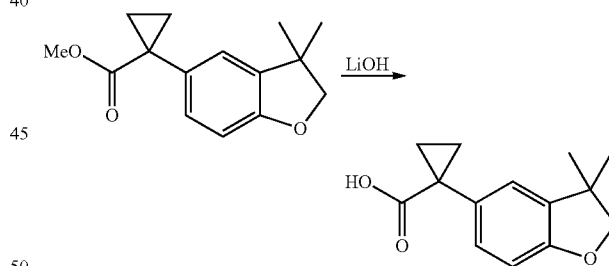
1-(3,3-Dimethyl-2,3-dihydrobenzofuran-5-yl)cyclopropanecarboxylic acid
