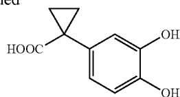
1-(3,4-Dihydroxy-phenyl)-cyclopropanecarboxylic acid
