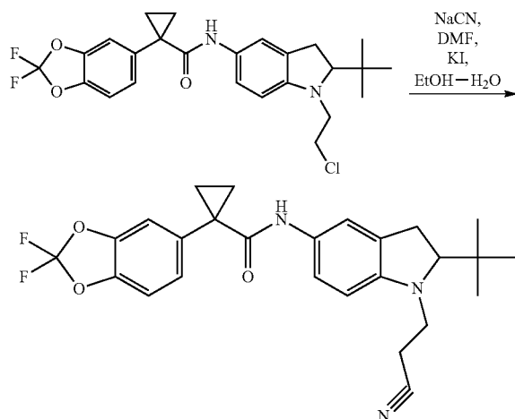
N-(2-tert-Butyl-1-(2-cyanoethyl)indolin-5-yl)-1-(2,2-difluorobenzo[d][1,3]dioxol-5-yl)cyclopropanecarboxamide
