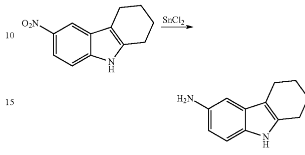
2,3,4,9-Tetrahydro-1H-carbazol-6-amine
