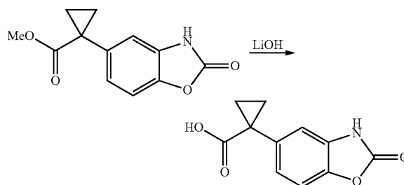
1-(2-Oxo-2,3-dihydrobenzo[d]oxazol-5-yl)cyclopropanecarboxylic acid
