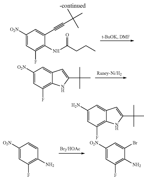
2-Bromo-6-fluoro-4-nitro-phenylamine
