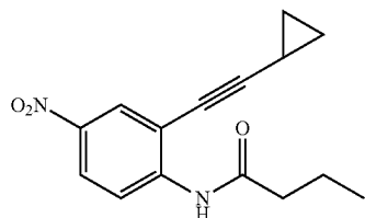
N-(2-(Cyclopropylethynyl)phenyl)-4-nitrobutyramide
