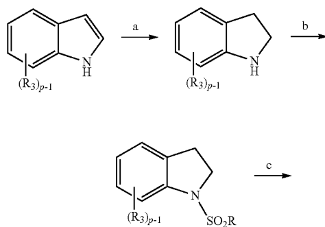
Scheme 14
