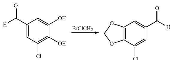
7-Chlorobenzo[d][1,3]dioxole-5-carbaldehyde
