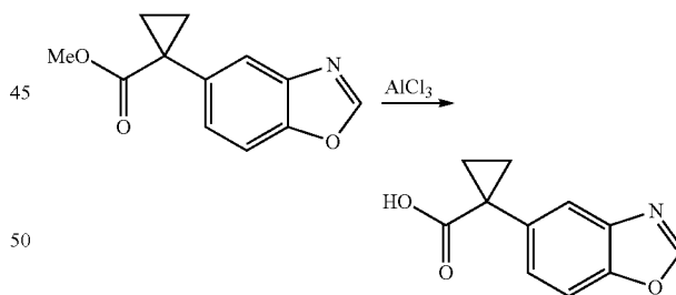
1-(Benzo[d]oxazol-5-yl)cyclopropanecarboxylic acid
