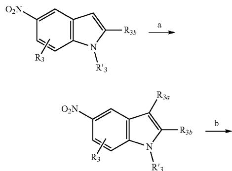
Scheme 28
