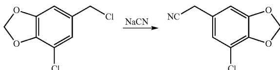
2-(7-Chlorobenzo[d][1,3]dioxol-5-yl)acetonitrile
