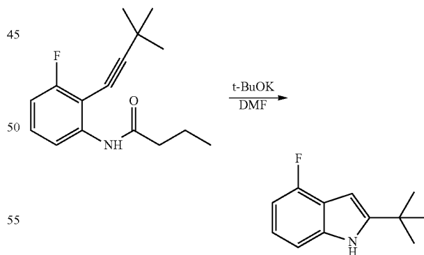
2-tert-Butyl-4-fluoro-1H-indole
