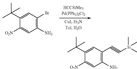
4-tert-Butyl-5-nitro-2-trimethylsilanylethynyl-phenylamine
