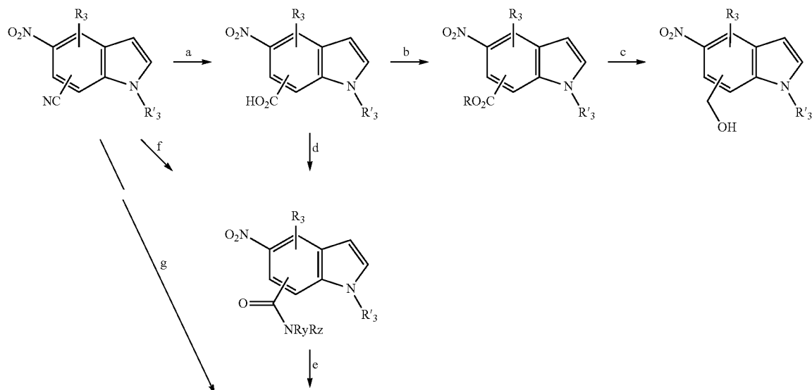
Scheme 30
