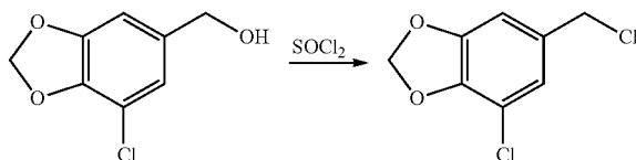
4-Chloro-6-(chloromethyl)benzo[d][1,3]dioxole
