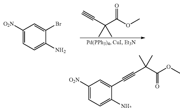
Methyl
