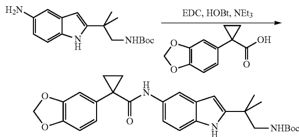
tert-Butyl 2-(5-(1-(benzo[d][1,3]dioxol-5-yl)cyclopropanecarboxamido)-1H-indol-2-yl)-2-methylpropylcarbamate
