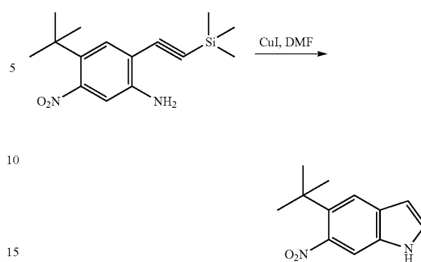
5-tert-Butyl-6-nitro-1H-indole
