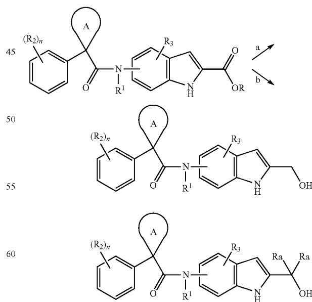
Scheme 33
