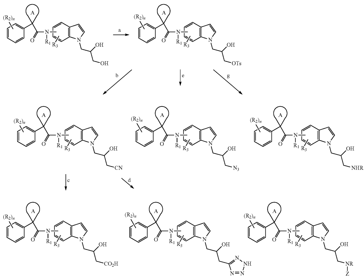
Scheme 40
