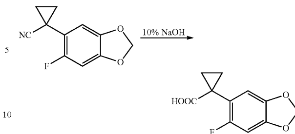
1-(6-Fluoro-benzo[1,3]dioxol-5-yl)-cyclopropanecarboxylic acid
