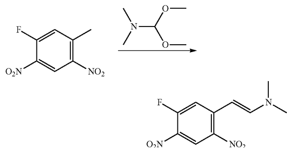
(E)-2-(5-Fluoro-2,4-dinitrophenyl)-N,N-dimethylethenamine
