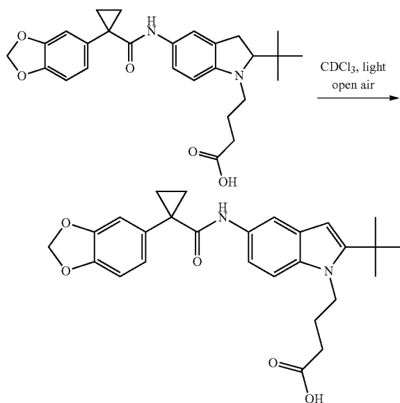
4-(5-(1-(Benzo[d][1,3]dioxol-5-yl)cyclopropanecarboxamido)-2-tert-butyl-1H-indol-1-yl)butanoic acid
