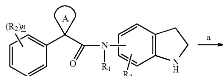
Scheme 41
