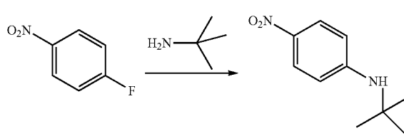
N-tert-Butyl-4-nitroaniline
