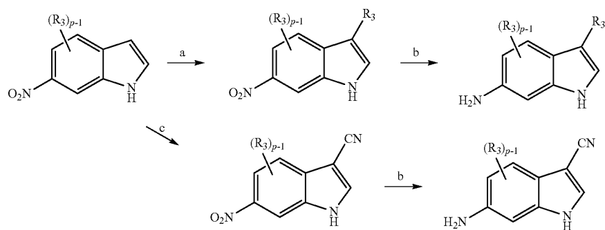
Scheme 15
