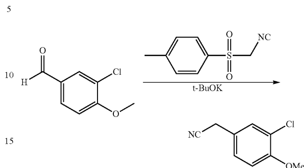
2-(3-Chloro-4-methoxyphenyl)acetonitrile
