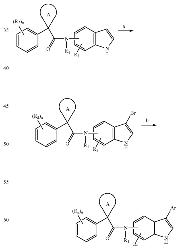
Scheme 37
