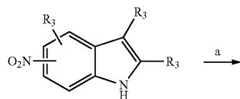
Scheme 16
