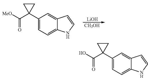
1-(1H-Indol-5-yl)cyclopropanecarboxylic acid
