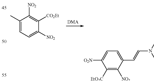
(E)-Ethyl 3-(2-(dimethylamino)vinyl)-2,6-dinitrobenzoate
