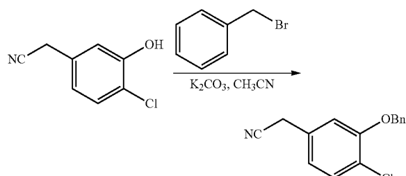
2-(3-(Benzyloxy)-4-chlorophenyl)acetonitrile
