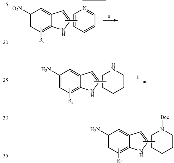
Scheme 29
