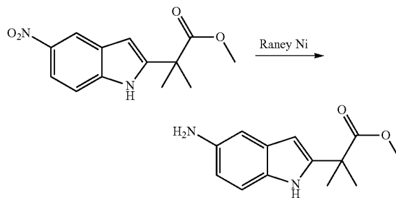
Methyl
