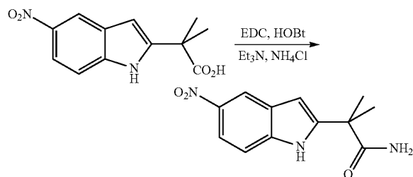
2-Methyl-2-(5-nitro-1H-indol-2-yl)propanamide
