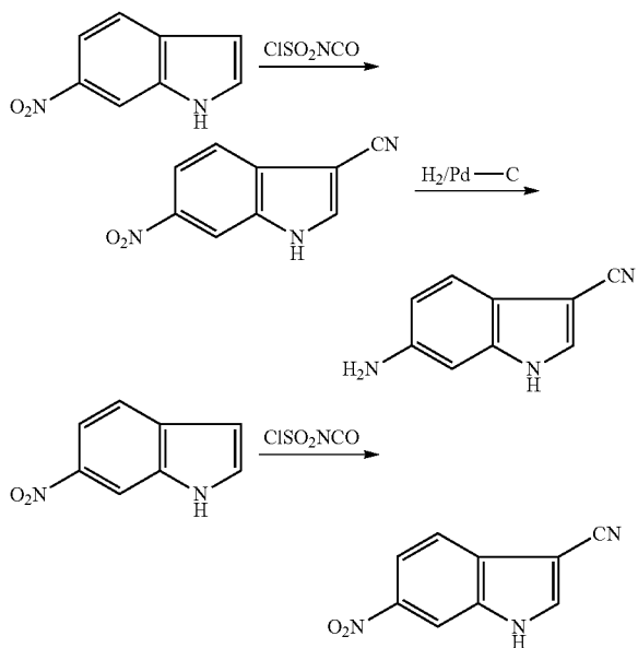
6-Nitro-1H-indole-3-carbonitrile
