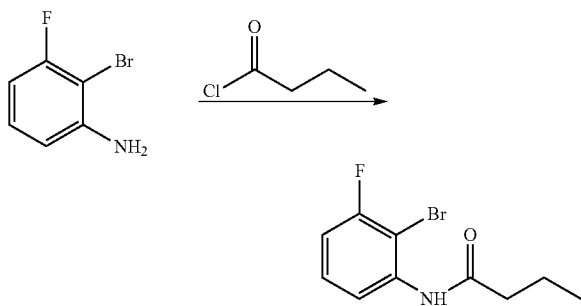
N-(2-Bromo-3-fluorophenyl)butyramide
