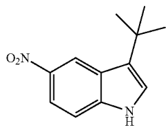
3-tert-Butyl-5-nitro-1H-indole
