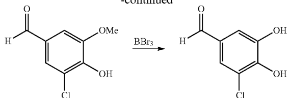
3-Chloro-4,5-dihydroxybenzaldehyde
