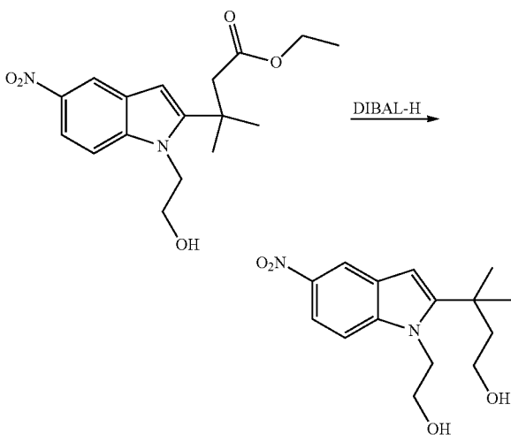
3-[1-(2-Hydroxy-ethyl)-5-nitro-1H-indol-2-yl]-3-methyl-butan-1-ol
