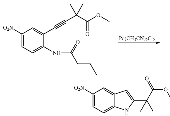
Methyl
