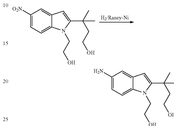
3-[5-Amino-1-(2-hydroxy-ethyl)-1H-indol-2-yl]-3-methyl-butan-1-ol
