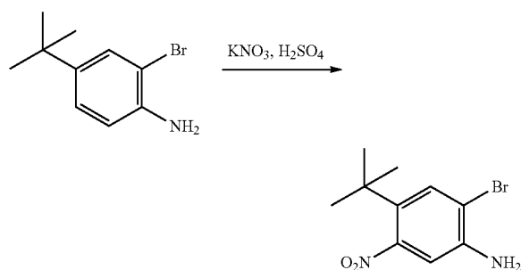
2-Bromo-4-tert-butyl-5-nitro-phenylamine
