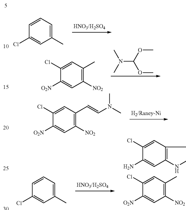
1-Chloro-5-methyl-2,4-dinitrobenzene
