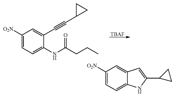
2-Cyclopropyl-5-nitro-1H-indole
