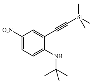
tert-Butyl-(4-nitro-2-trimethylsilylethynyl-phenyl)-amine
