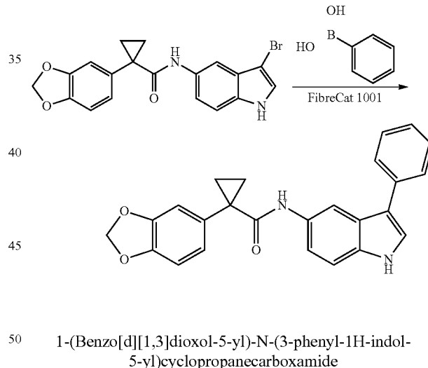
1-(Benzo[d][1,3]dioxol-5-yl)-N-(3-phenyl-1H-indol-5-yl)cyclopropane carboxamide
