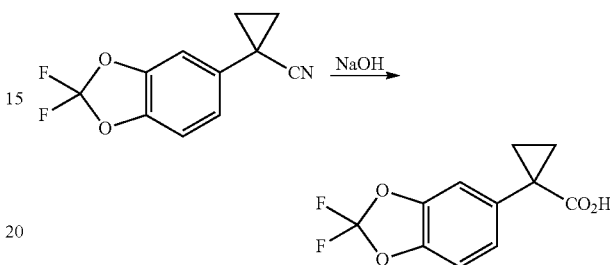
1-(2,2-Difluoro-benzo[1,3]dioxol-5-yl)-cyclopropanecarboxylic acid
