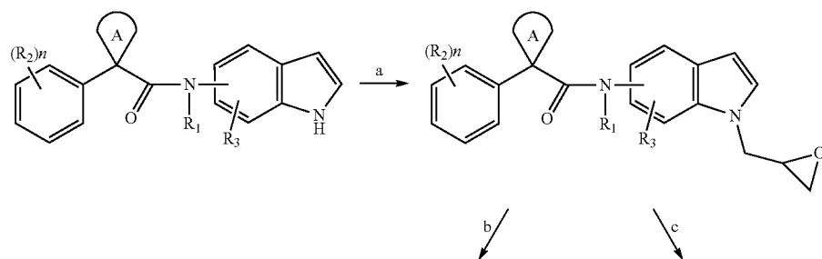
Scheme 39
