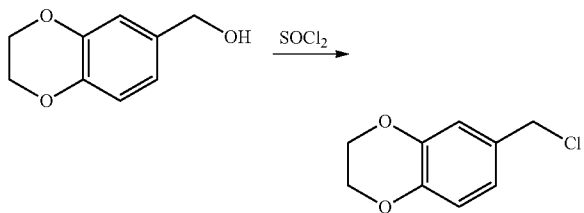
6-Chloromethyl-2,3-dihydro-benzo[1,4]dioxine
