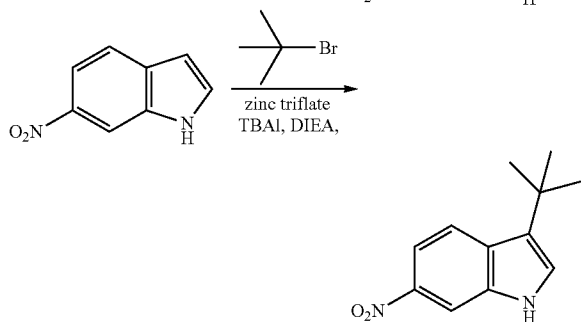
3-tert-Butyl-6-nitro-1H-indole
