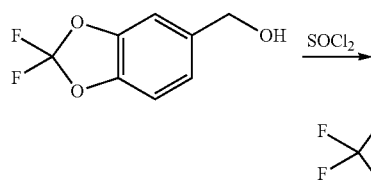
5-Chloromethyl-2,2-difluoro-benzo[1,3]dioxole
