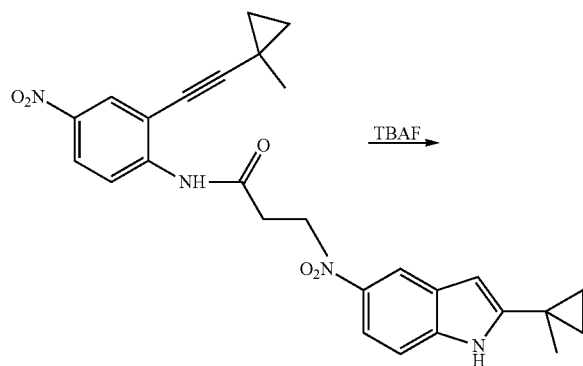
2-(1-Methylcyclopropyl)-5-nitro-1H-indole
