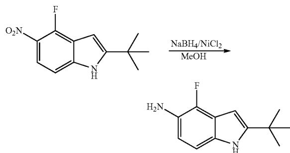
2-tert-Butyl-4-fluoro-1H-indol-5-amine
