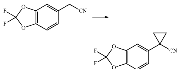
(2,2-Difluoro-benzo[1,3]dioxol-5-yl)-acetonitrile
