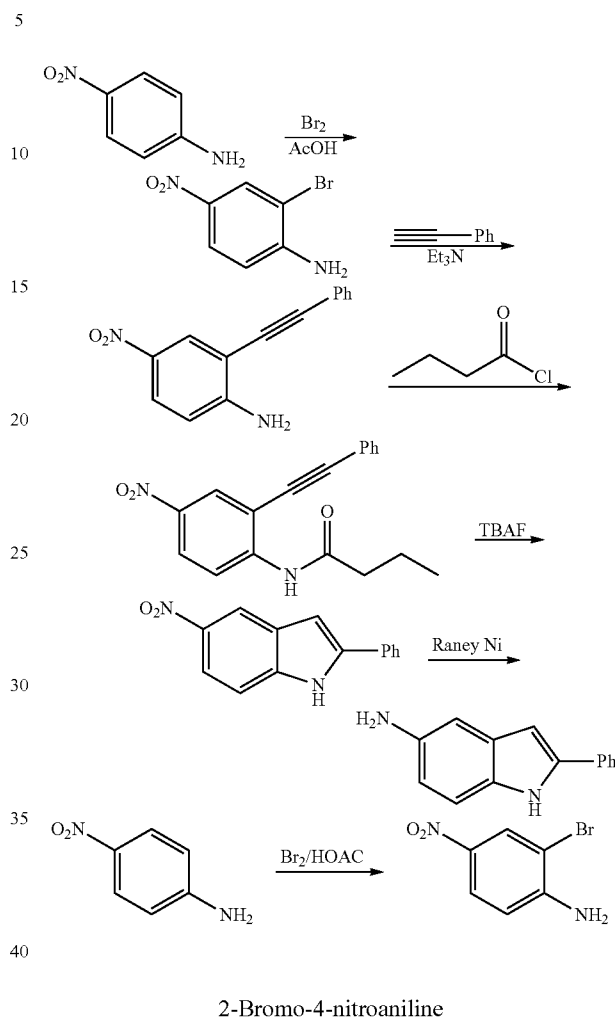
2-Bromo-4-nitroaniline
