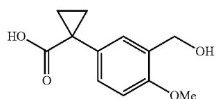
1-(3-Hydroxymethyl-4-methoxy-phenyl)-cyclopropanecarboxylic acid
