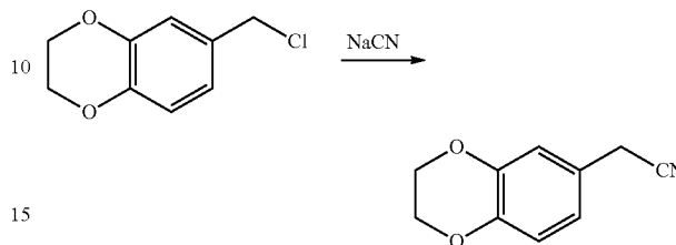
2-(2,3-Dihydrobenzo[b][1,4]dioxin-6-yl)acetonitrile
