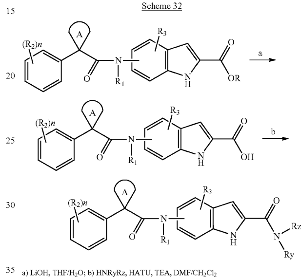
Scheme 32
