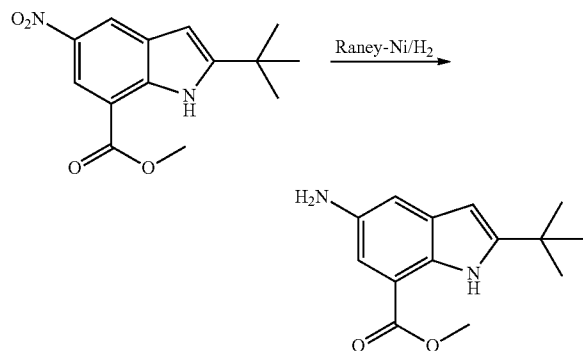
Methyl 5-amino-2-tert-butyl-1H-indole-7-carboxylate
