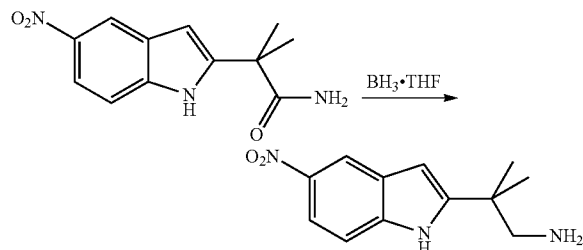
2-Methyl-2-(5-nitro-1H-indol-2-yl)propan-1-amine
