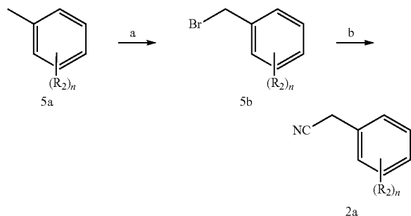
Scheme 5
