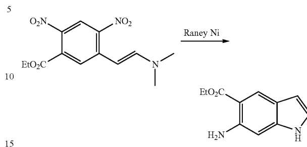
Ethyl 6-amino-1H-indole-5-carboxylate
