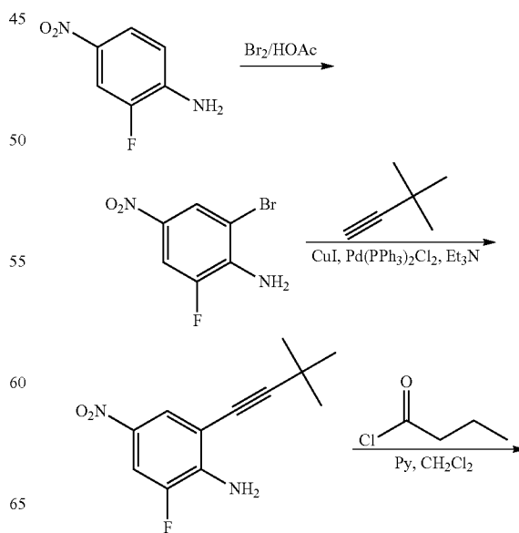
2-tert-Butyl-7-fluoro-1H-indol-5-amine
