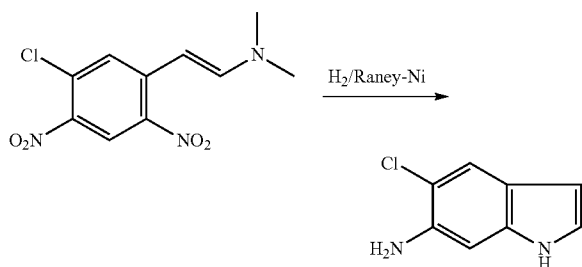
5-Chloro-1H-indol-6-amine
