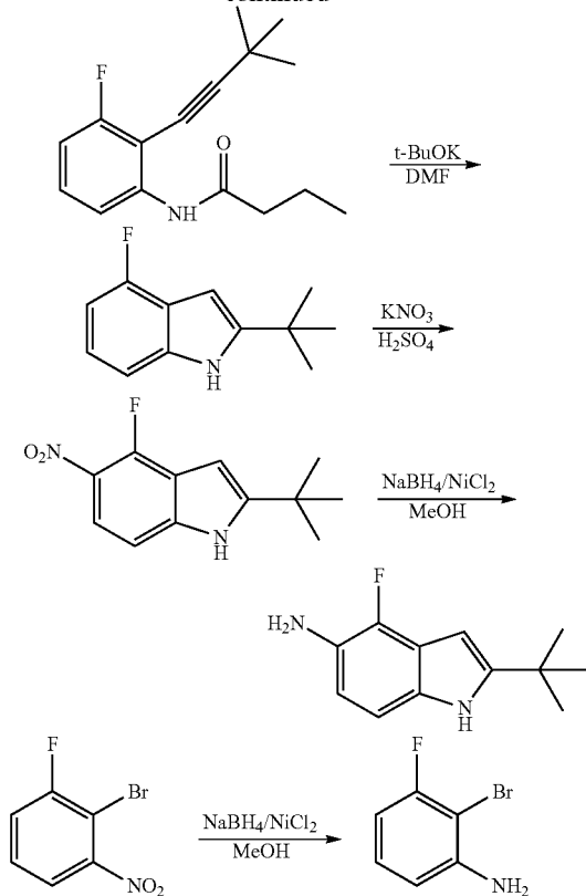
2-Bromo-3-fluoroaniline
