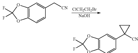
1-(2,2-Difluoro-benzo[1,3]dioxol-5-yl)-cyclopropanecarbonitrile
