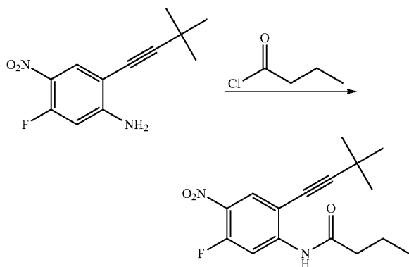
N-(2-(3,3-Dimethylbut-1-ynyl)-5-fluoro-4-nitrophenyl)butyramide
