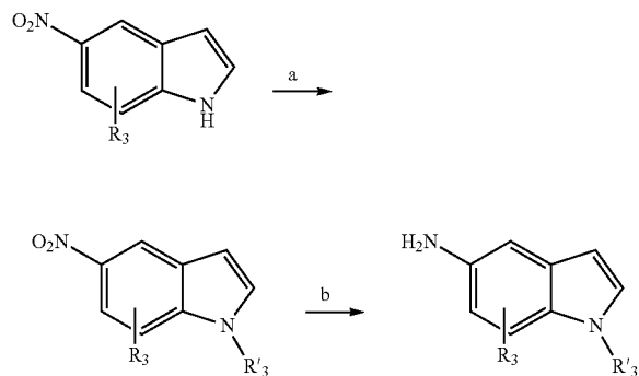
Scheme 27
