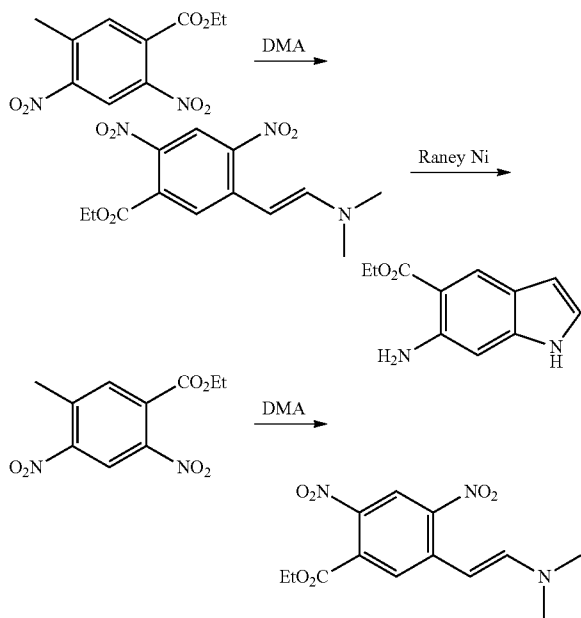
(E)-Ethyl 5-(2-(dimethylamino)vinyl)-2,4-dinitrobenzoate
