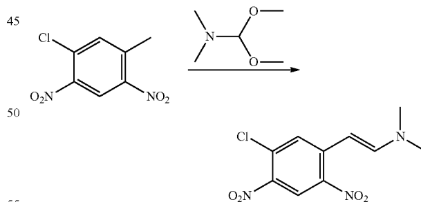
(E)-2-(5-Chloro-2,4-dinitrophenyl)-N,N-dimethylethenamine
