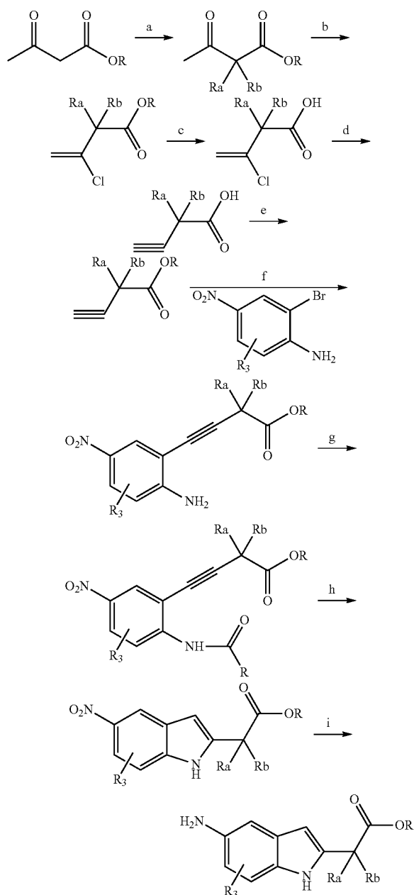
Scheme 31
