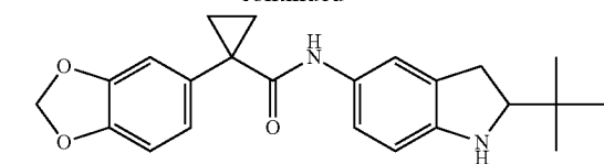
1-(Benzo[d][1,3]dioxol-5-yl)-N-(2-tert-butylindolin-5-yl)cyclopropanecarboxamide
