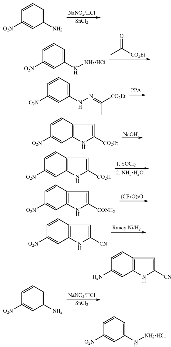
(3-Nitrophenyl)hydrazine hydrochloride
