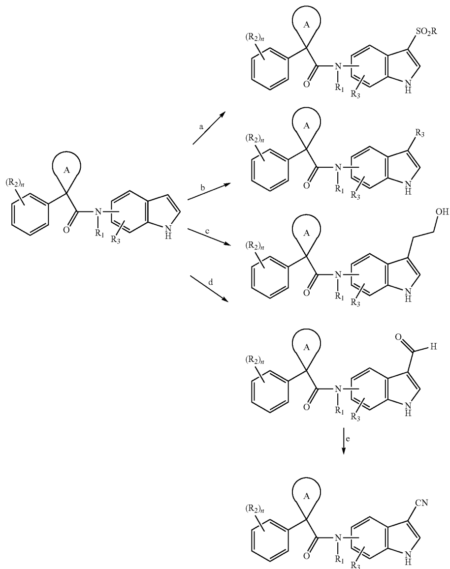
Scheme 38
