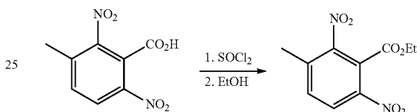
Ethyl 3-methyl-2,6-dinitrobenzoate
