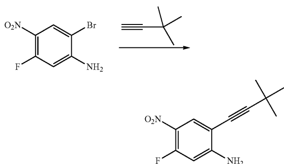
2-(3,3-Dimethylbut-1-ynyl)-5-fluoro-4-nitroaniline
