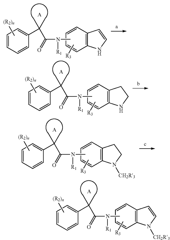
Scheme 35
