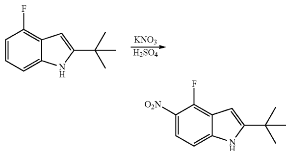
2-tert-Butyl-4-fluoro-5-nitro-1H-indole
