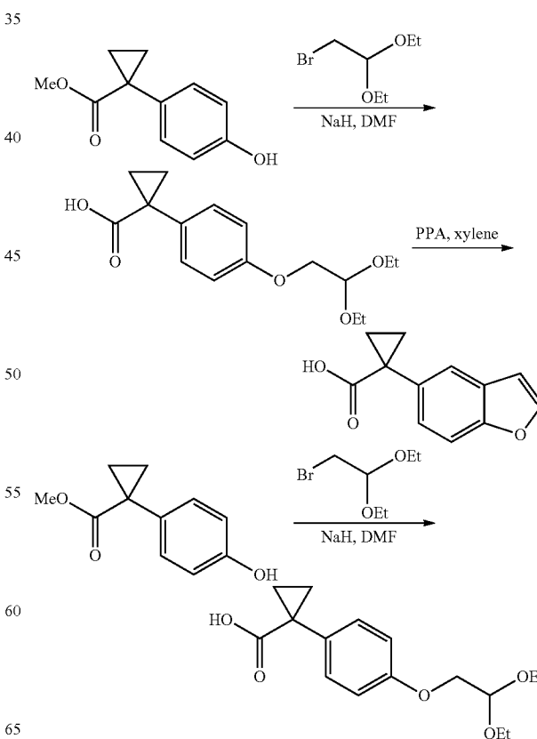
1-(Benzofuran-5-yl)cyclopropanecarboxylic acid
