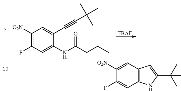
2-tert-Butyl-6-fluoro-5-nitro-1H-indole
