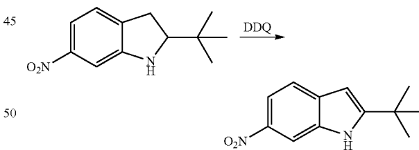
2-tert-Butyl-6-nitro-1H-indole
