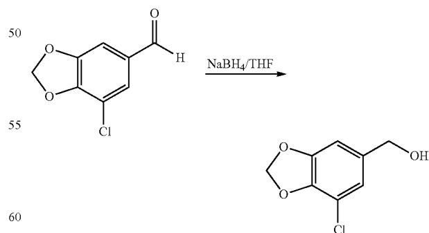
(7-Chlorobenzo[d][1,3]dioxol-5-yl)methanol
