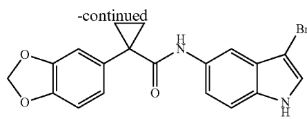
1-(Benzo[d][1,3]dioxol-5-yl)-N-(3-bromo-1H-indol-5-yl)cyclopropanecarboxamide
