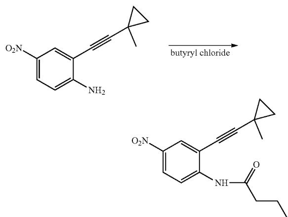
N-[2-(1-Methyl-cyclopropylethynyl)-4-nitro-phenyl]-butyramide
