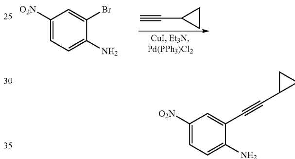
2-(Cyclopropylethynyl)-4-nitroaniline
