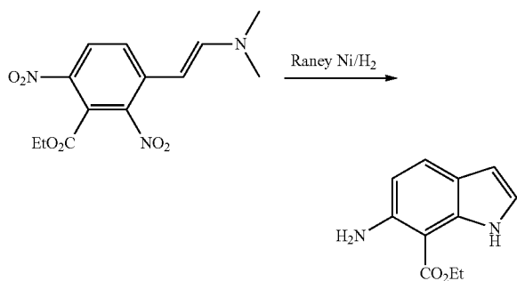
Ethyl 6-amino-1H-indole-7-carboxylate
