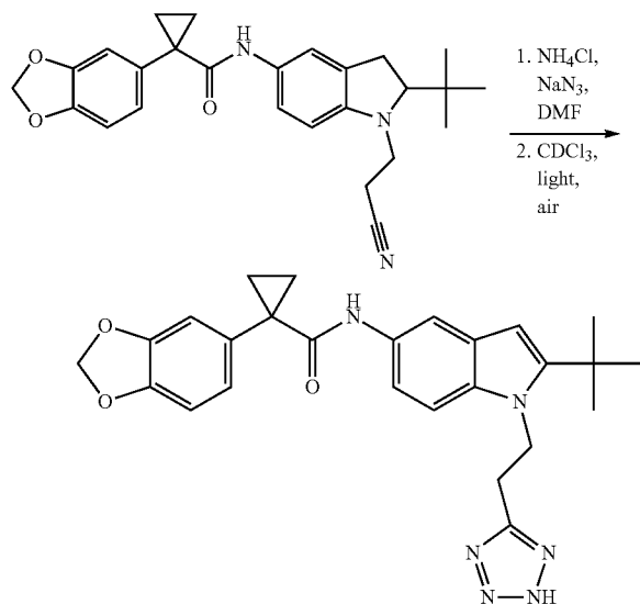
N-(1-(2-(2H-Tetrazol-5-yl)ethyl)-2-tert-butyl-1H-indol-5-yl)-1-(benzo[d][1,3]dioxol-5-yl)cyclopropanecarboxamide
