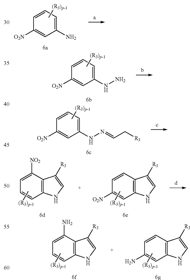
Scheme 6
