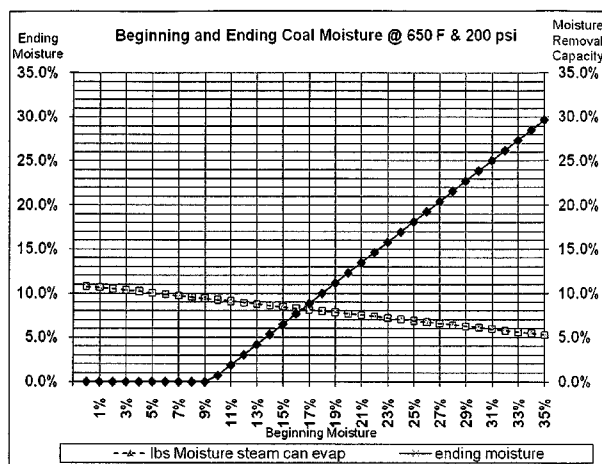
Evaporation of Moisture from Coal by Mill with 650 °F, 200 psi Steam Source
