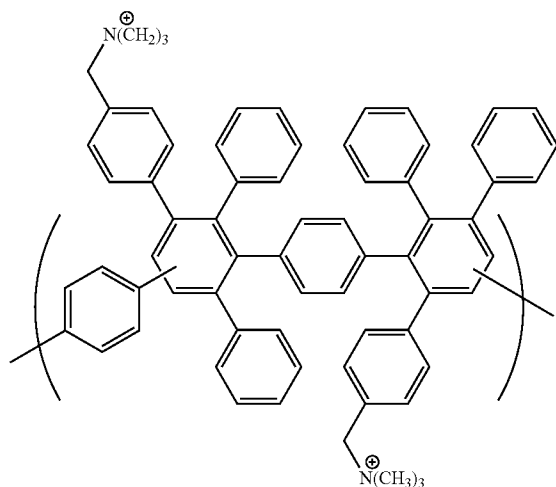
Tetraalkylammonium functionalized poly(phenylene)
