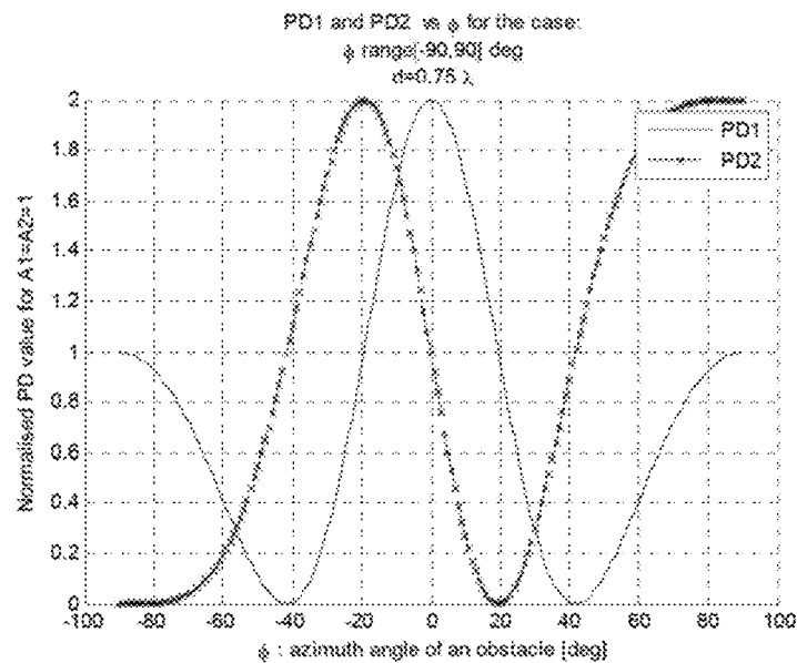
b) Apparatus 101, 102b angle detection up to \pm 40 degrees
