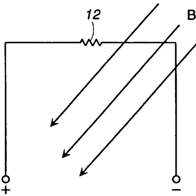
FIG. 4 (PRIOR ART)
