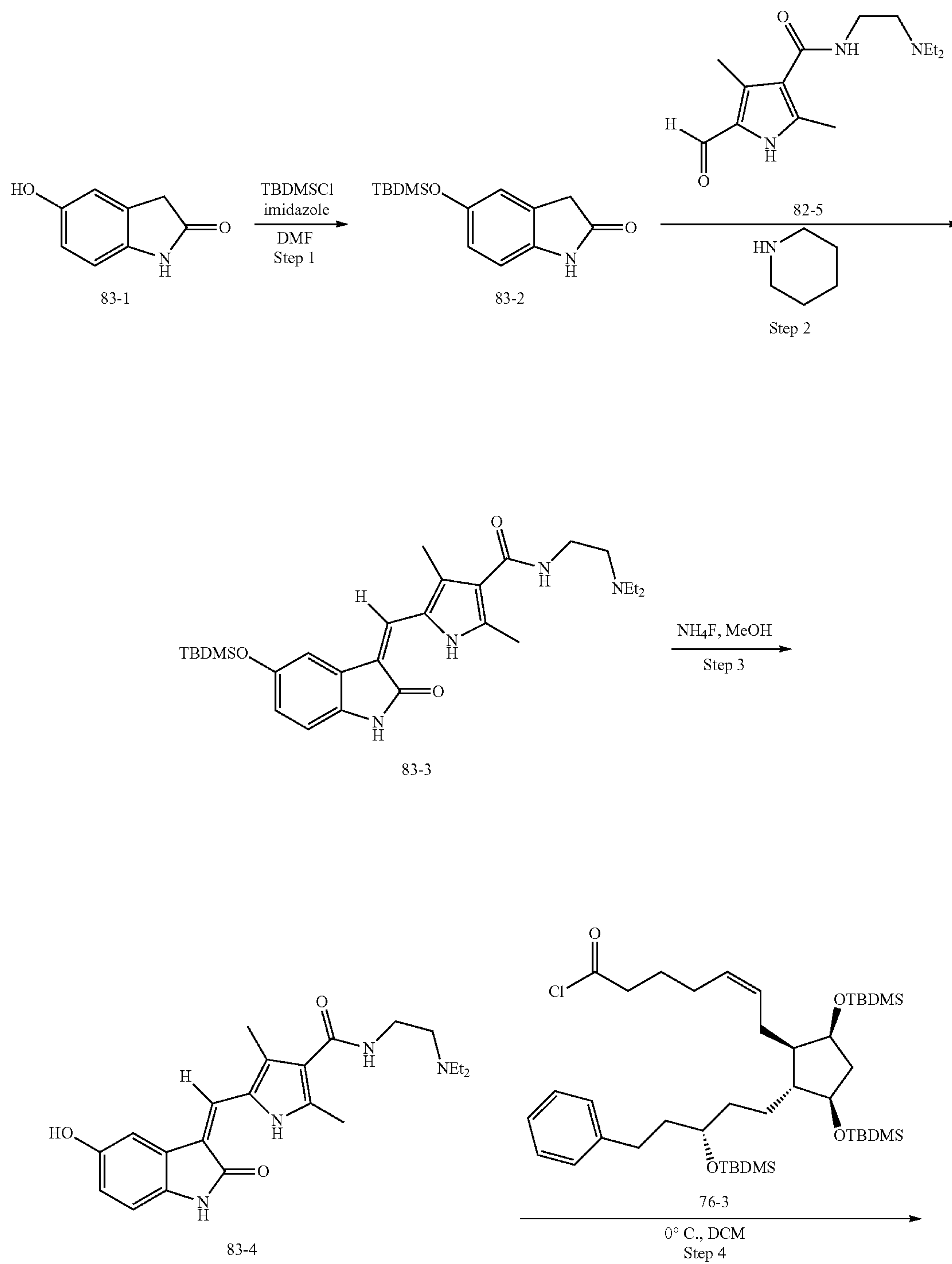
Scheme 83:
