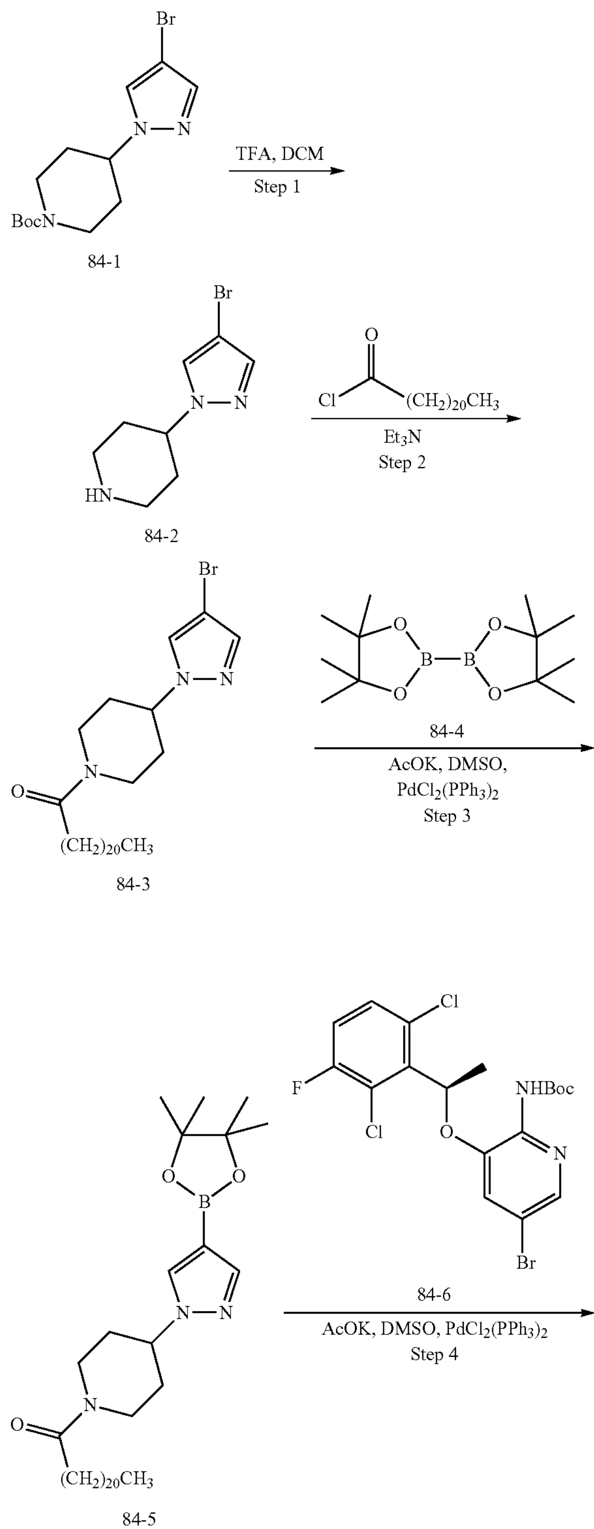
Scheme 84:
