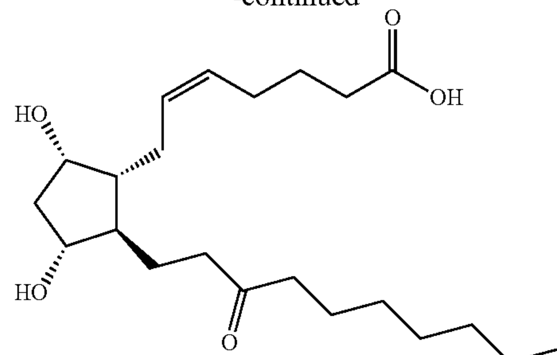
Unoprostone
