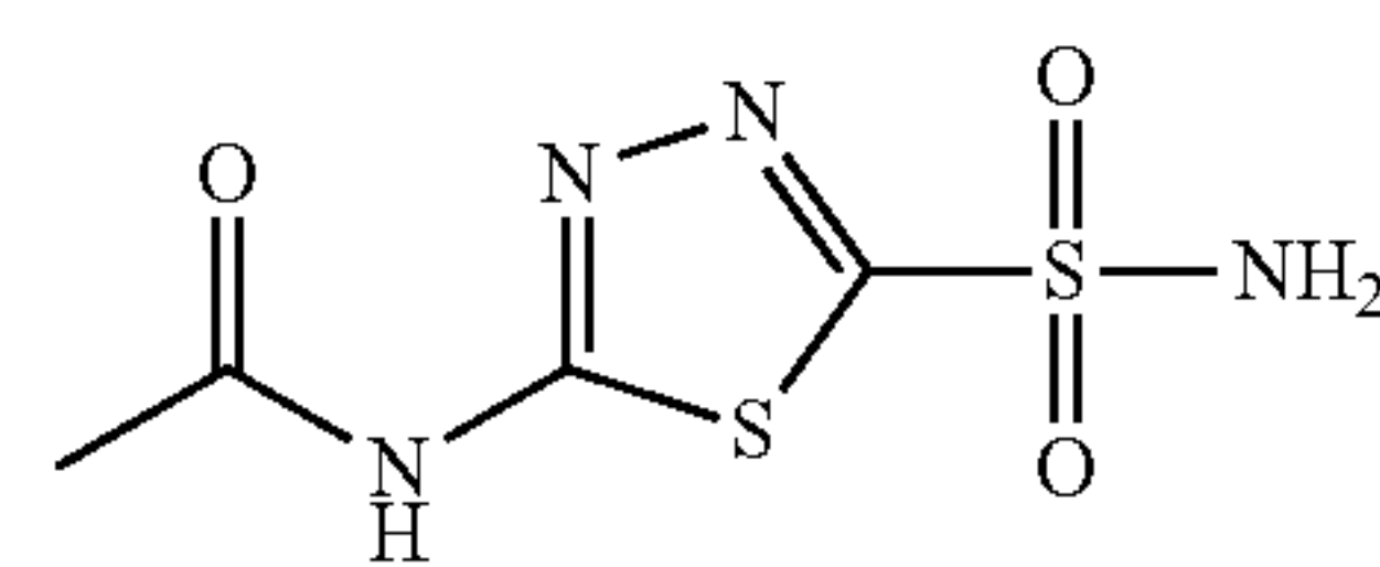
Methazolamide
