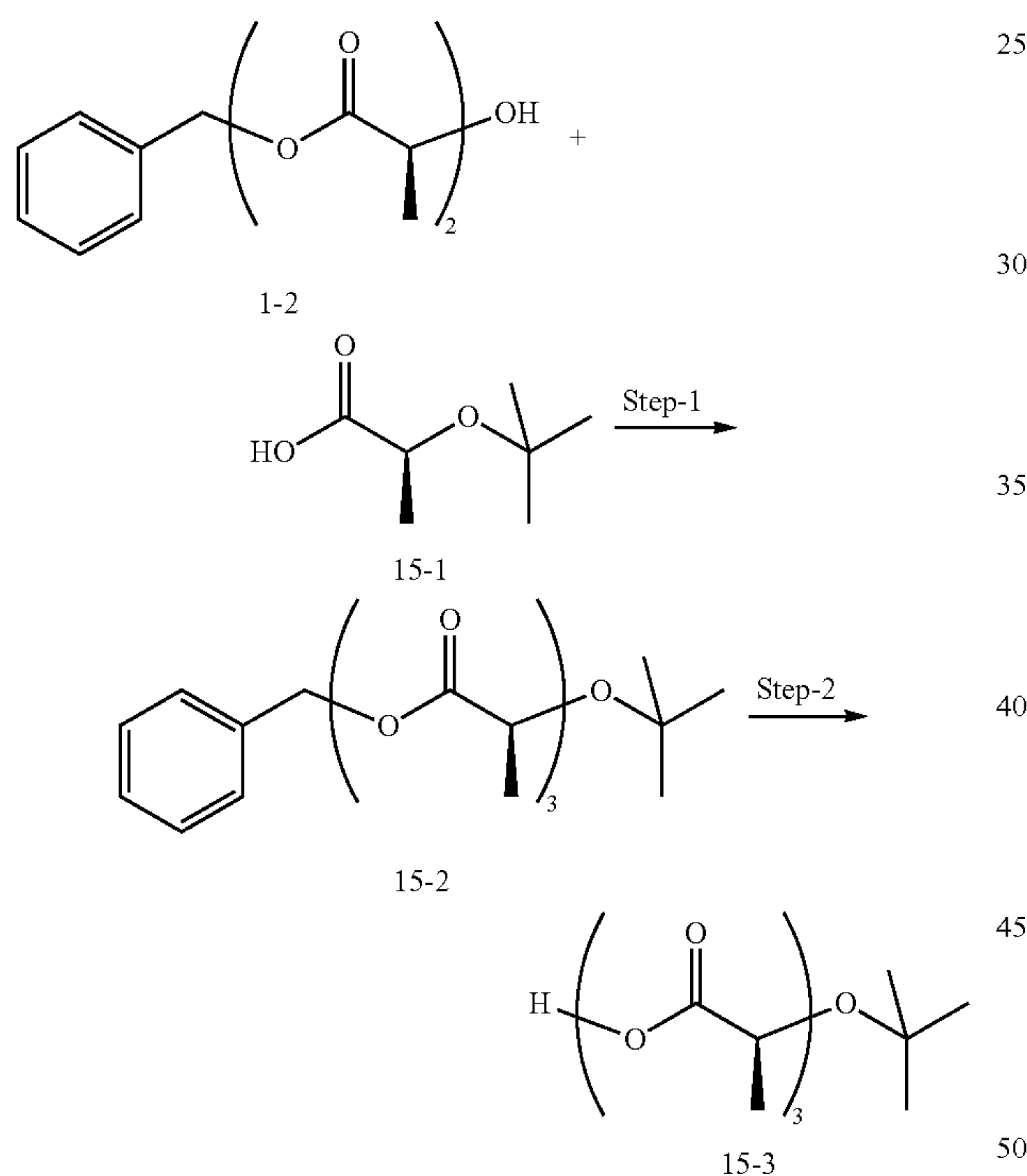
Scheme 15: (S)-2-tert-Butoxy-propionic acid (S)-1-((S)-1-carboxy-ethoxycarbonyl)-ethyl ester (15-3):
