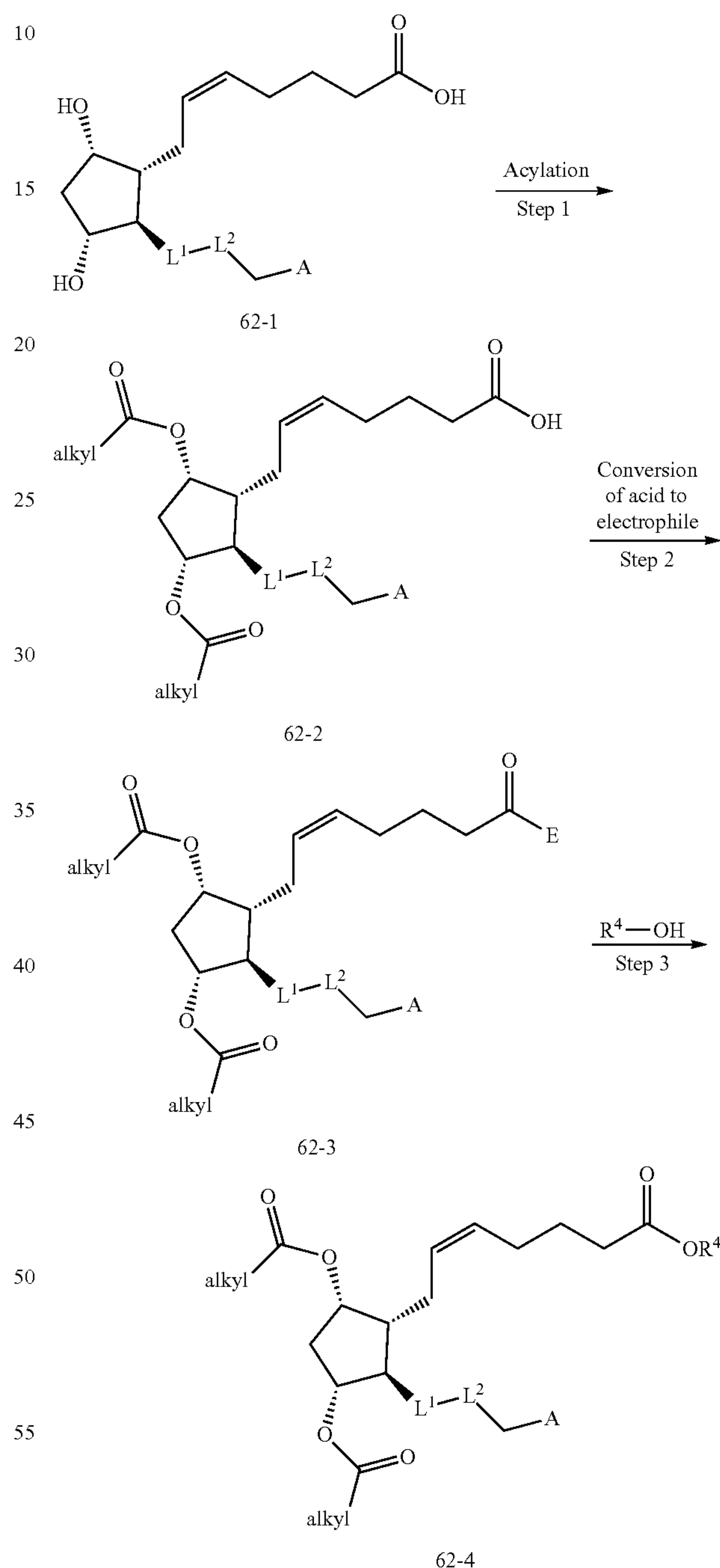
Scheme 62:
