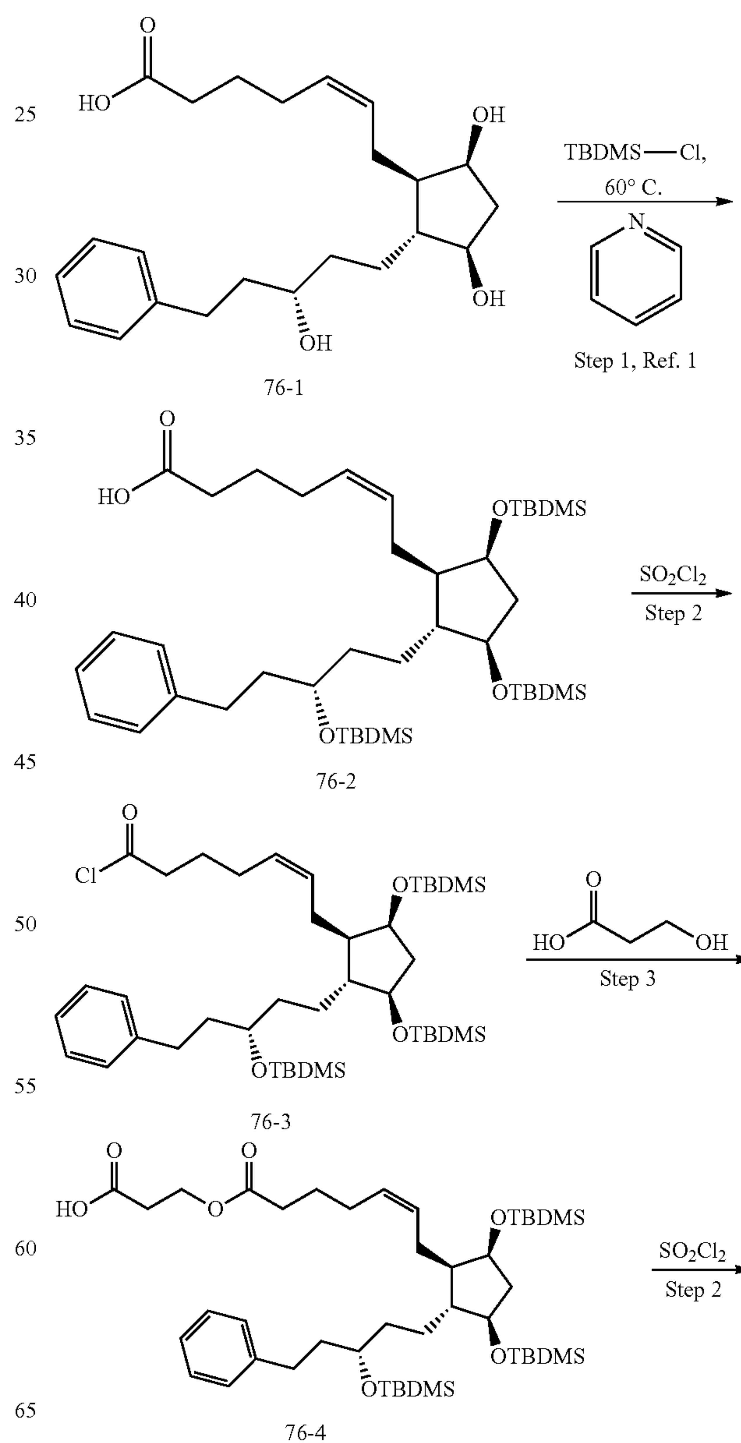
Scheme 76:
