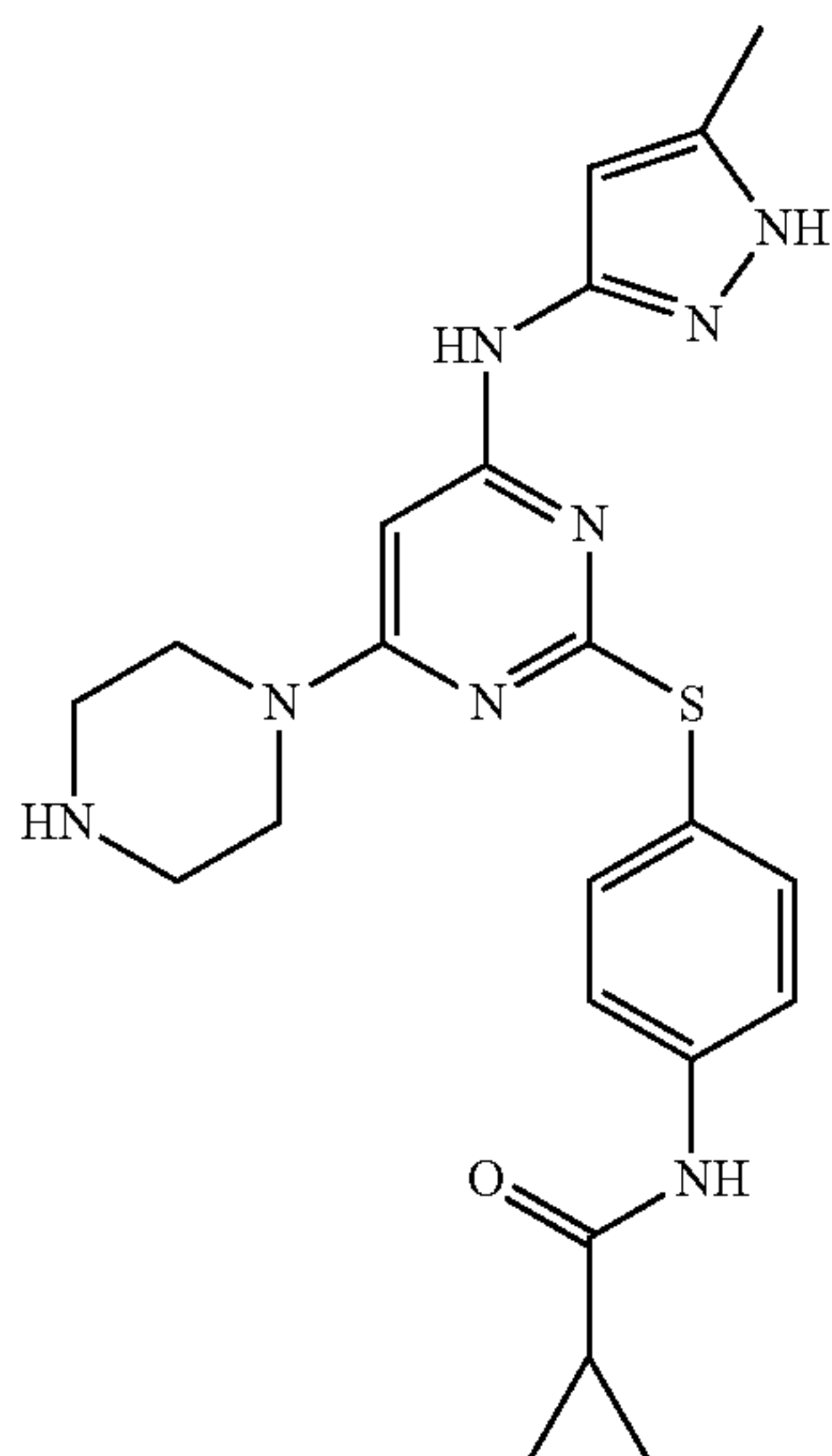
Tozasertib derivative
