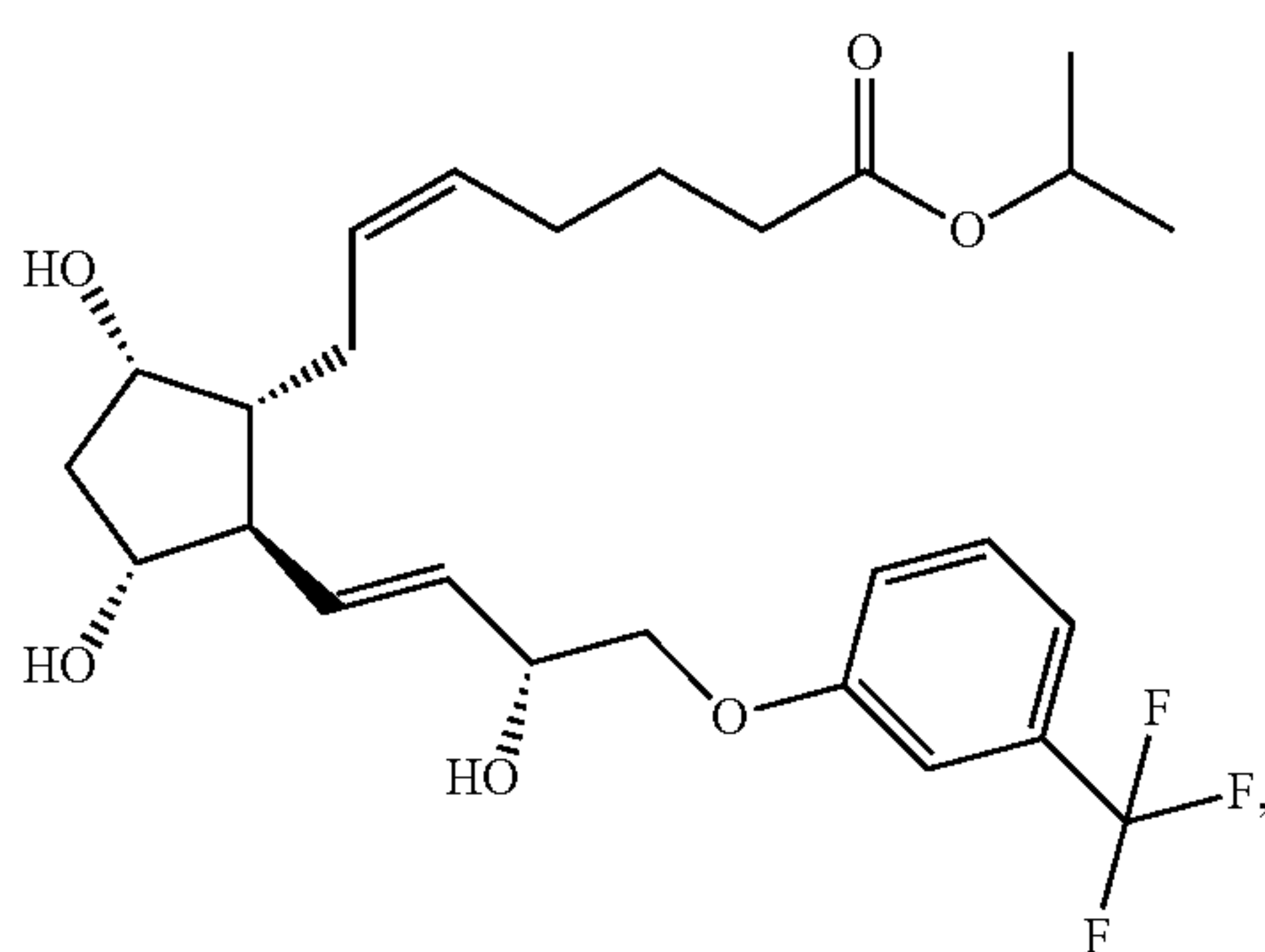
Travoprost
