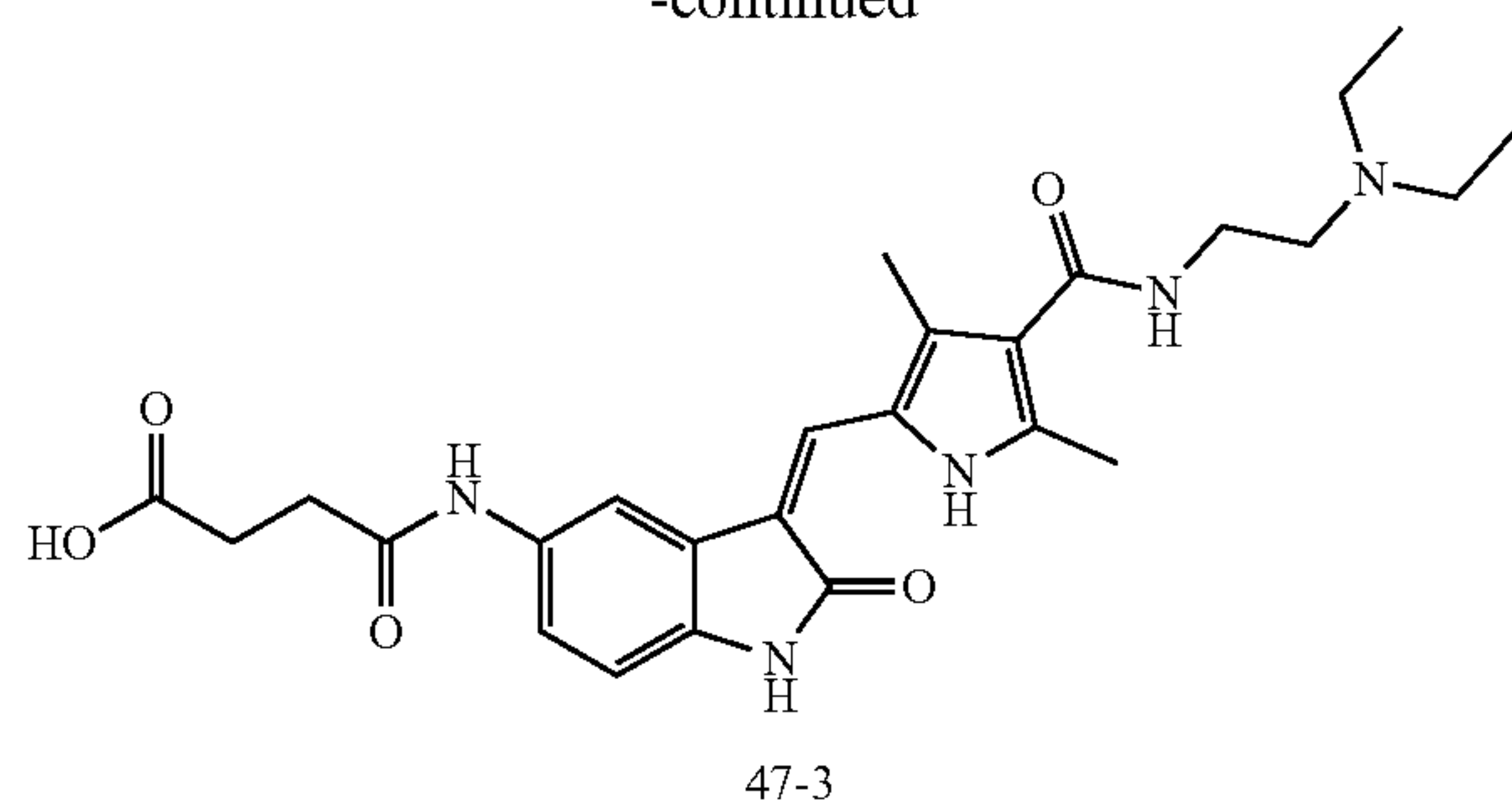
Scheme 49: (3Z)-3-[(4-{[2-(Diethylamino)ethyl]carbamoyl}-3,5-dimethyl-1H-pyrrol-2-yl)methylidene]-2-oxo-2,3-dihydro-1H-indol-5-yl (2S)-2-[(2S)-2-(acetyloxy)propanoyl]oxypropanoate (49-1):
