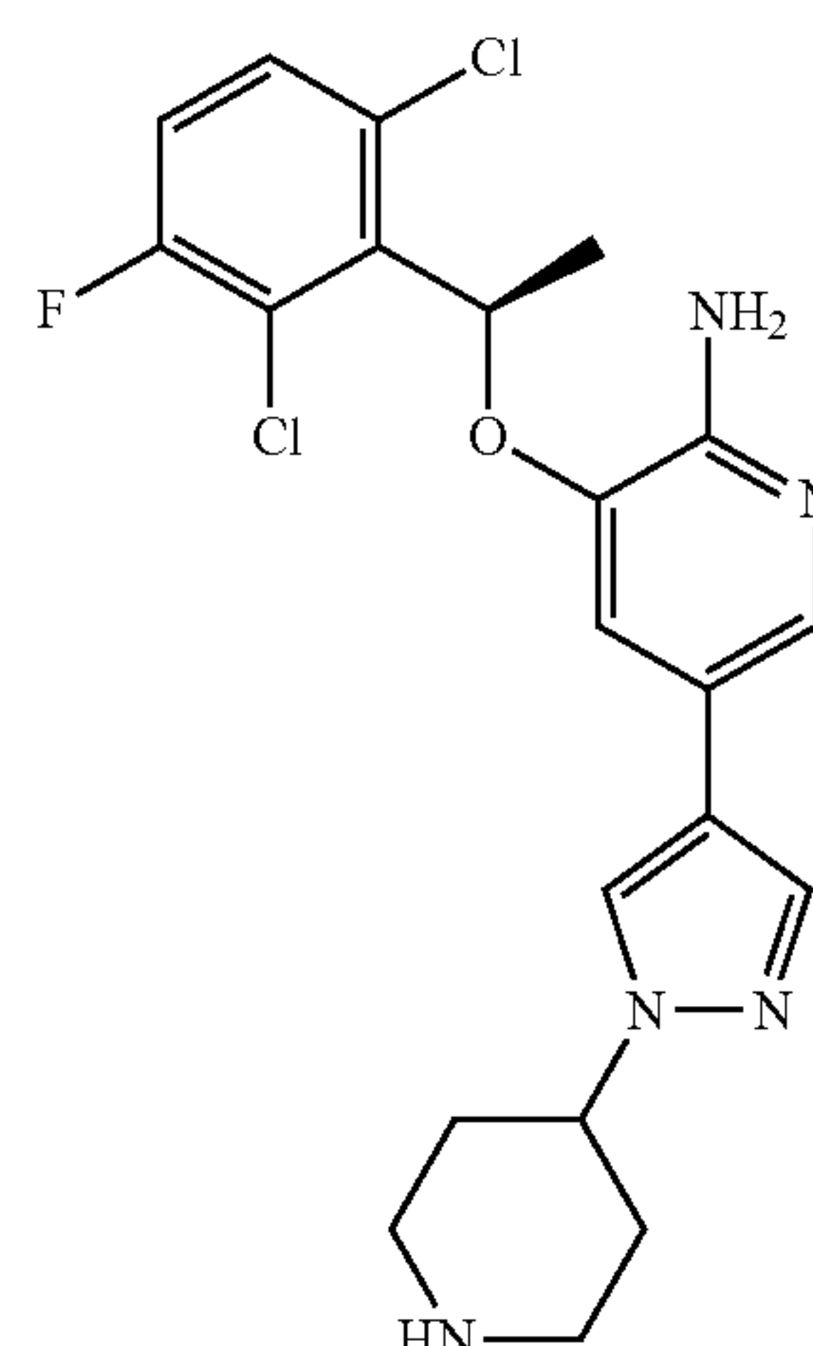
Crizotinib
