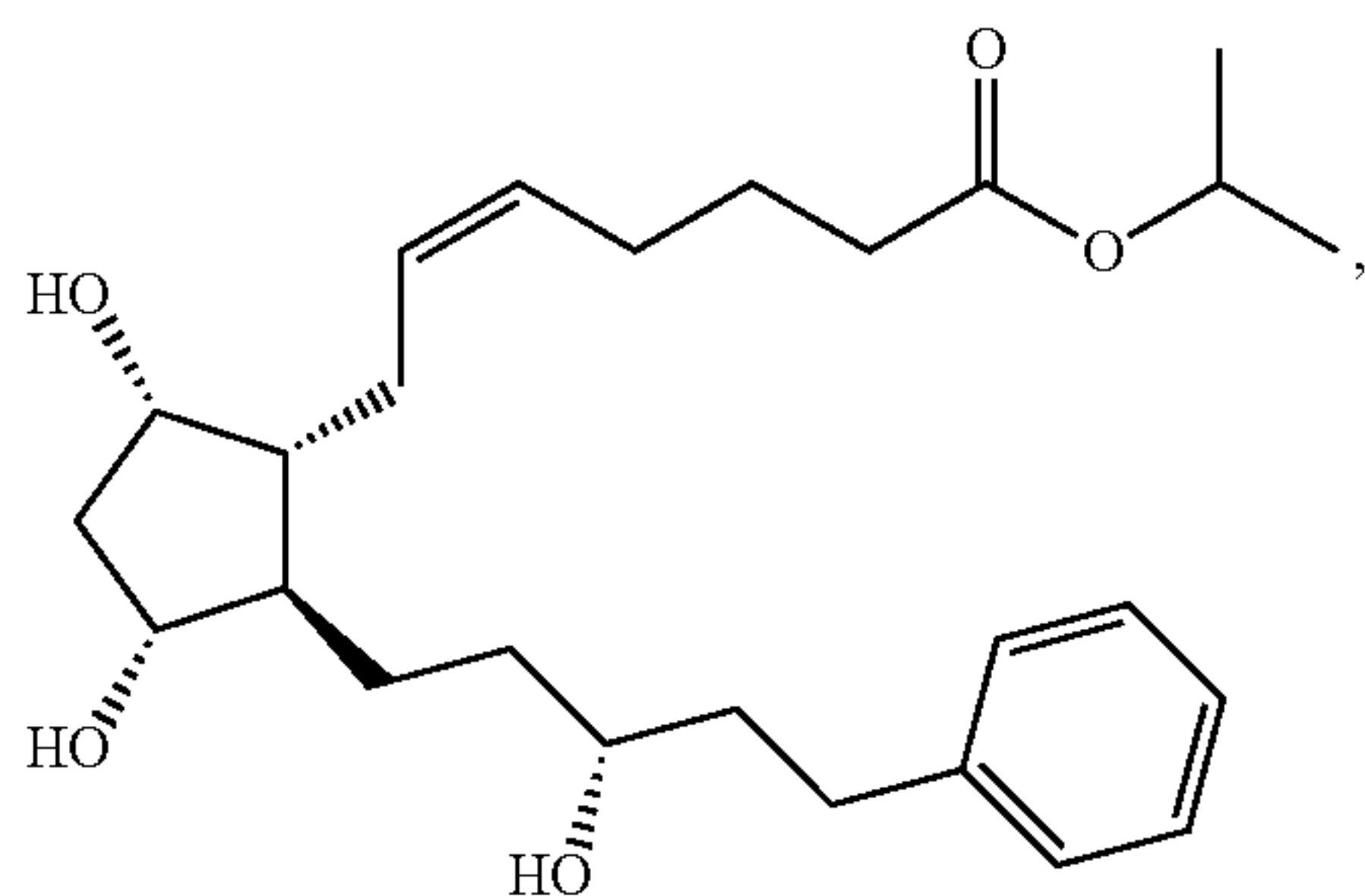
Latanoprost
