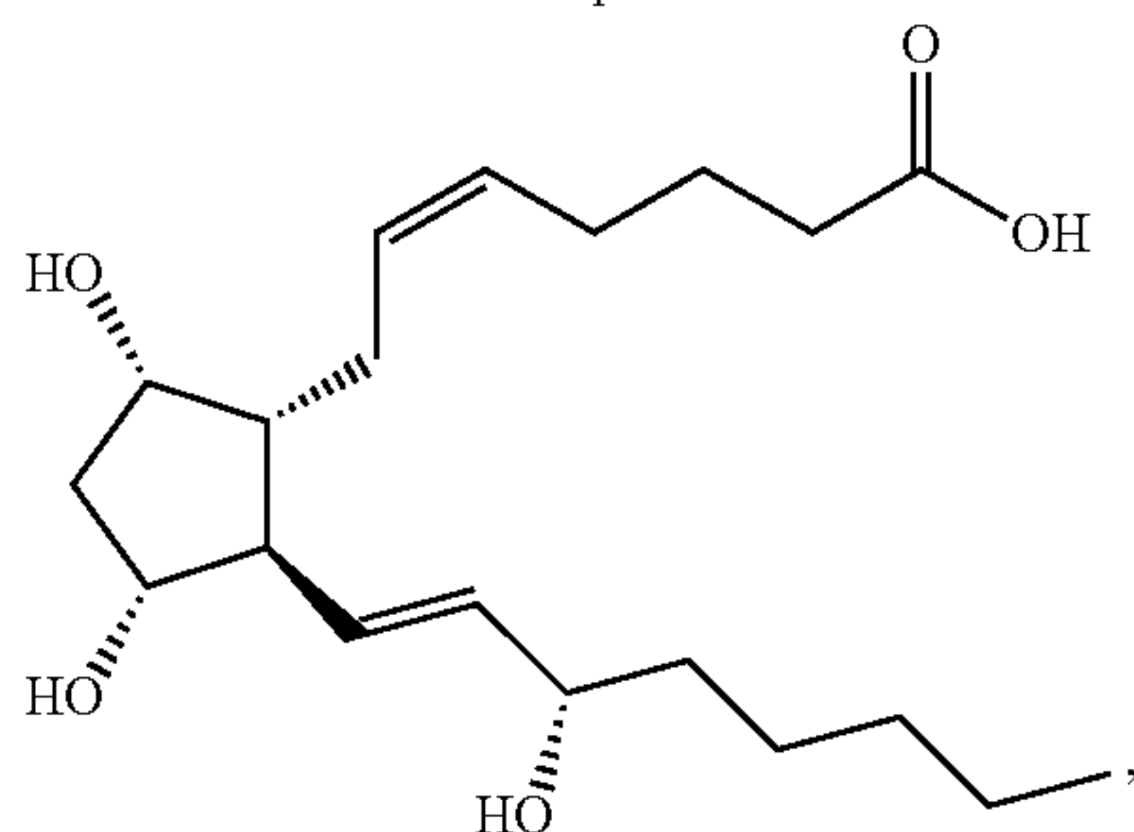
Dinoprost
