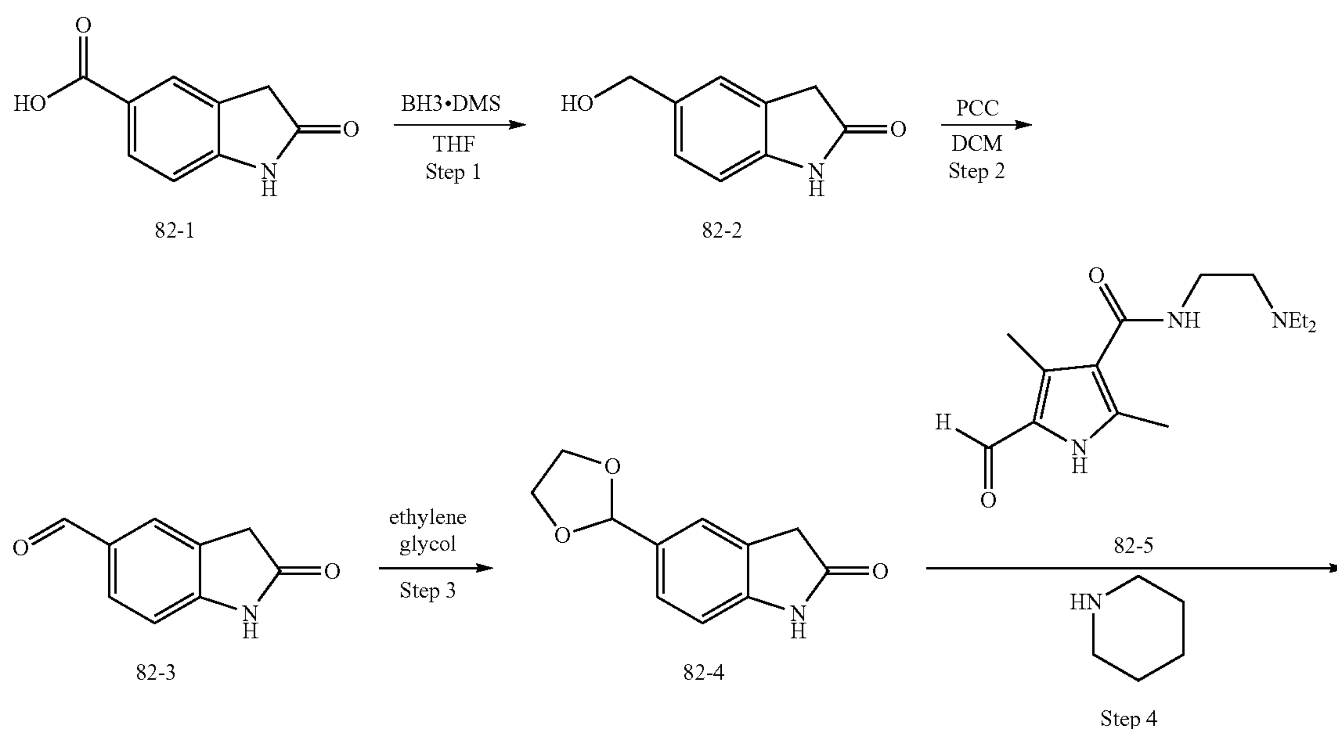
Scheme 82:
