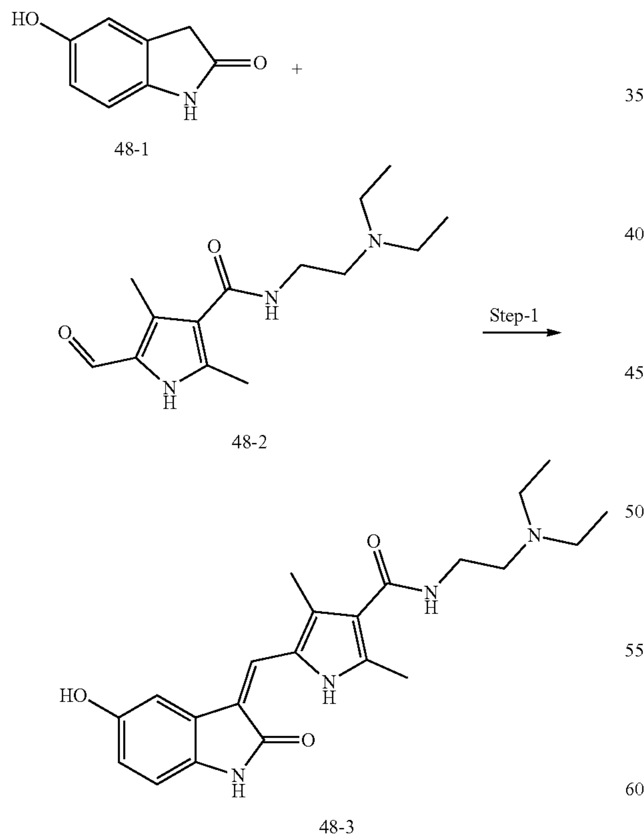
Scheme 48: 5-Hydroxy Sunitinib (48-3):
