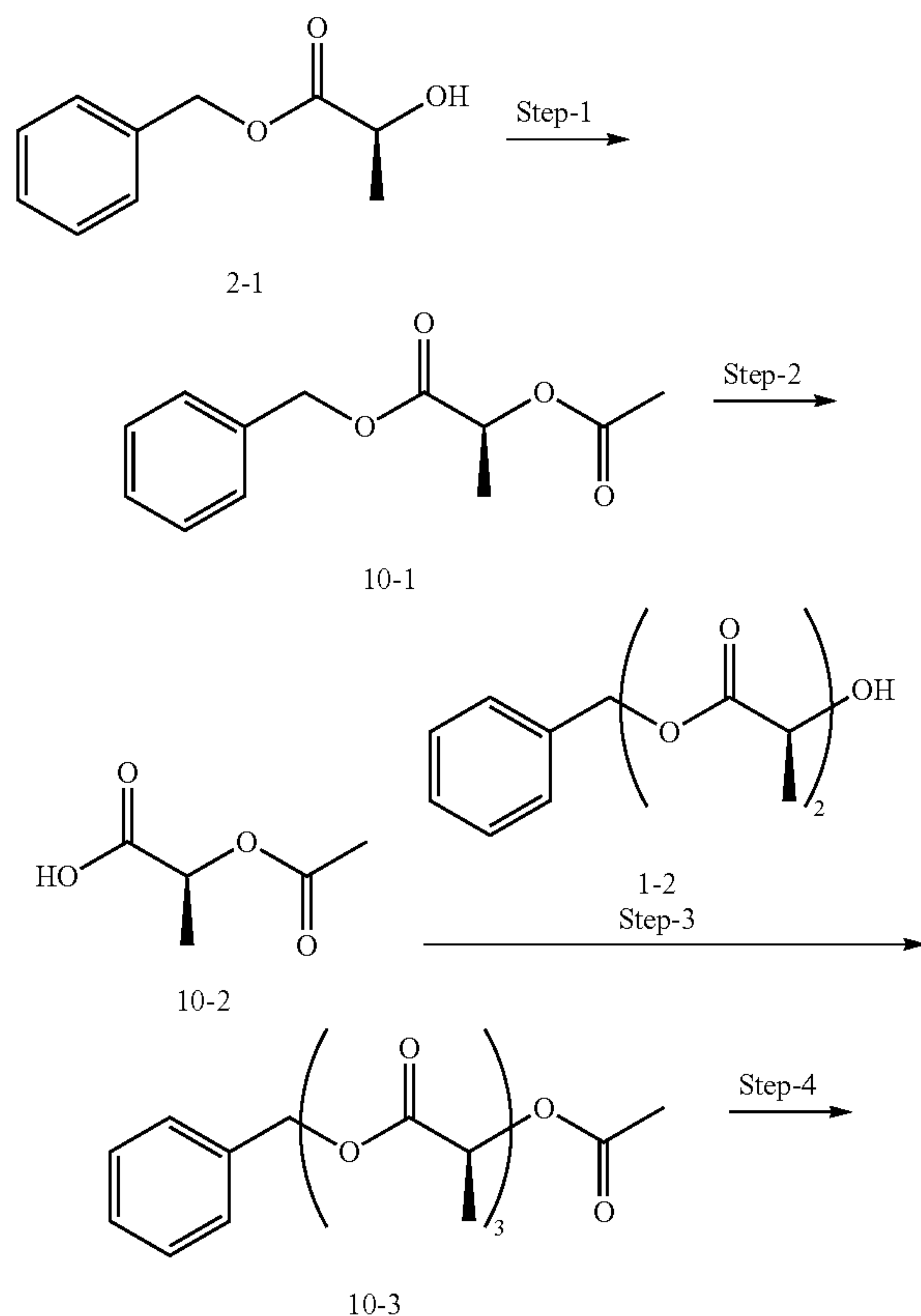
Scheme 10: (S)-2-[(S)-2-((S)-2-Acetoxy-propionyloxy)-propionyloxy]-propionic acid (10-4):
