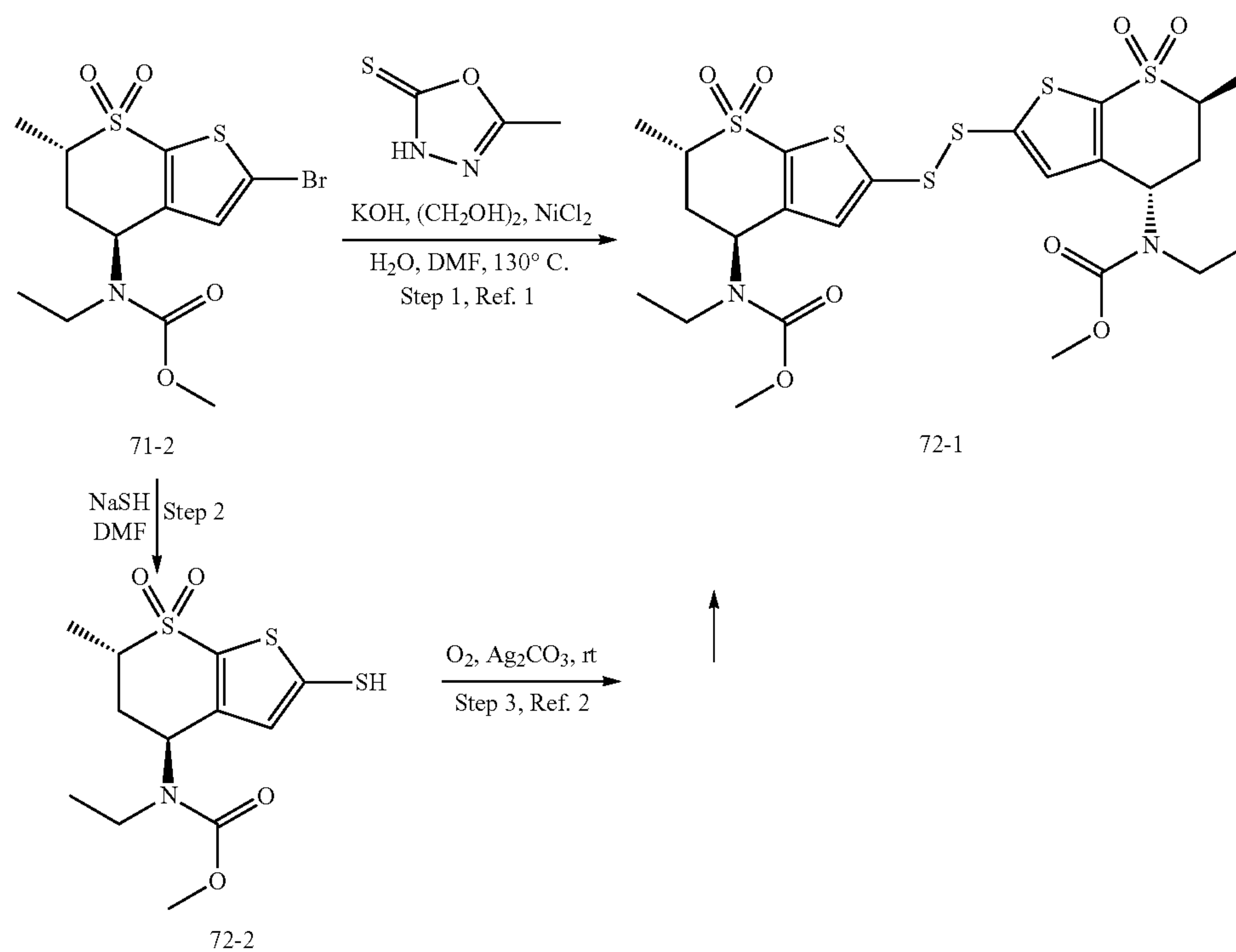
Scheme 72:
