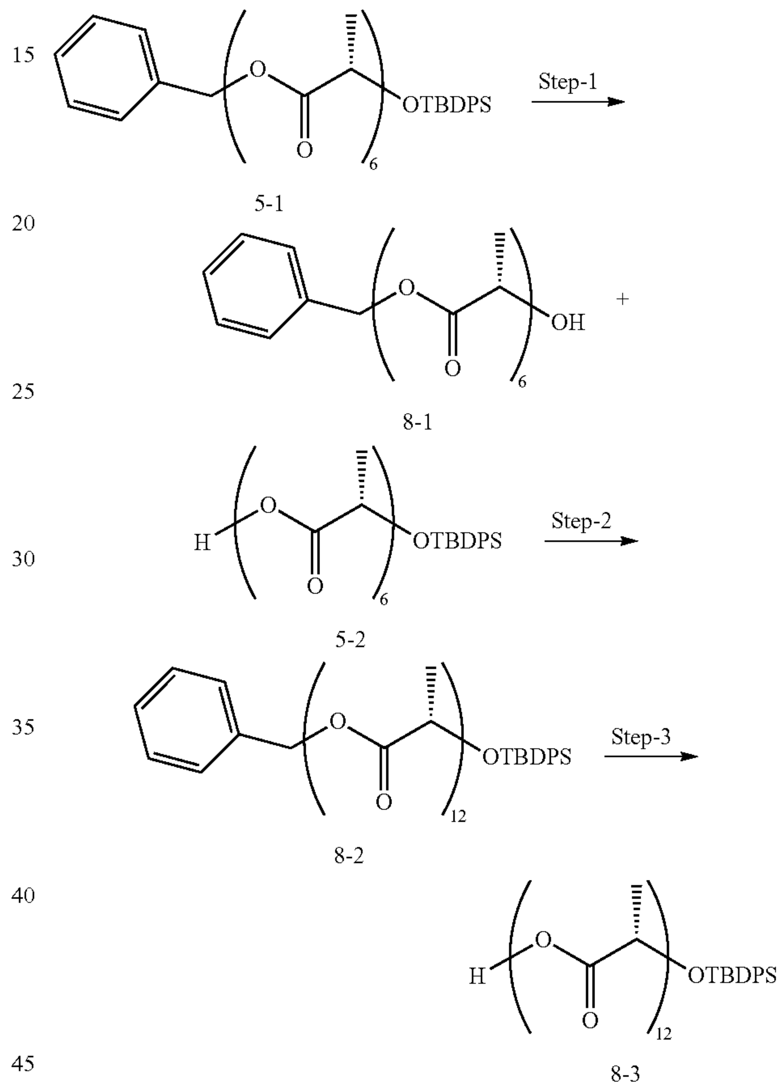
Scheme 8: Compound 8-3 (PLA (n=12)-O-TBDPS):
