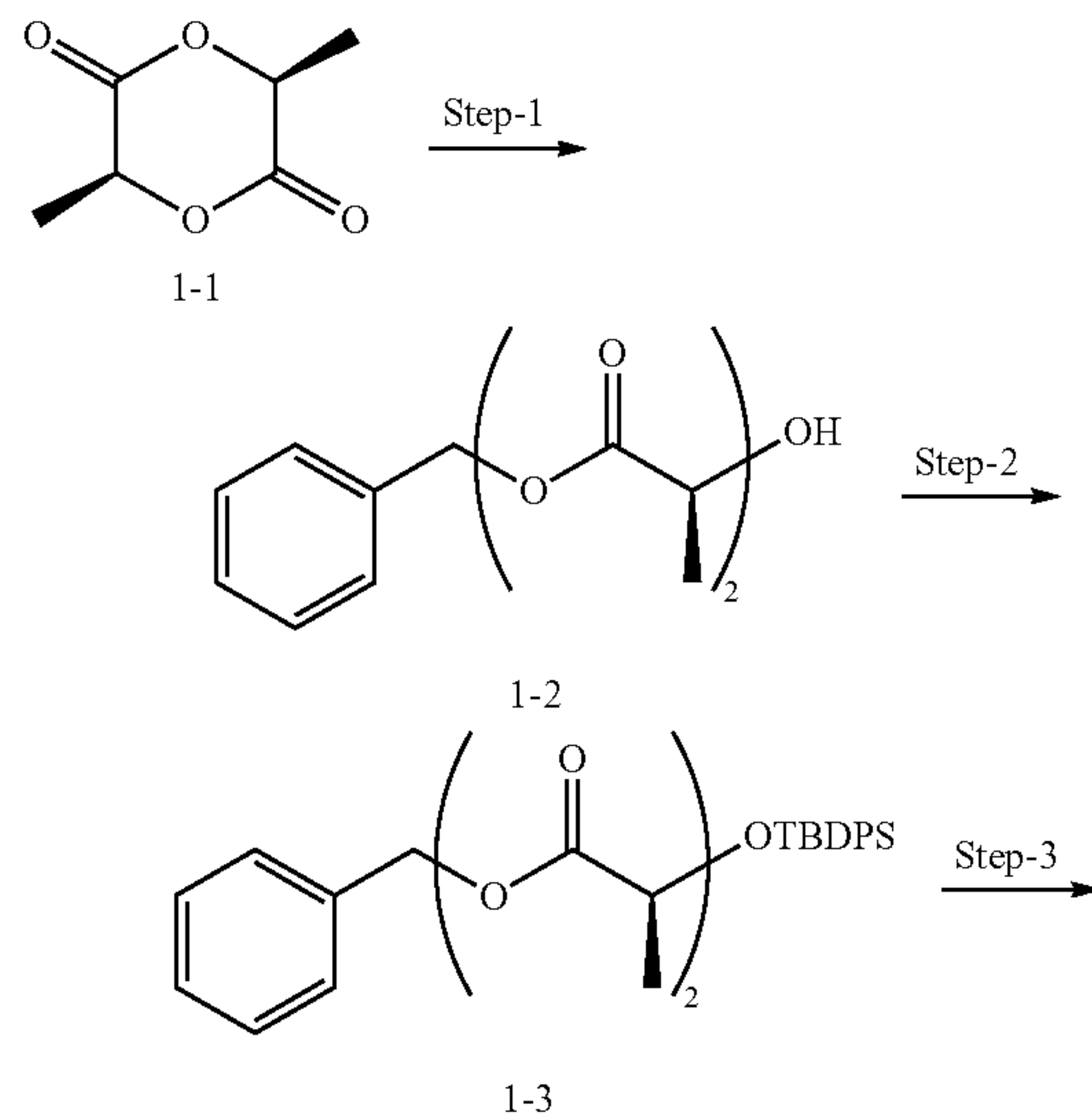
Scheme 1: (S)-2-(tert-Butyl-diphenyl-silanyloxy)-propionic acid (S)-1-carboxy-ethyl ester (1-4):
