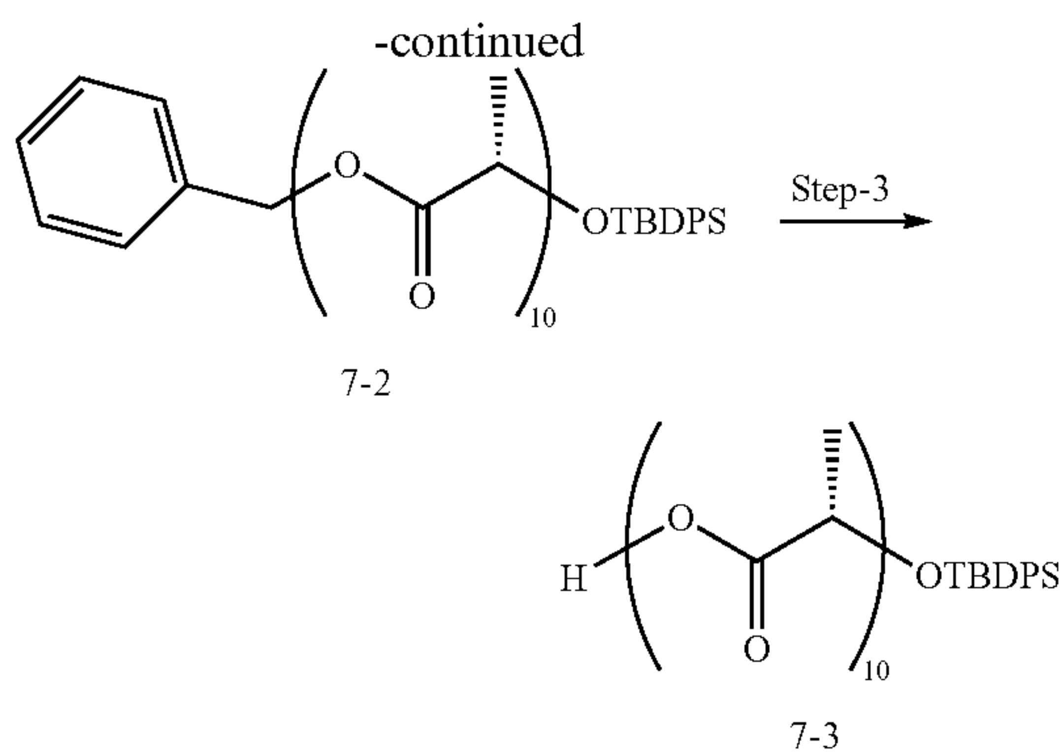
Scheme 8: Compound 8-3 (PLA (n=12)-O-TBDPS):
