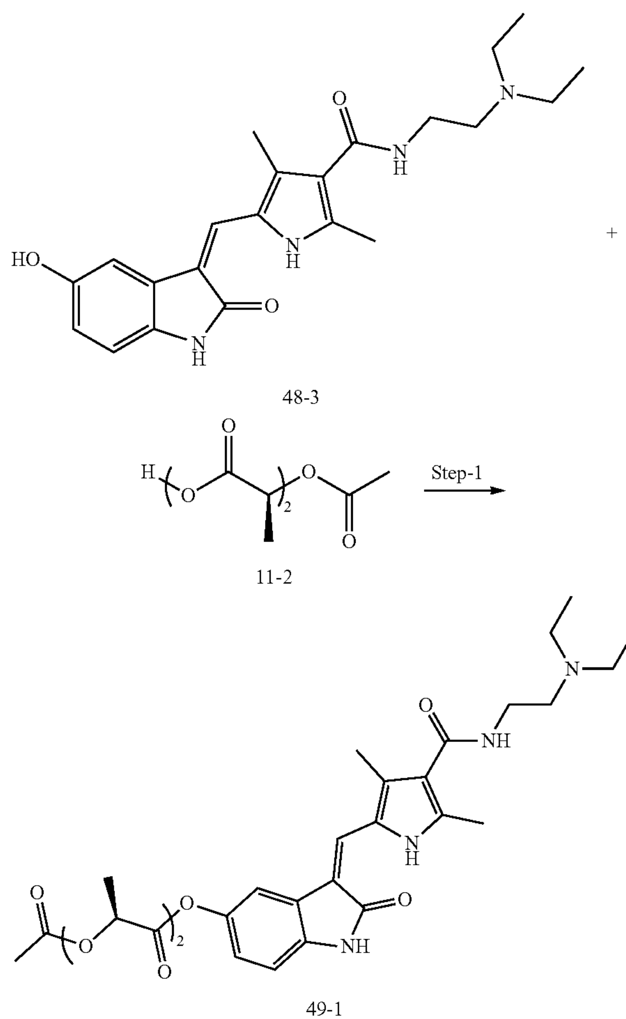
Scheme 49: (3Z)-3-[(4-{[2-(Diethylamino)ethyl]carbamoyl}-3,5-dimethyl-1H-pyrrol-2-yl)methylidene]-2-oxo-2,3-dihydro-1H-indol-5-yl (2S)-2-[(2S)-2-(acetyloxy)propanoyl]oxypropanoate (49-1):
