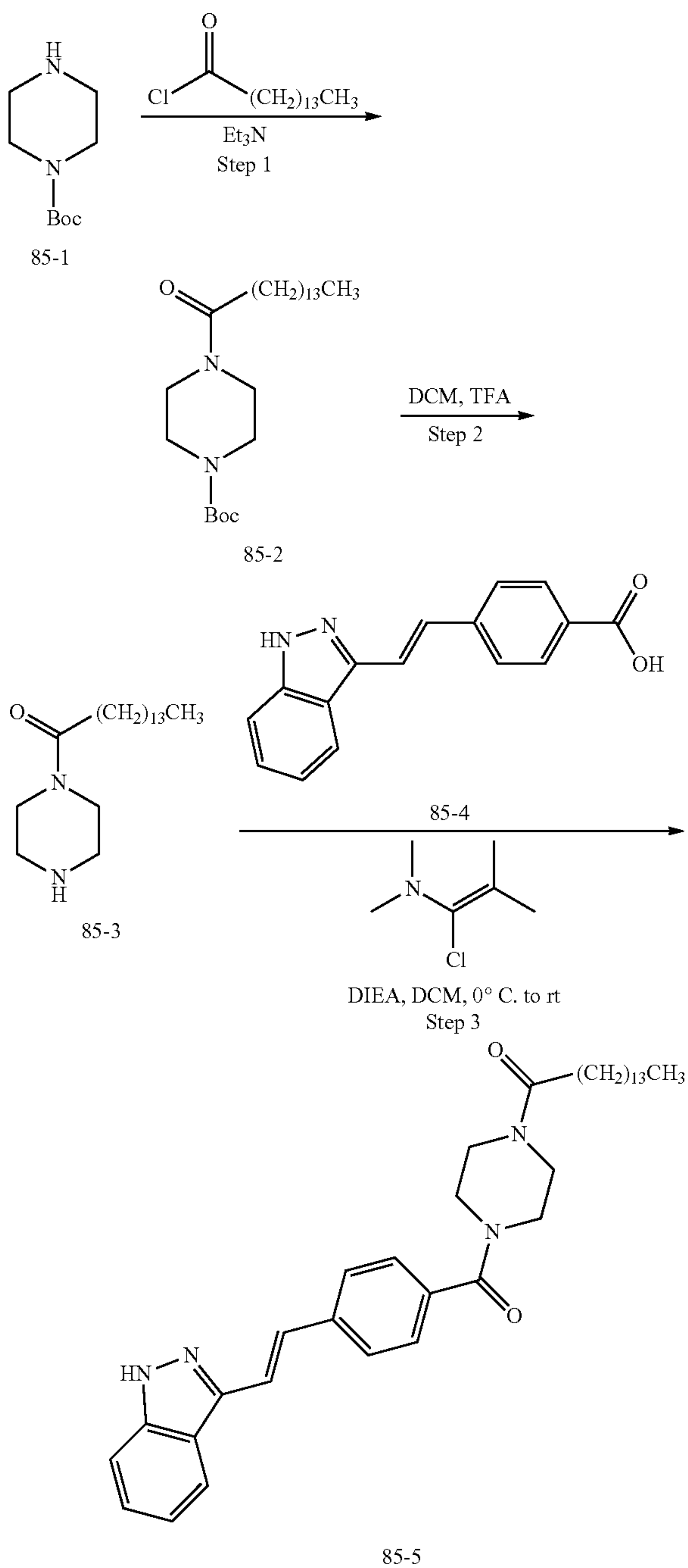
Scheme 85:
