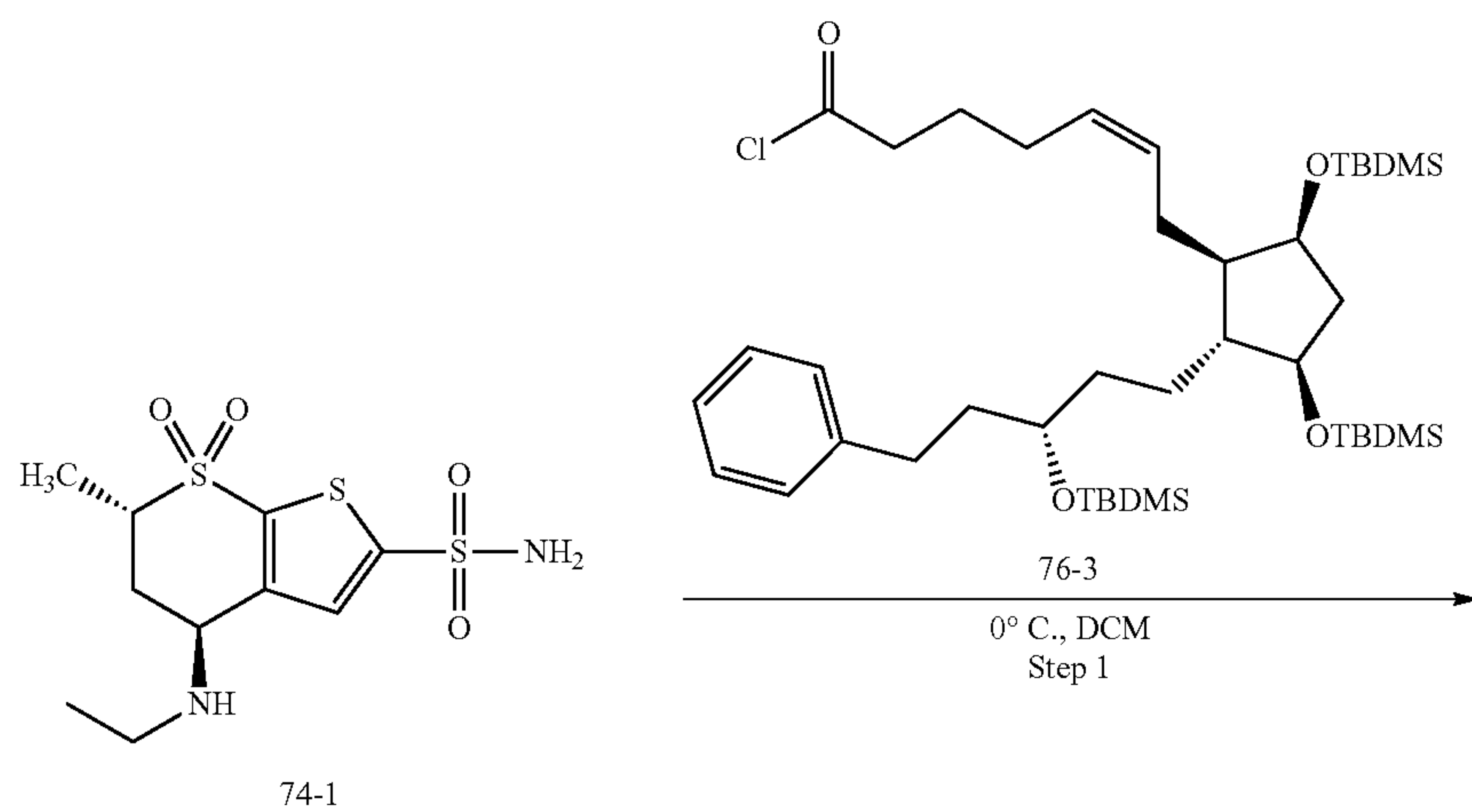
Scheme 80:
