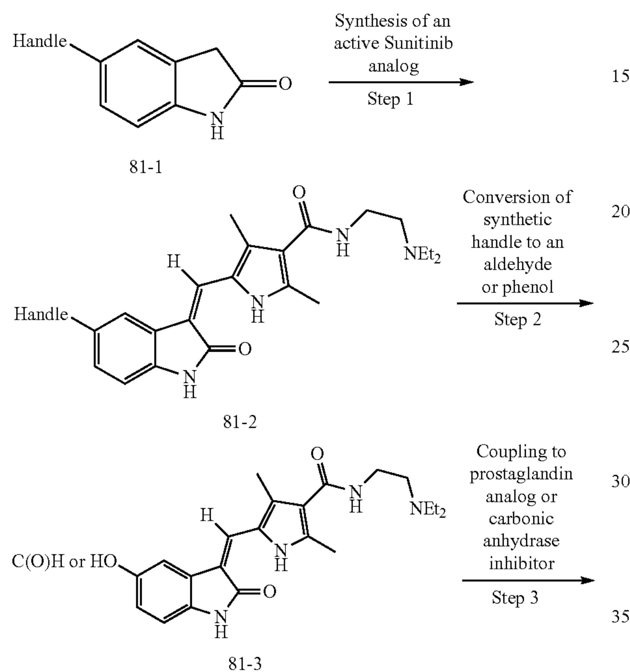
Scheme 81
