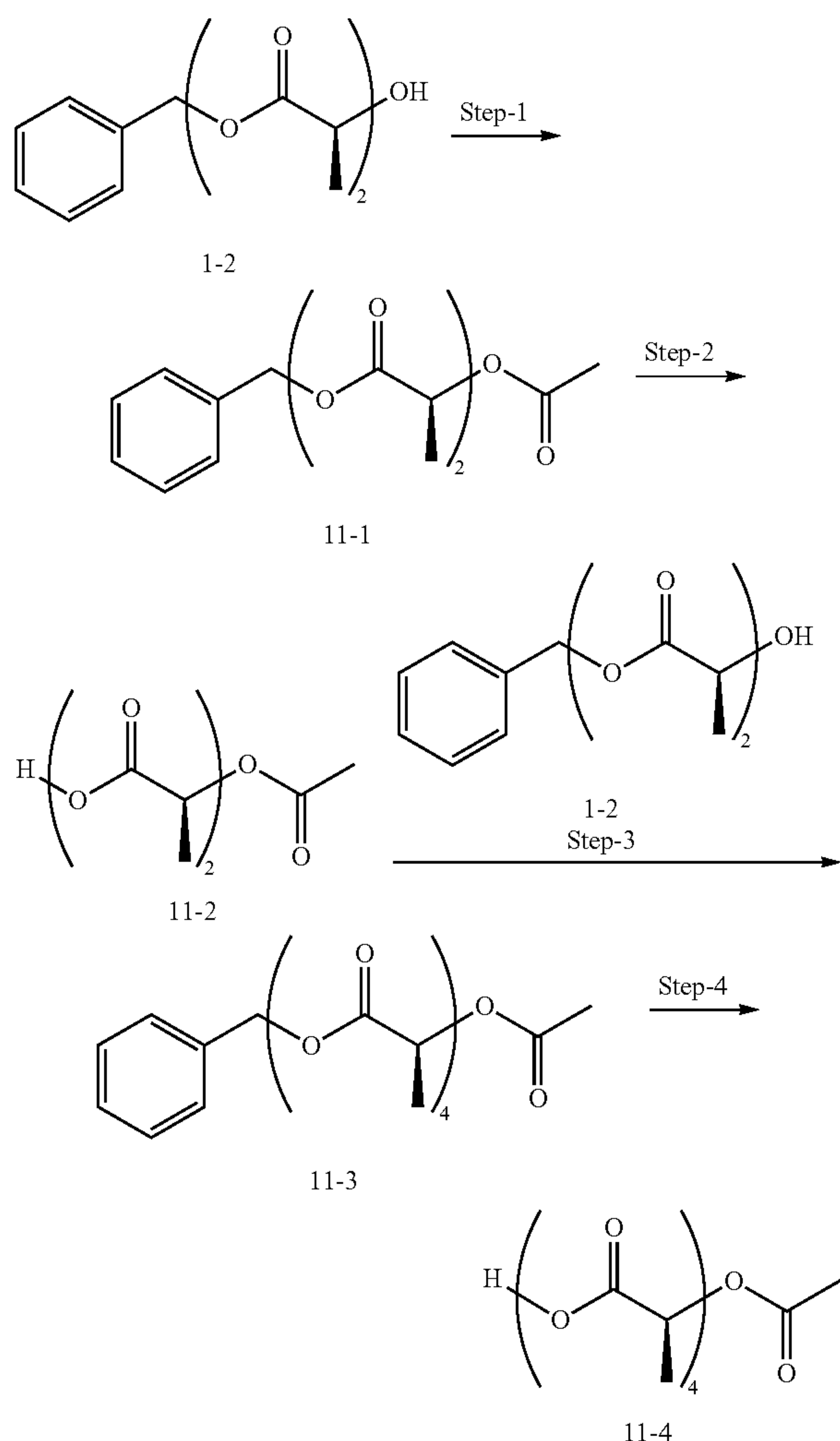
Scheme 11: (S)-2-((S)-2-[(S)-2-((S)-2-Acetoxy-propionyloxy)-propionyloxy]-propionyloxy)-propionic acid (11-4):
