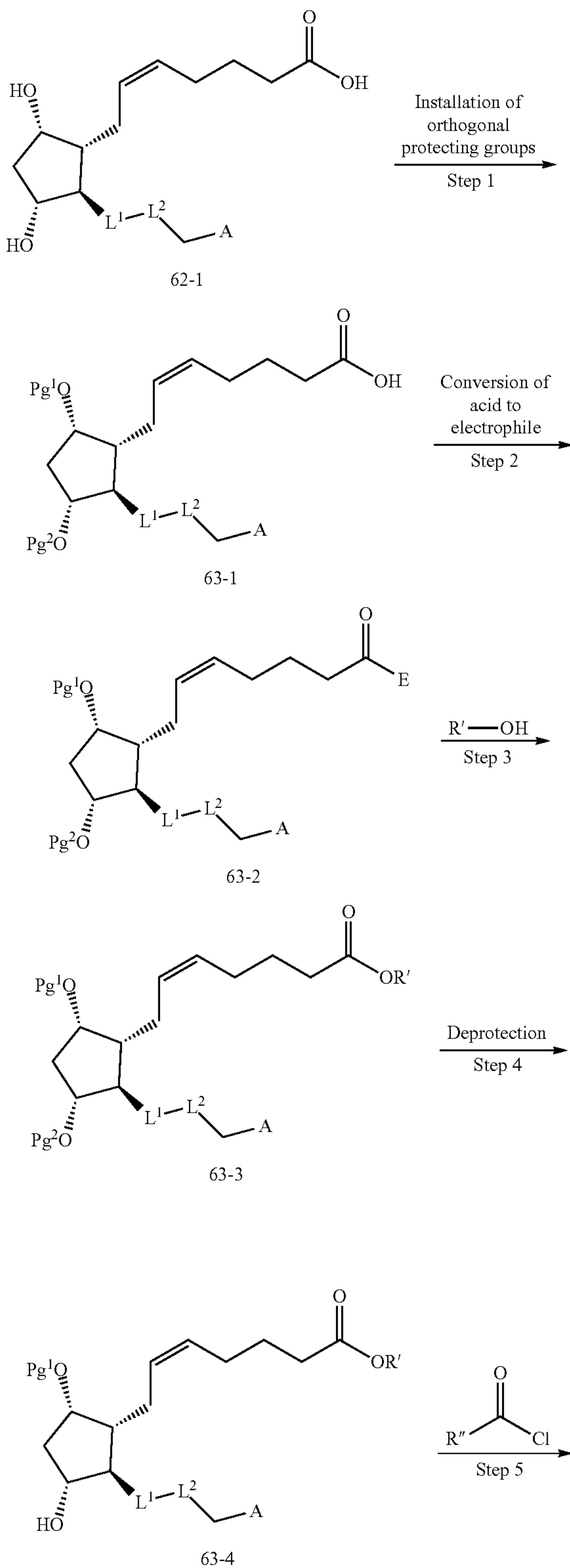
Scheme 63:
