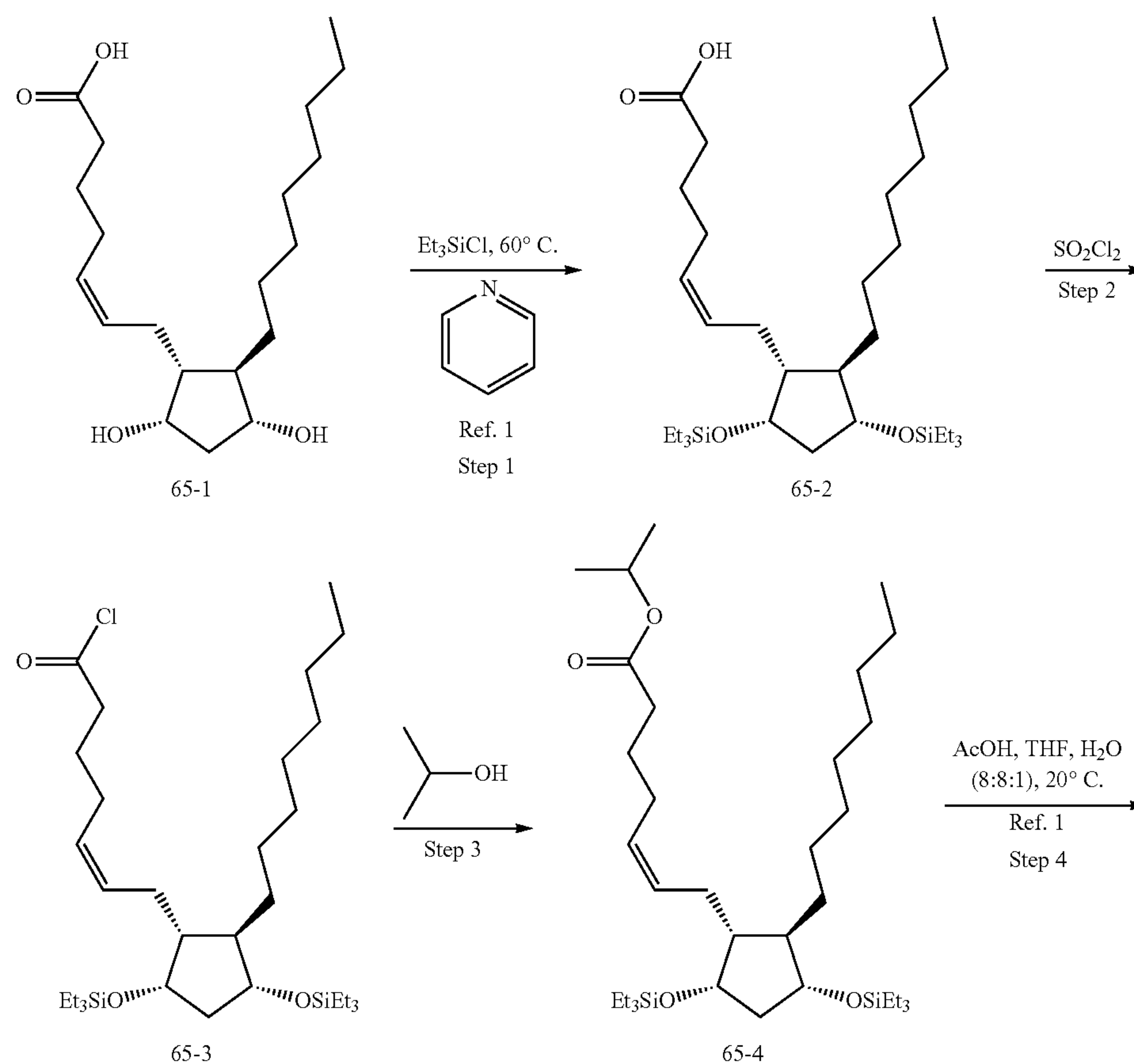
Scheme 65:
