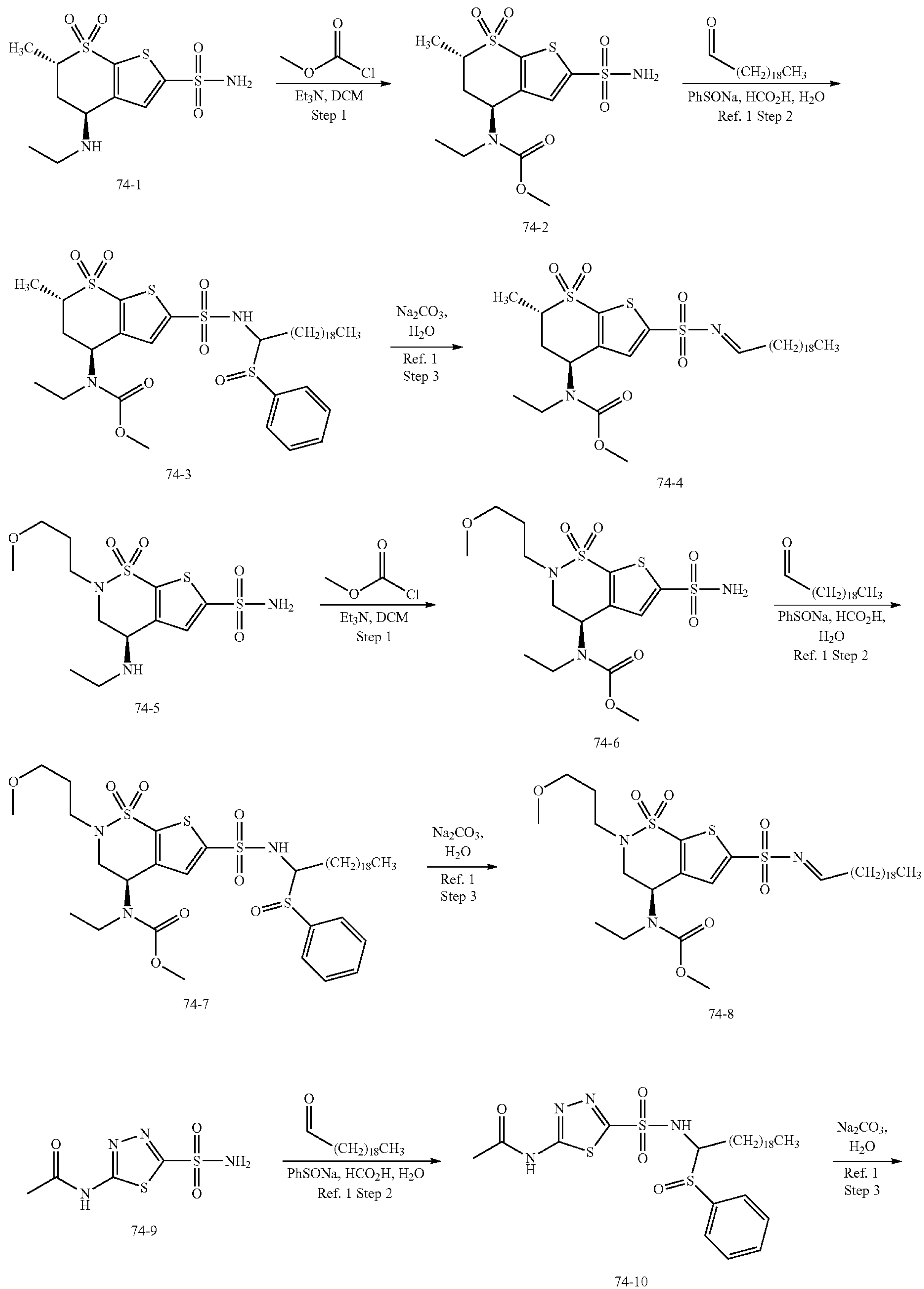
Scheme 74:
