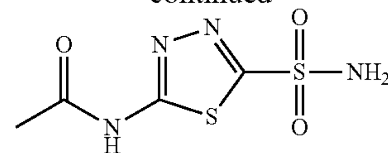
Acetazolamide
