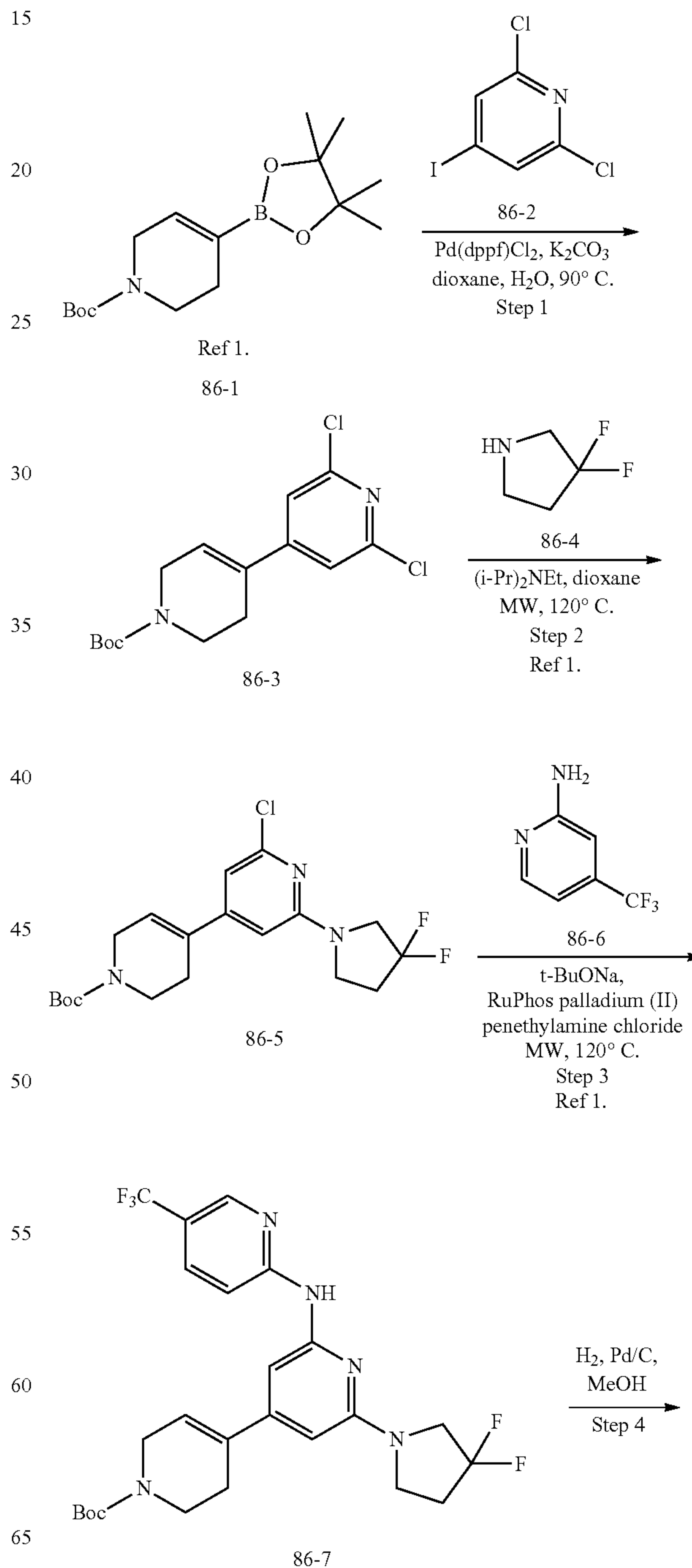
Scheme 86:
