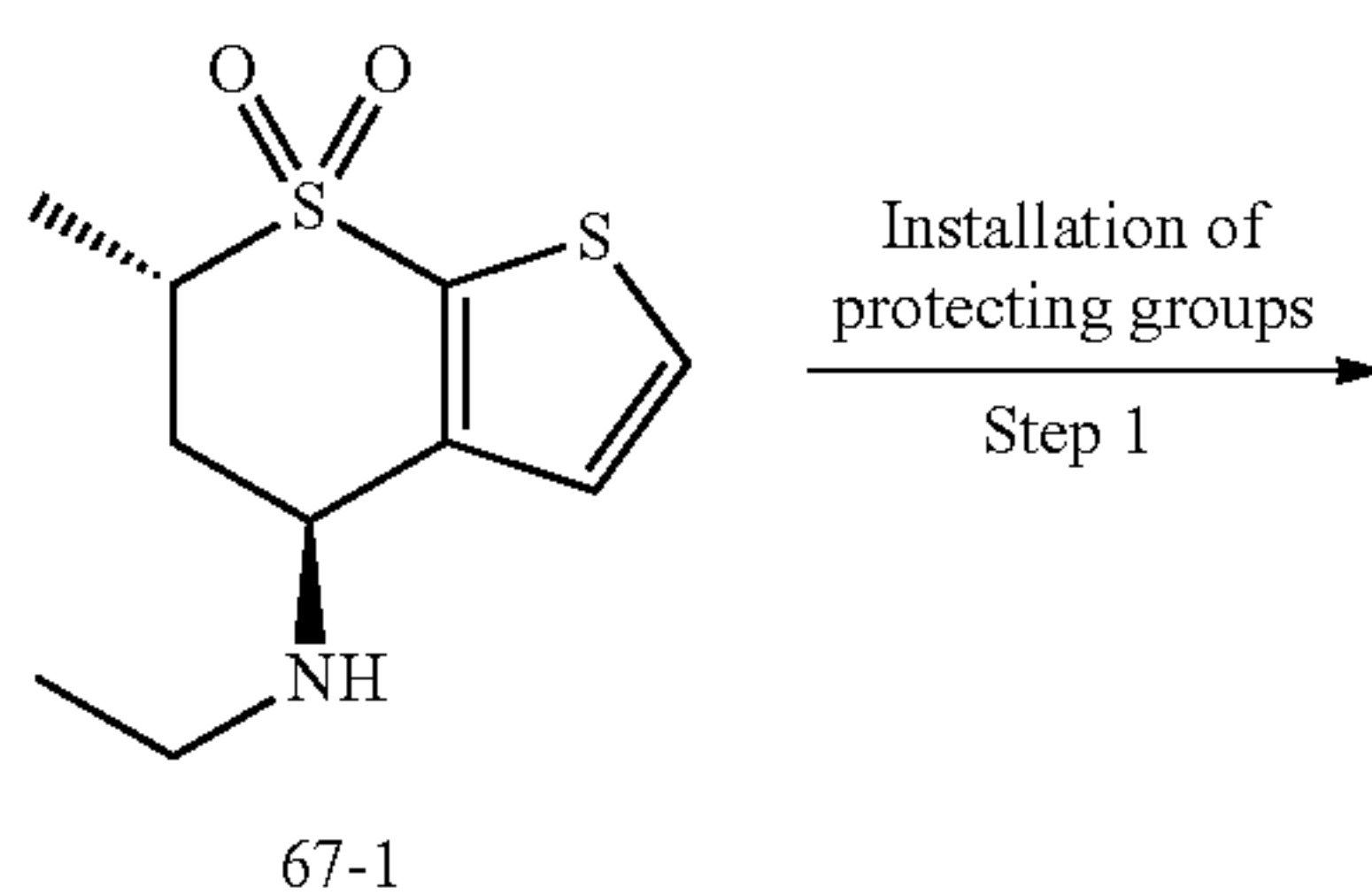
Scheme 67:
