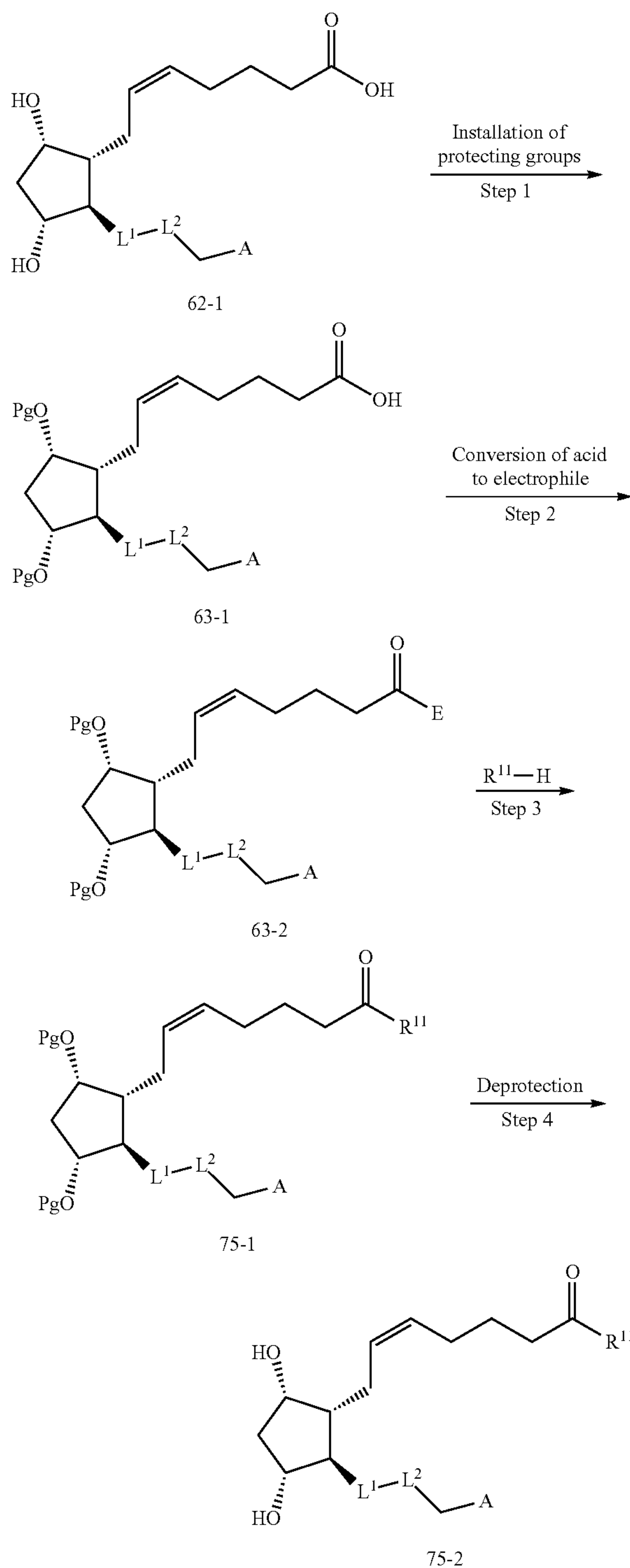
Scheme 75:
