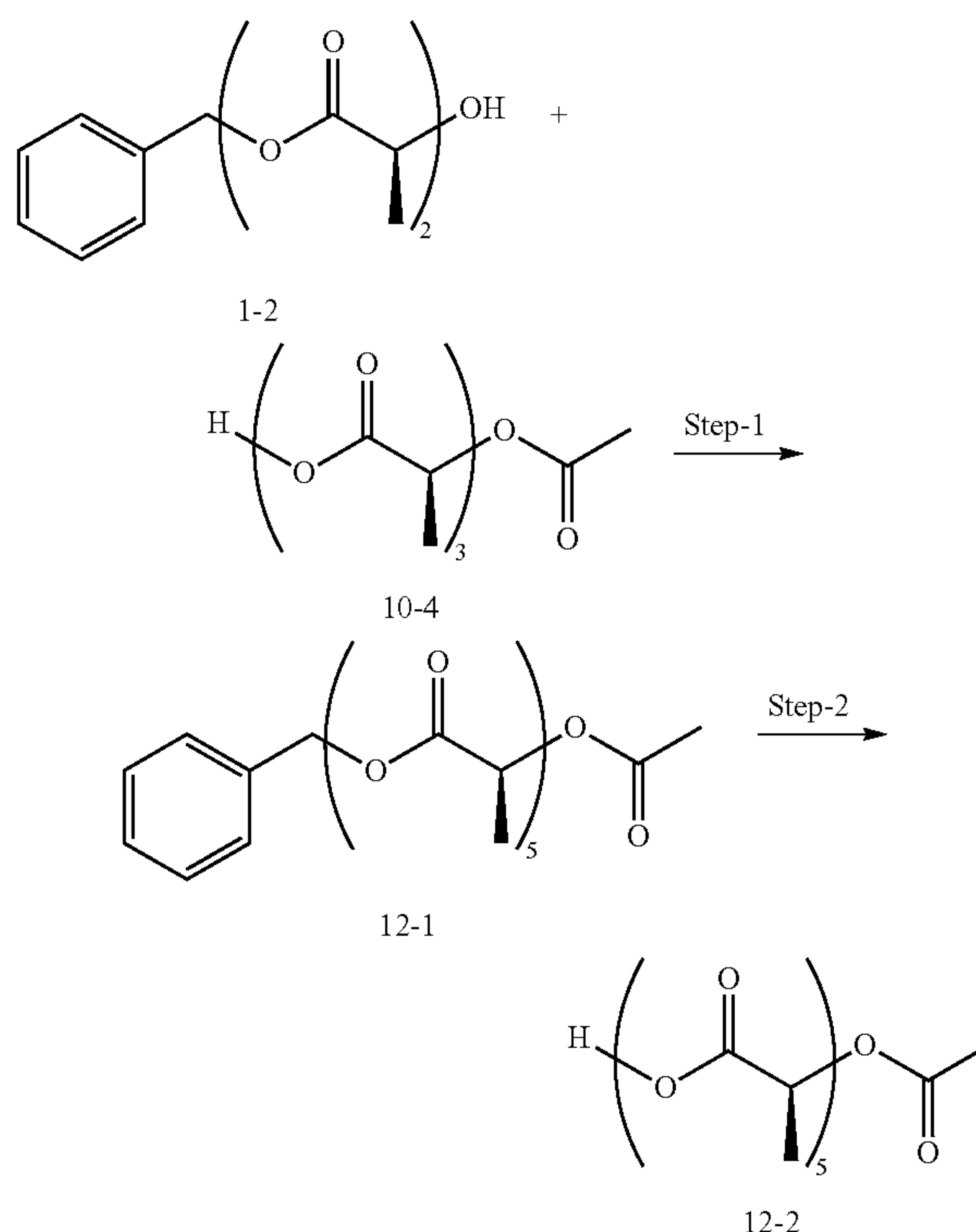
Scheme 12: (S)-2-((S)-2-[(S)-2-[(S)-2-((S)-2-Acetoxy-propionyloxy)-propionyloxy]-propionyloxy]-propionyloxy)-propionic acid (12-2):
