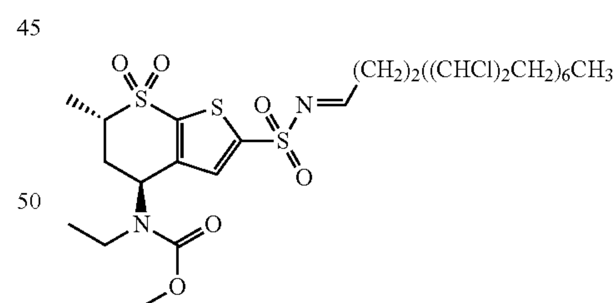
73-9
