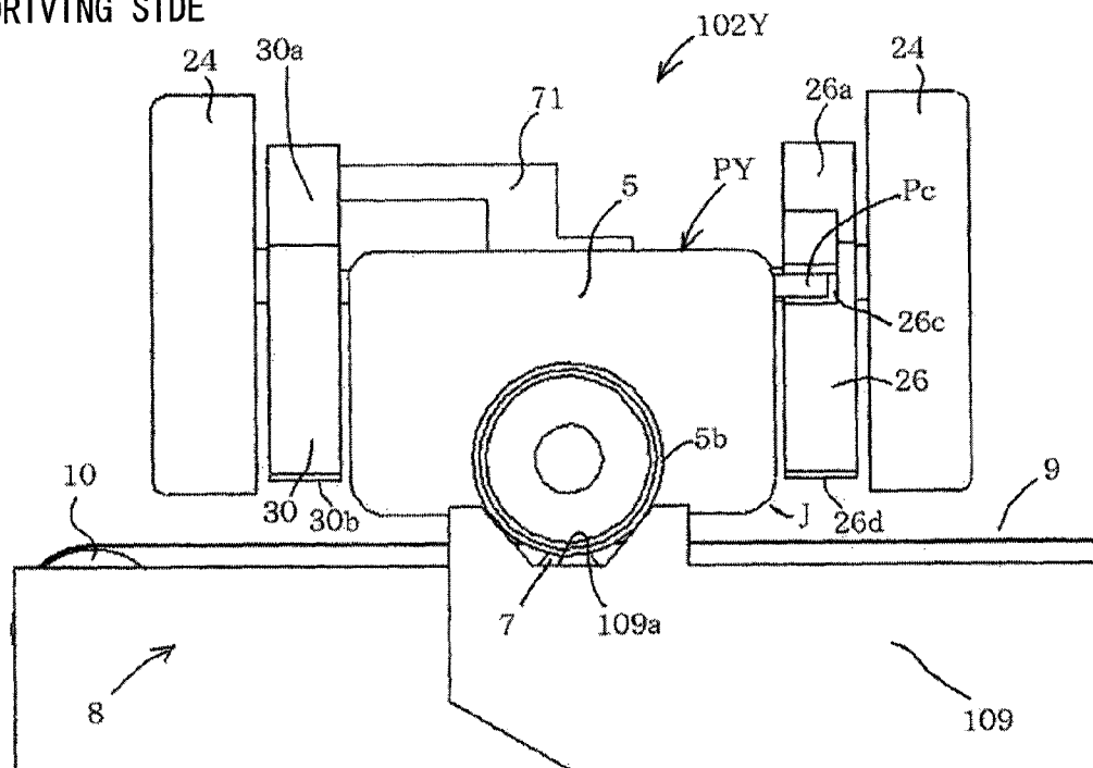
FIG. 7B DRIVING SIDE
