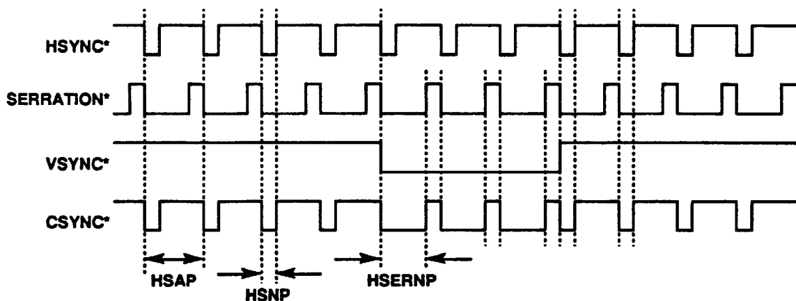
Horizontal Timing and Composite Sync Generation—Non-Interlaced Format
