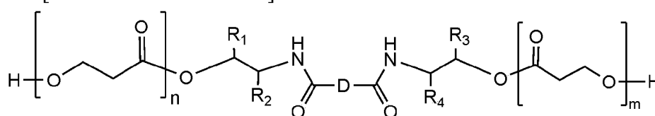
[Chemical Formula 2]
