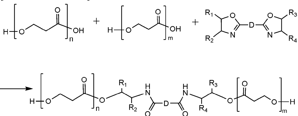
[Reaction Scheme 1]
