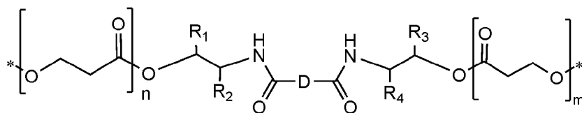
[Chemical Formula 1]
