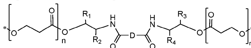
[Chemical Formula 1]
