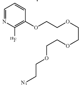
Synthesis of [ ^{18}\text{F} ]-3-(2-(2-(2-(2-azidoethoxy)ethoxy)ethoxy)ethoxy)-2-fluoropyridine
