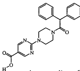
intermediate 6
