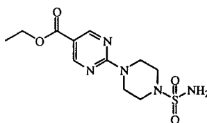
intermediate 10
