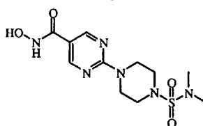
compound 2
