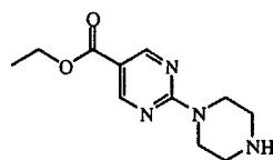
intermediate 2
