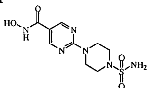
compound 3
