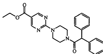
intermediate 5
