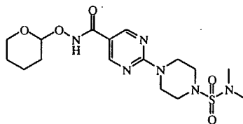
intermediate 9
