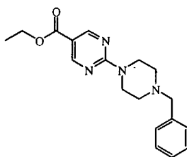
intermediate 1
