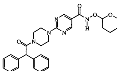
intermediate 7
