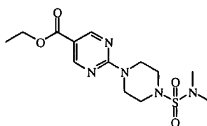
intermediate 3
