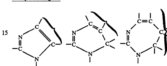
alkenylene bridge
