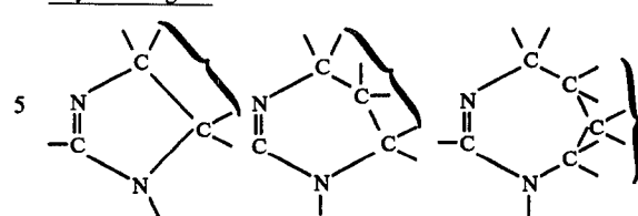
alkylene bridge
