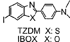
Thioflavin T
