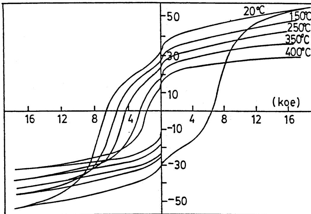
HYSTERESIS LOOPS IN C_{.76}Zr_{18}B_3Si_3 AT DIFFERENT TEMPERATURES.
