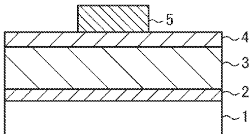
FIG. 13C PRIOR ART
