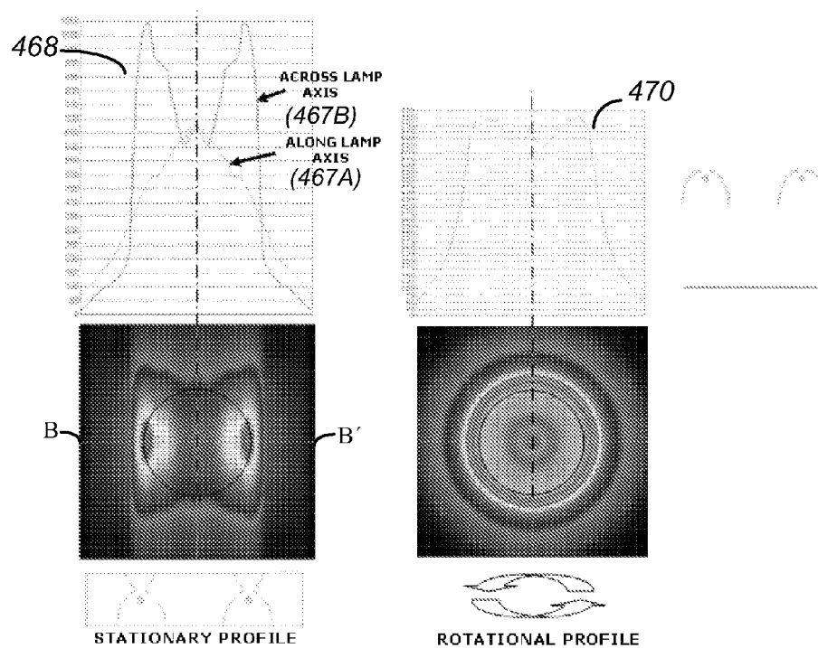
Primary Reflector (asymmetric) - dual lamp
