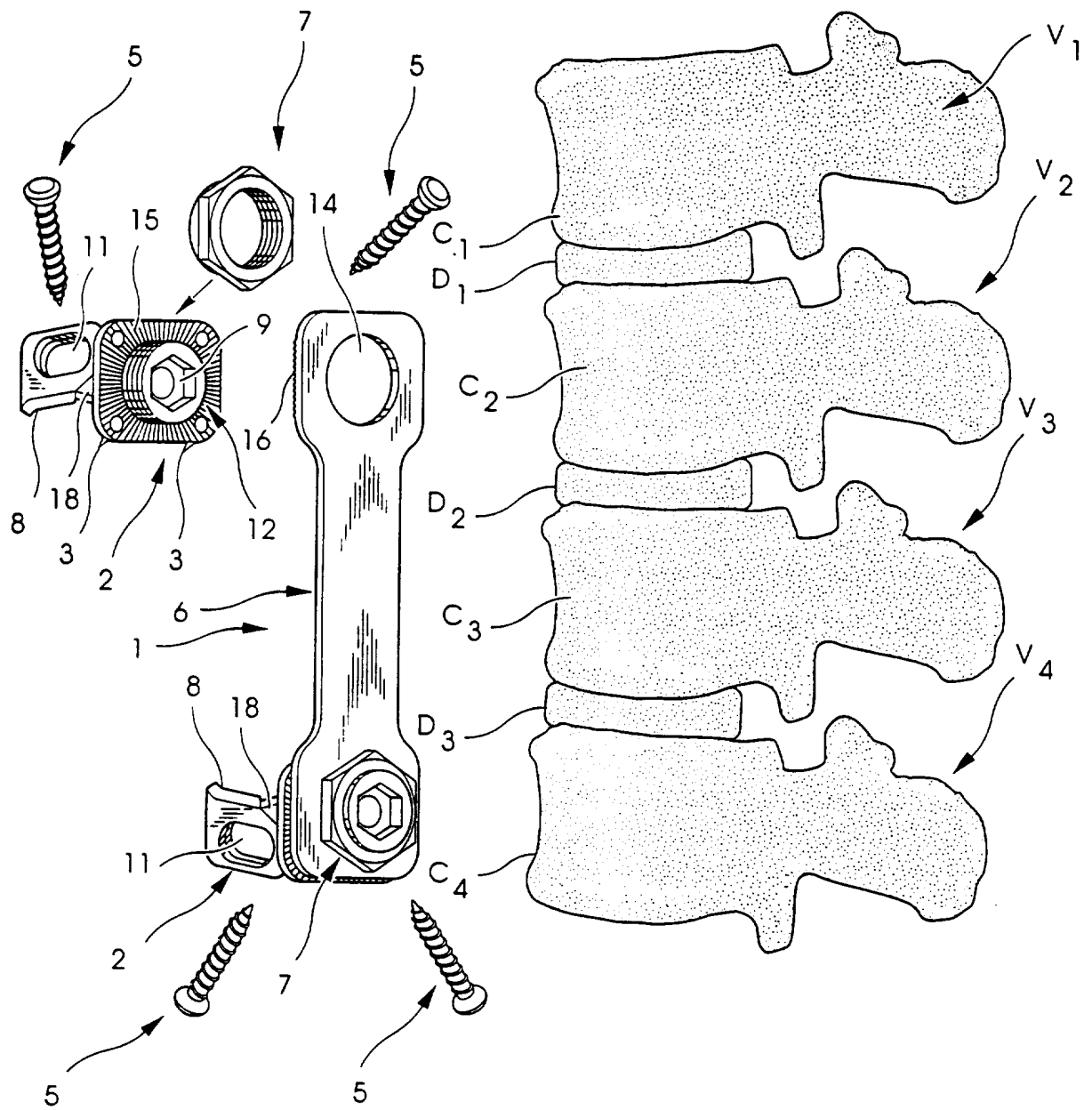
Fig. 1 (PRIOR ART)
