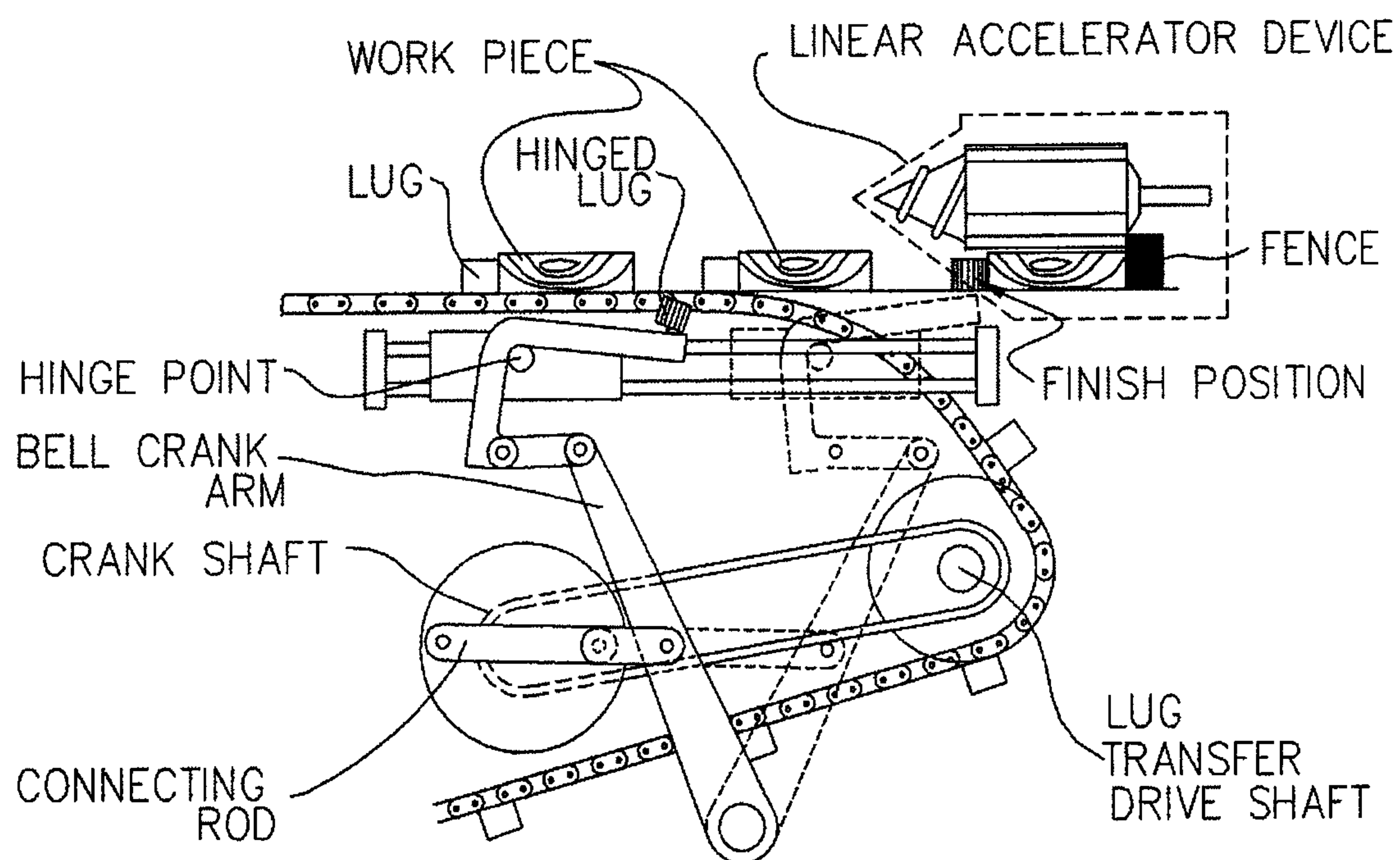
Fig 19 TRANSVERSE ACCELERATION DEVICE SLIDER CRANK TYPE
