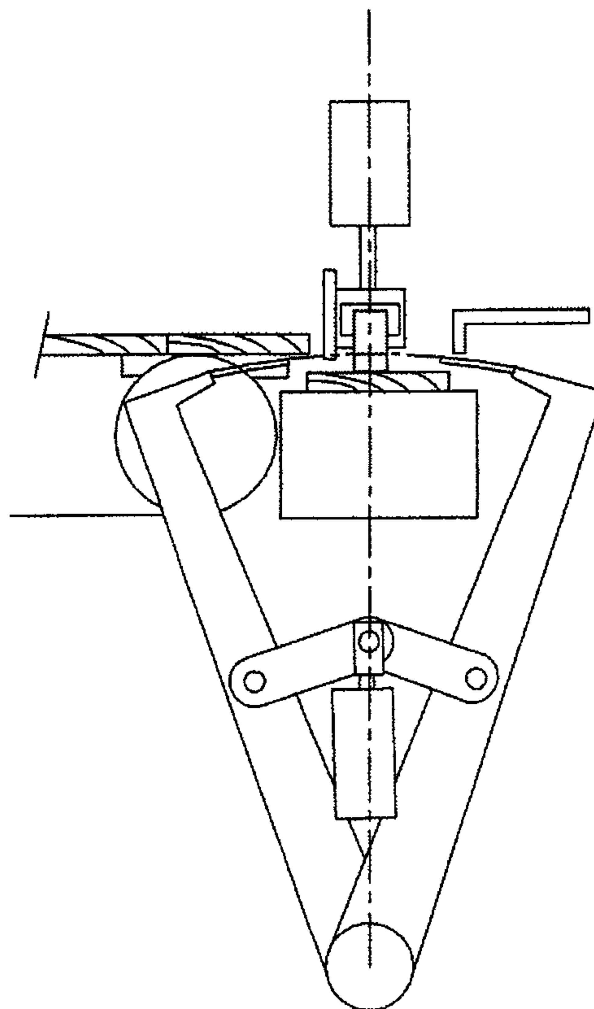
Fig 14b ALTERNATE SHEET FED VERTICAL ACCELERATION
