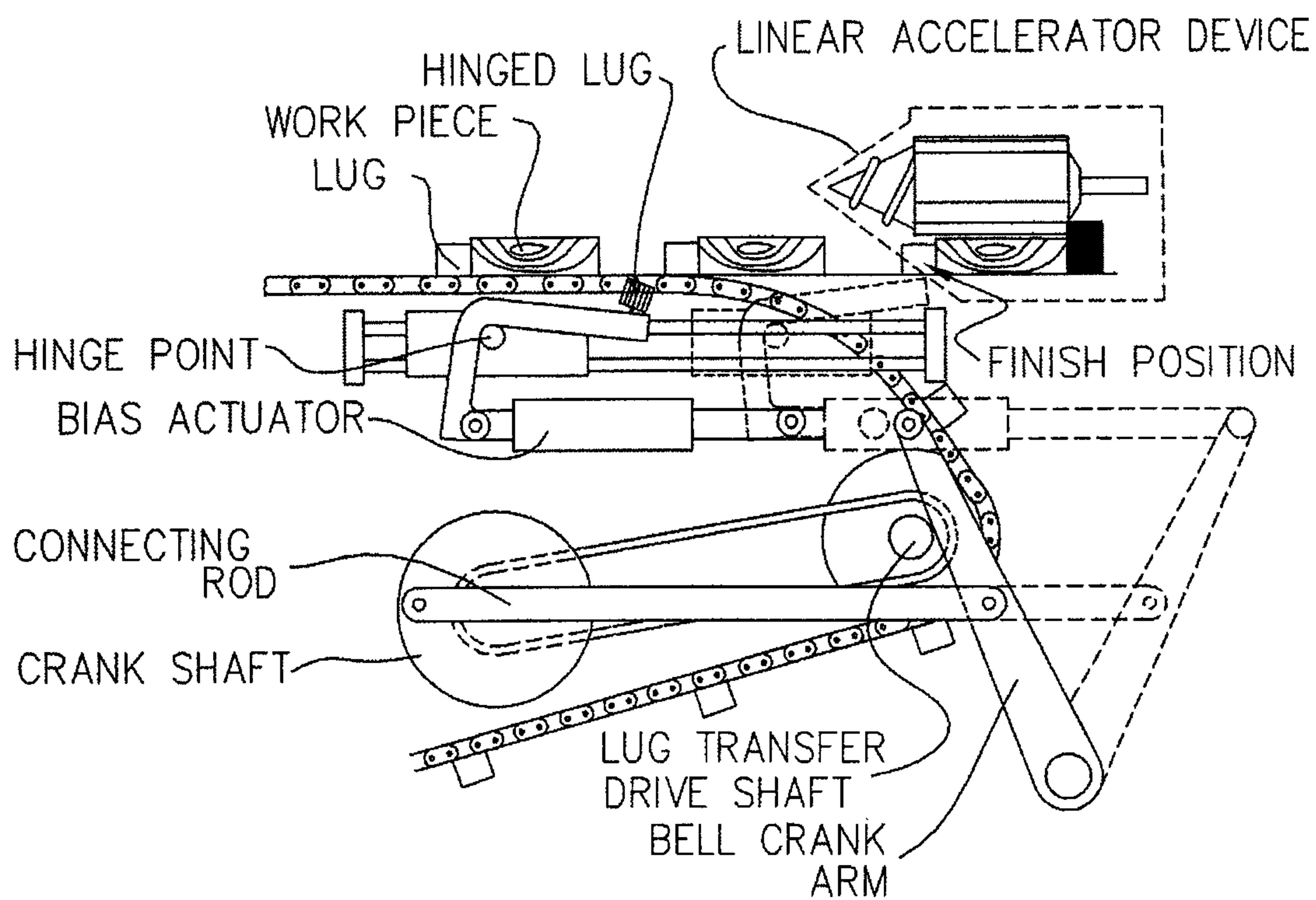
Fig 20 TRANSVERSE ACCELERATION DEVICE
