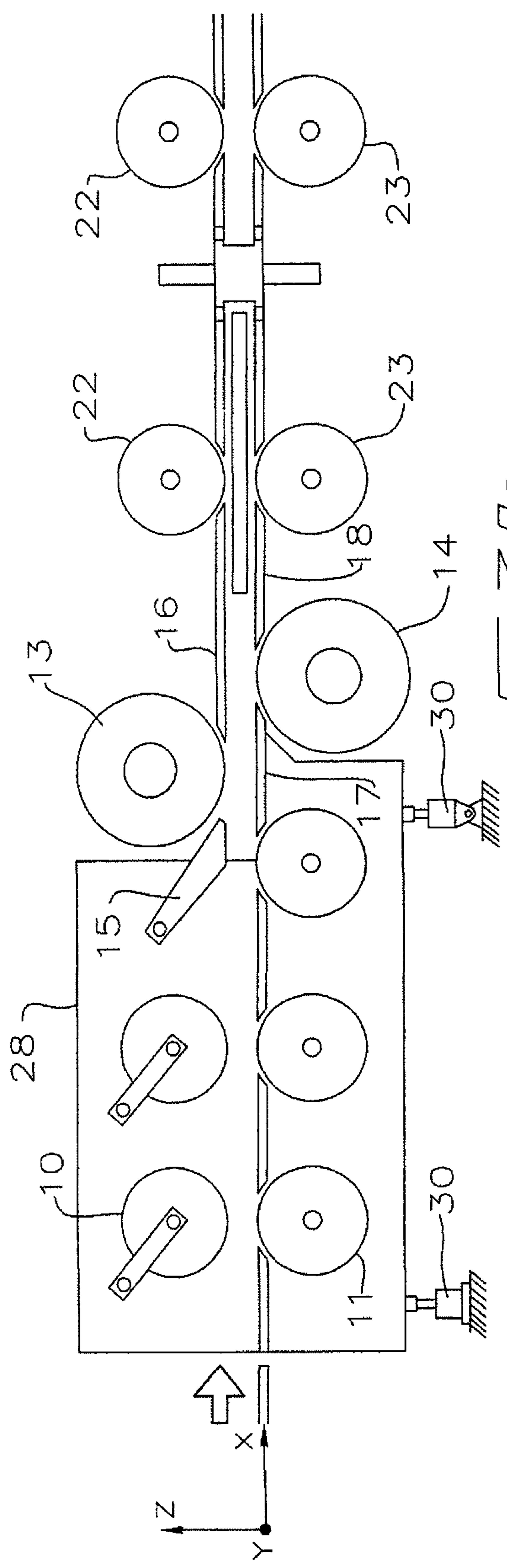
OPTIMIZING PLANNER-THREE AXIS INFED POSITIONING MODULE WITH INTERMEDIATE SIDE HEAD STEERING
