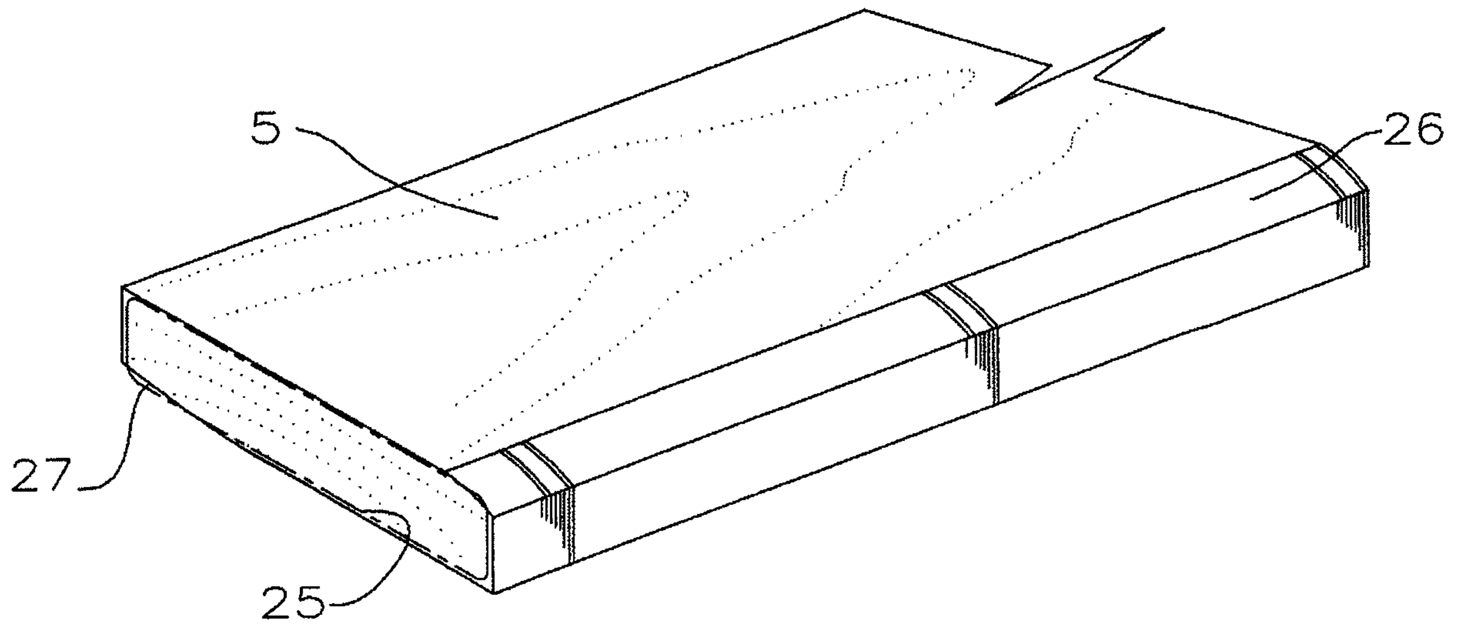
NON-OPTIMIZED PLANING OF A WORK PIECE
