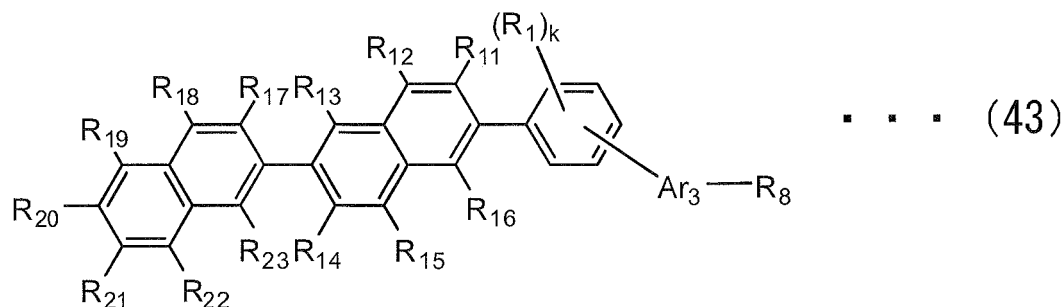
[Chemical Formula 72]
