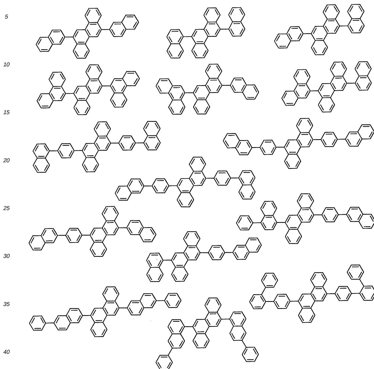
[Chemical Formula 46]
