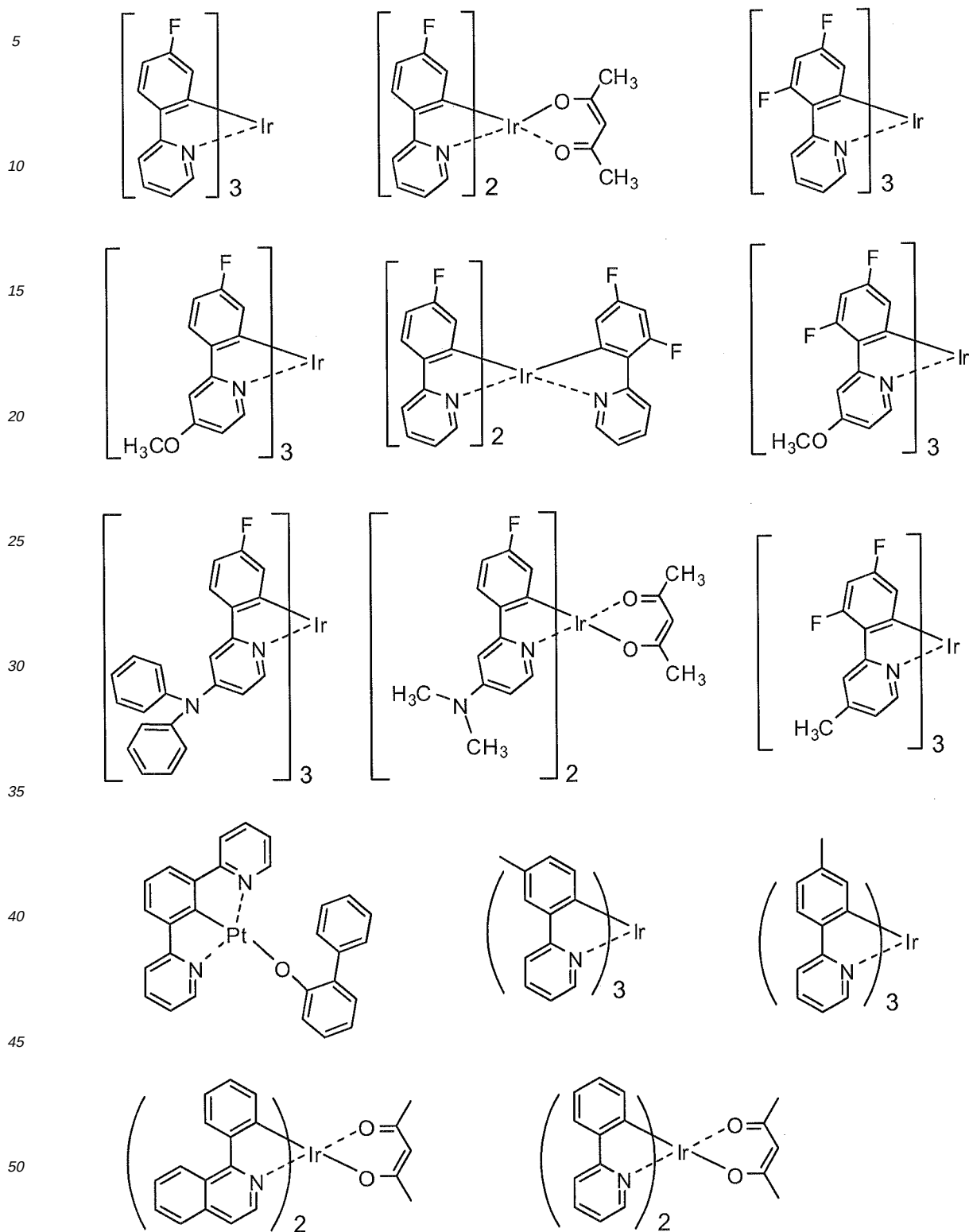
[Chemical Formula 104]
