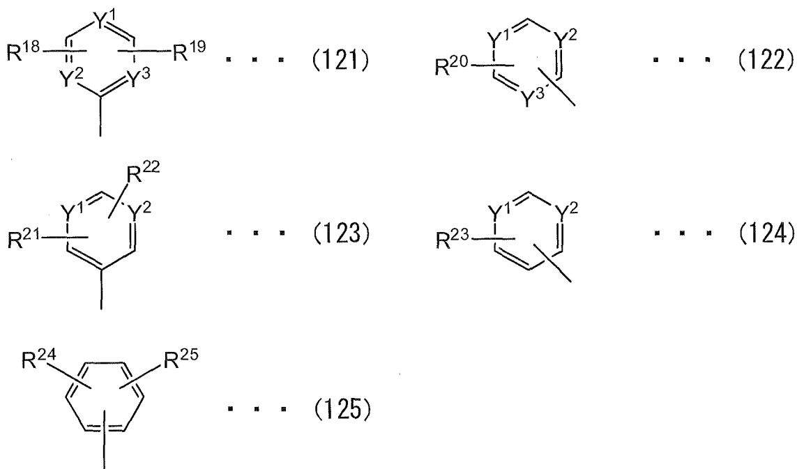
[Chemical Formula 11]
