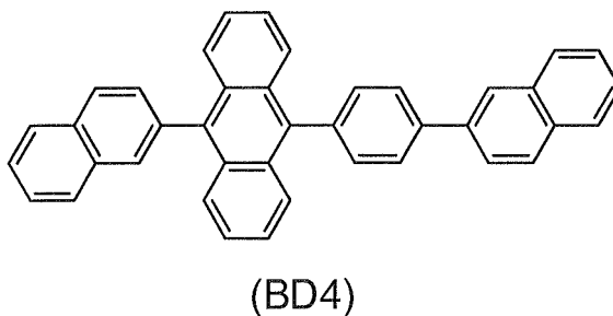
[Chemical Formula 180]
