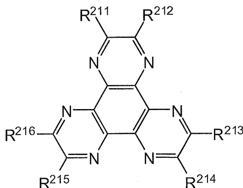
[Chemical Formula 170]
