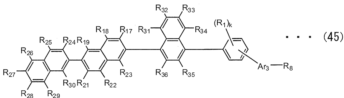
[Chemical Formula 74]
