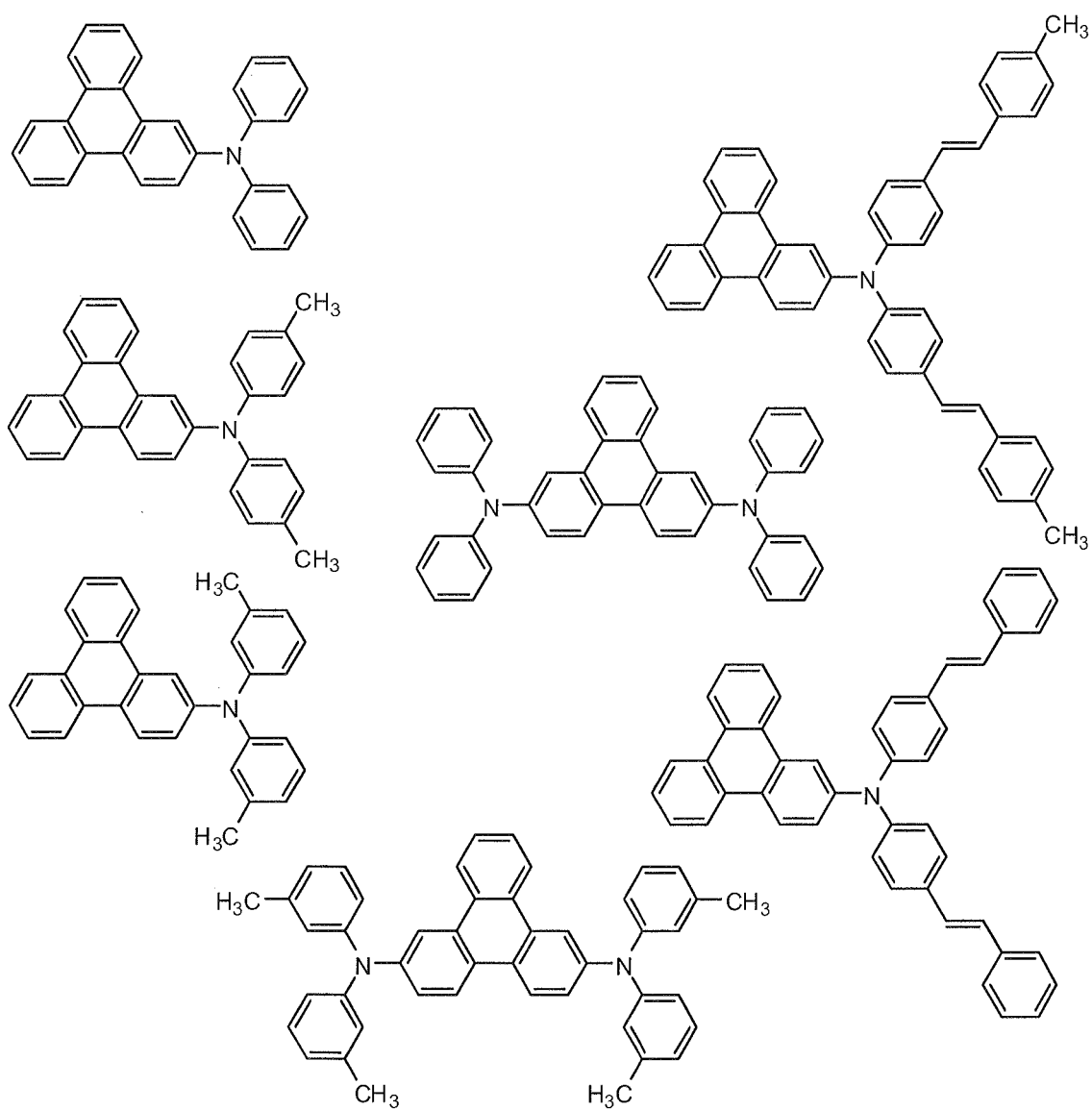
[Chemical Formula 63]
