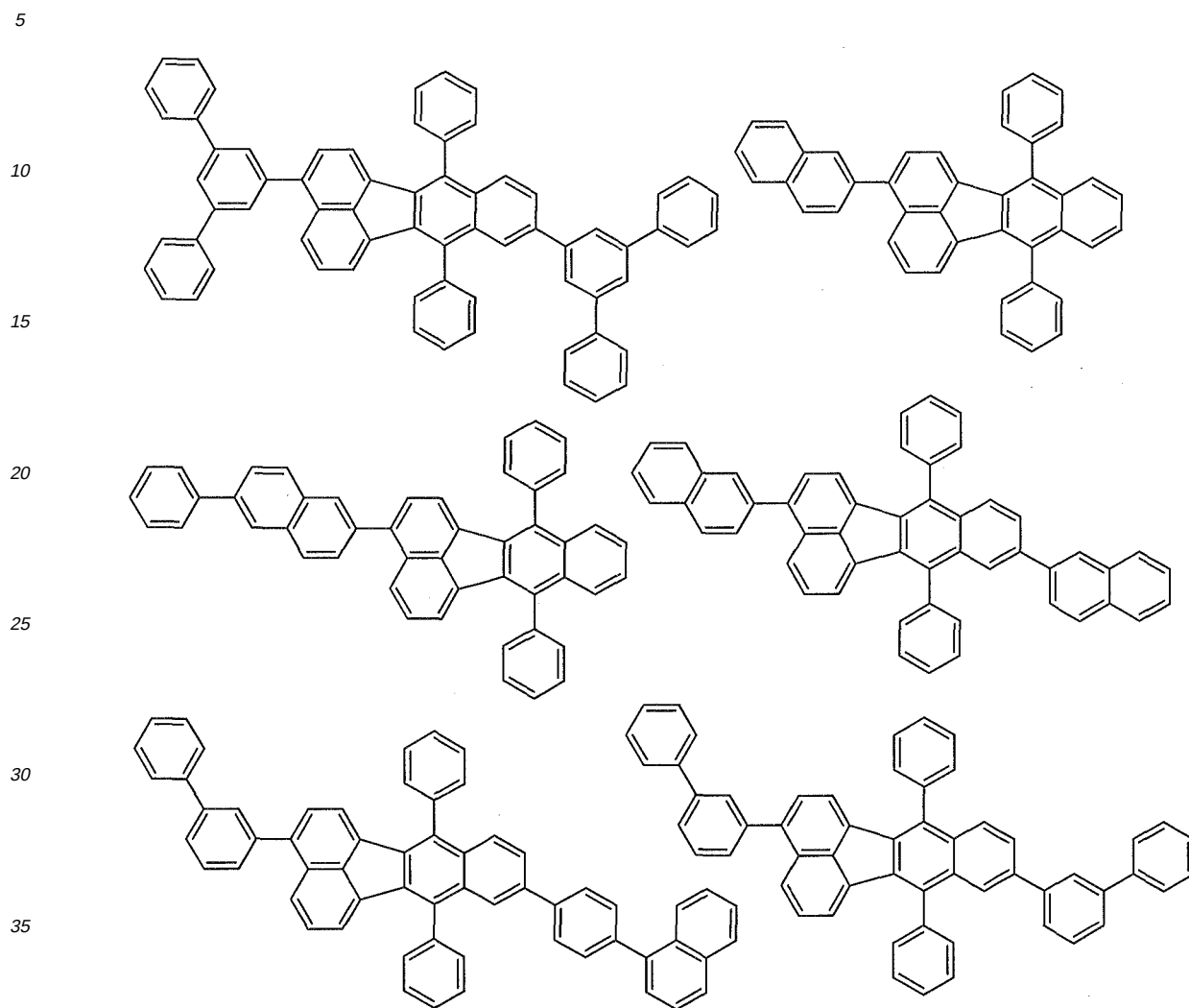
[Chemical Formula 61]
