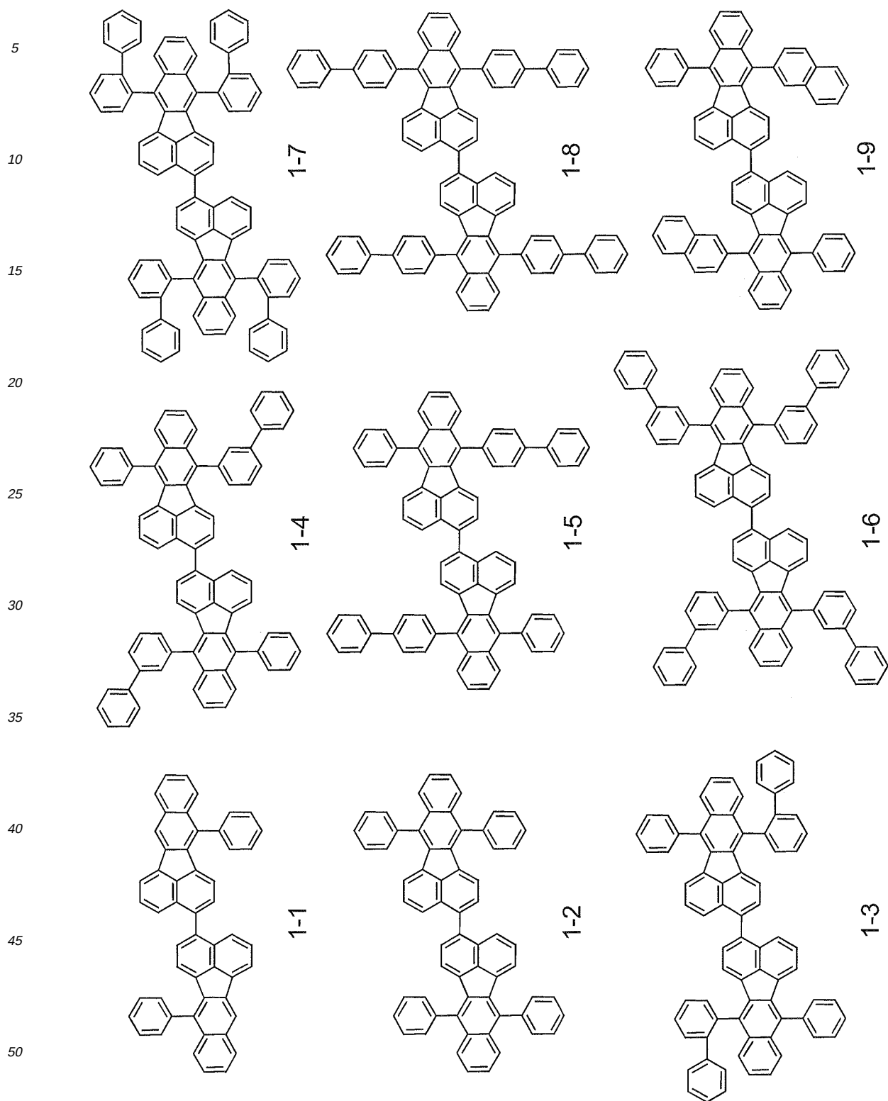
[Chemical Formula 132]
