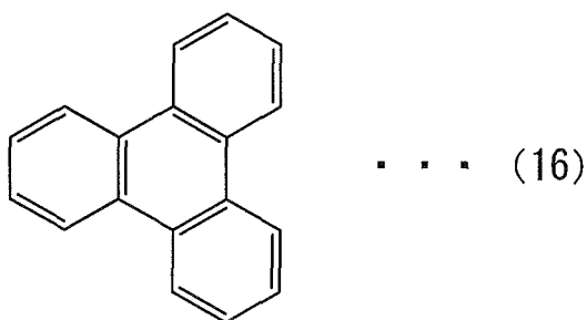
[Chemical Formula 62]
