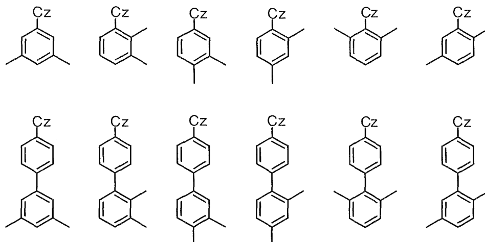
[Chemical Formula 10]
