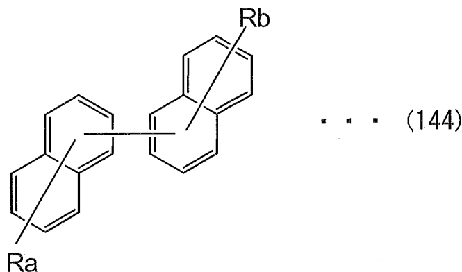
[Chemical Formula 101]
