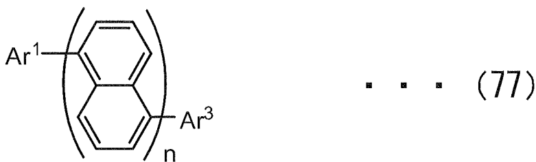
[Chemical Formula 84]
