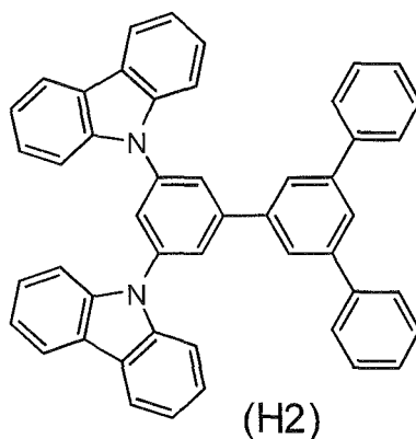
[Chemical Formula 174]
