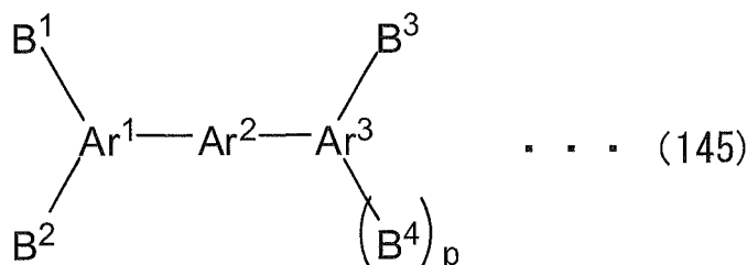
[Chemical Formula 102]
