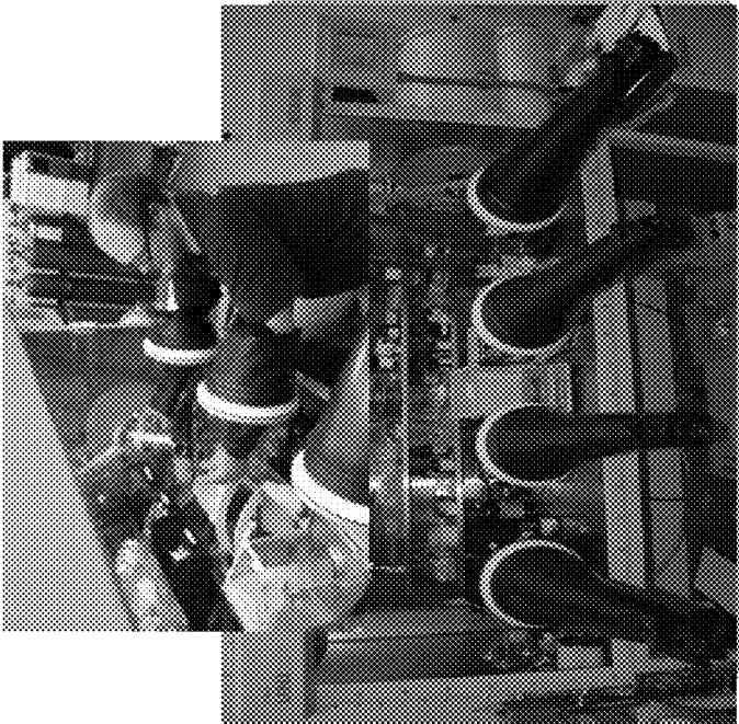
Sample synthesis
