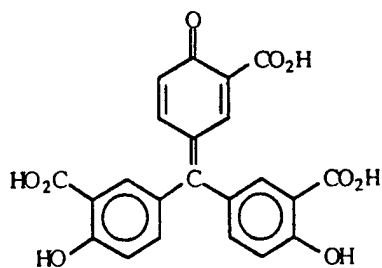
Aurintricarboxylic Acid
