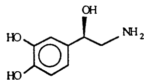
Norepinephrine
