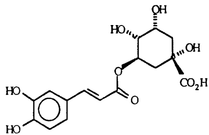
Chlorogenic Acid
