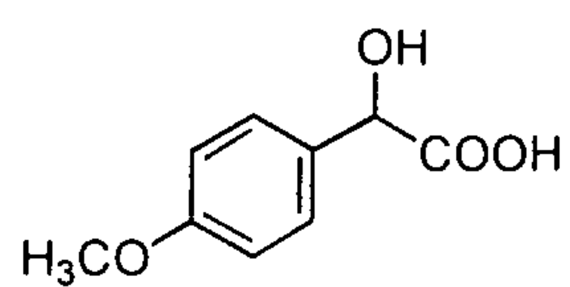
methoxy-mandelic acid
