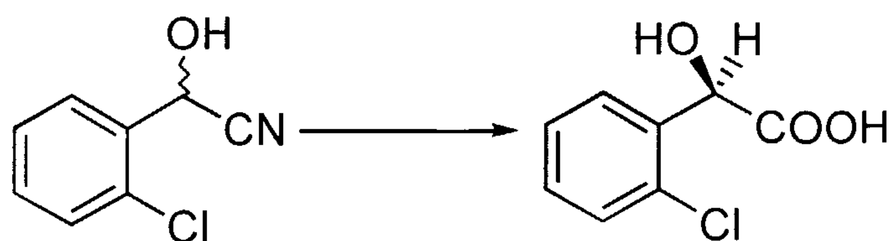
(R) -2-chloromandelic acid
