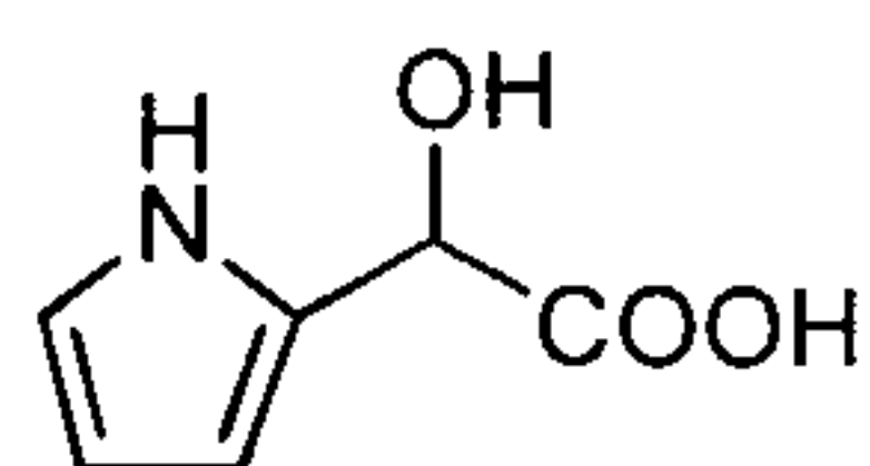
1-pyrrole glycolic acid
