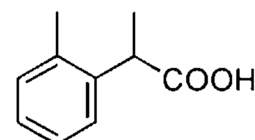
methyl-mandelic acid
