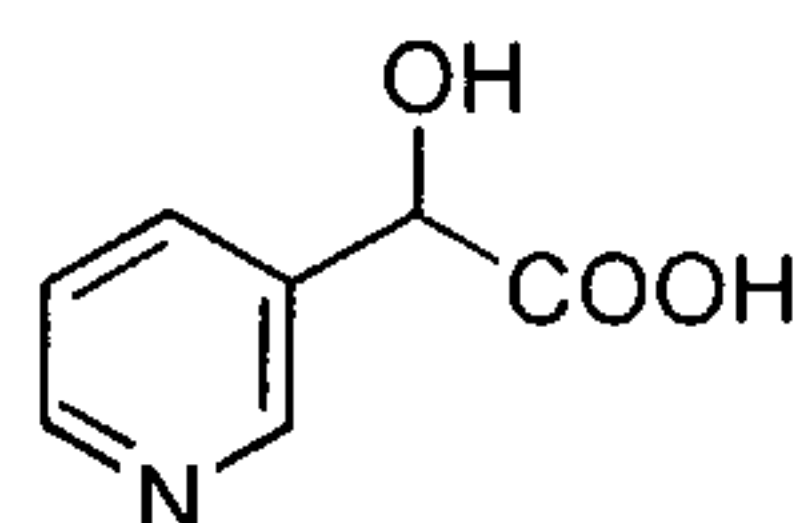
3-pyridyl glycolic acid
