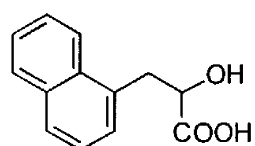
naphthyl acetic acid
