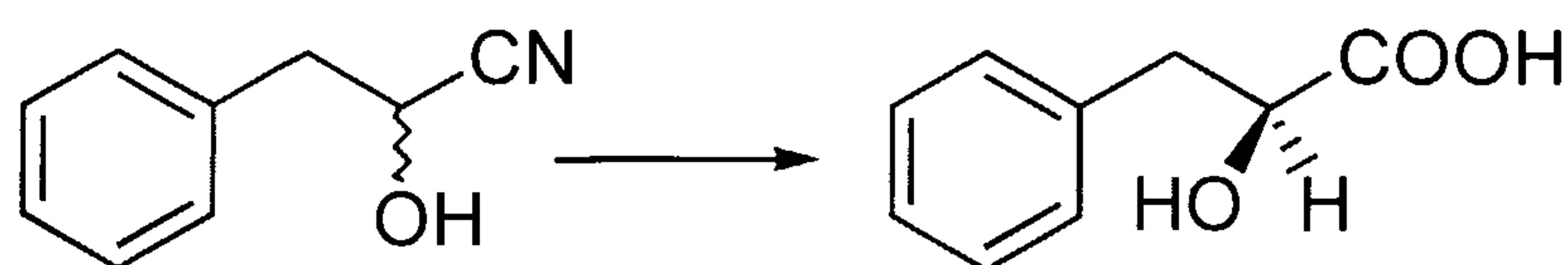
Phenylacetaldehyde cyanohydrin
