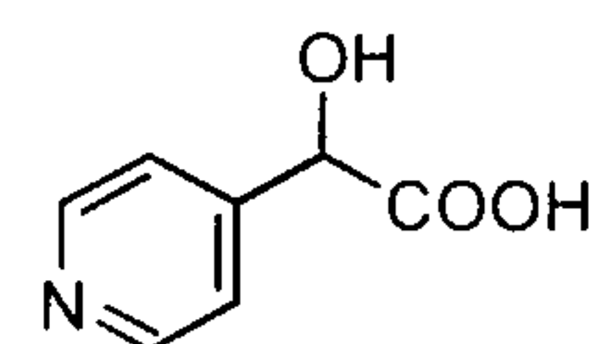
4-pyridyl glycolic acid
