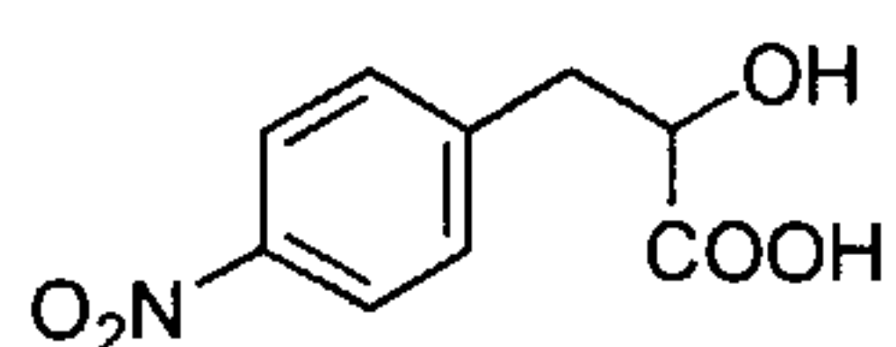
nitro phenyl lactic acid
