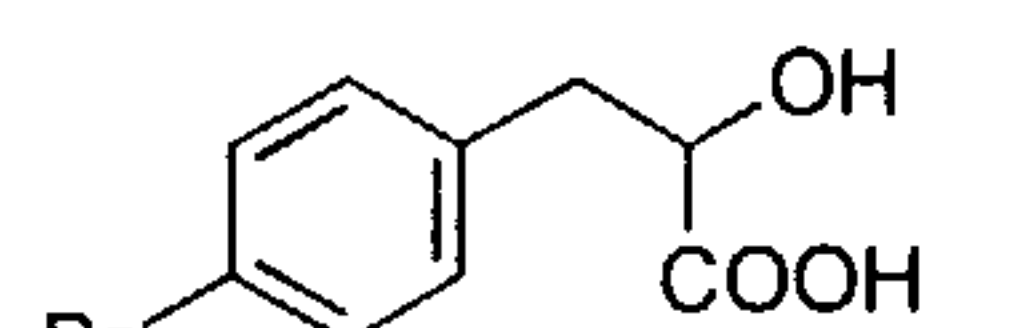
bromophenyl lactic acid
