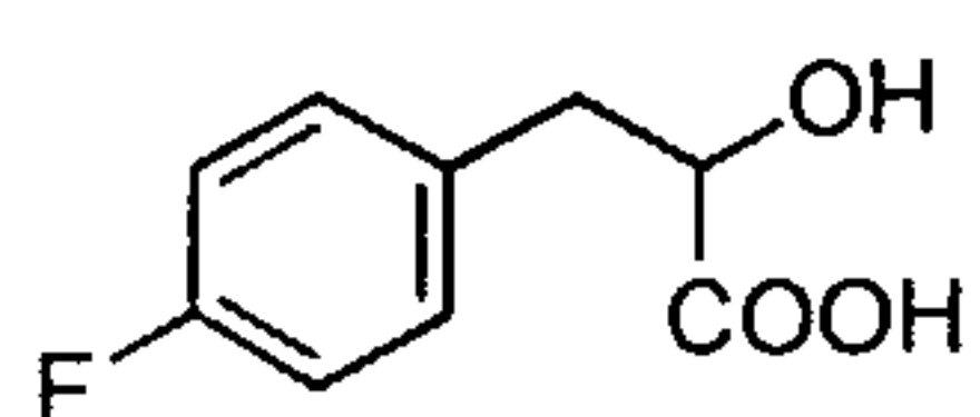
fluorophenyl lactic acid
