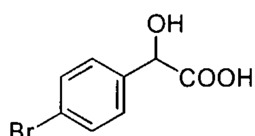
bromo-mandelic acid
