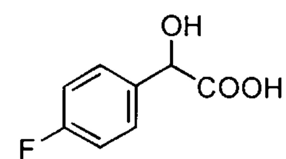
fluoro-mandelic acid
