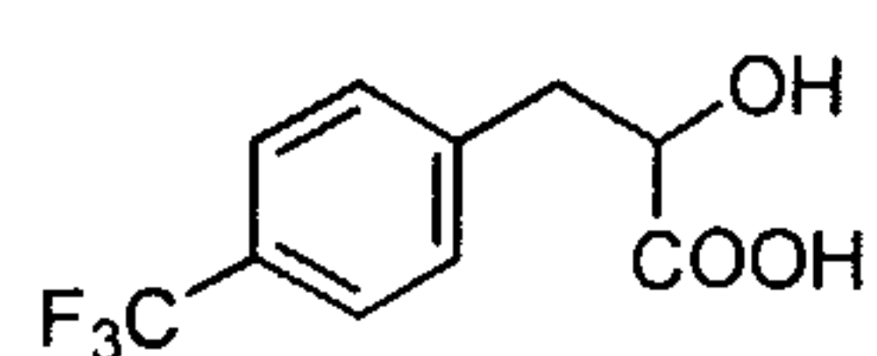
trifluoromethylphenyl lactic acid
