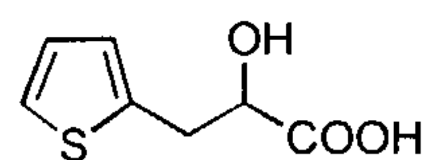
thienyl acetic acid
