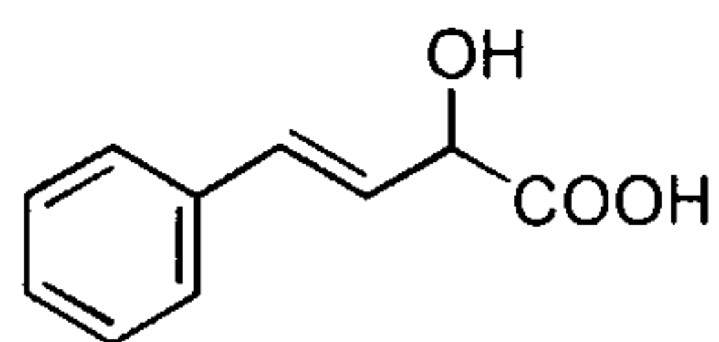
4-phenyl-2-hydroxy-3,4-butenic acid
