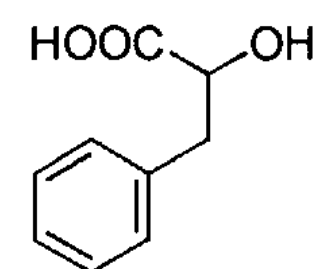
phenyl lactic acid
