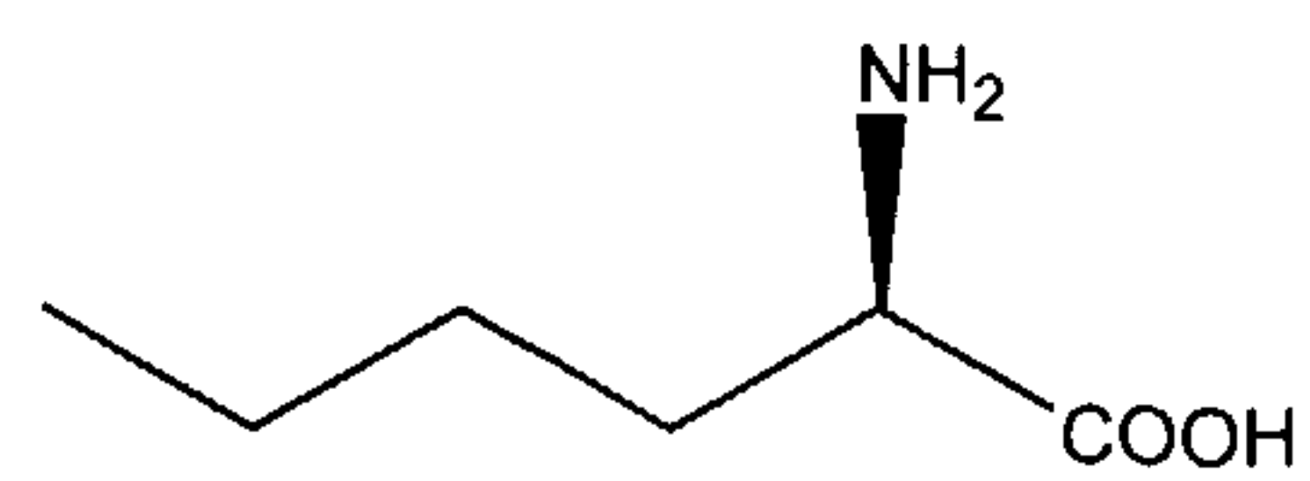
D-norleucine
