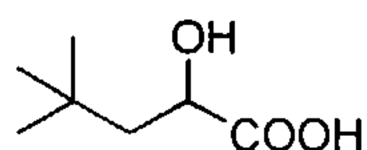
2-hydroxy-4-di-methyl-pentanoic acid
