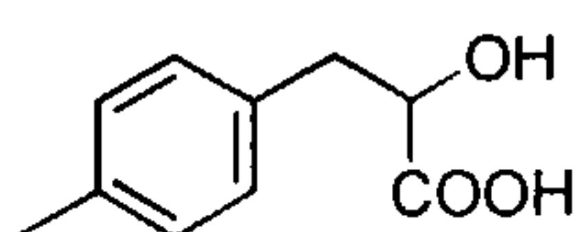
methyl phenyl lactic acid
