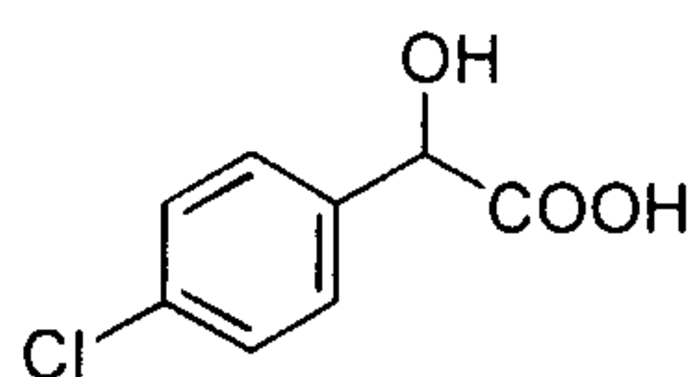
chloro-mandelic acid
