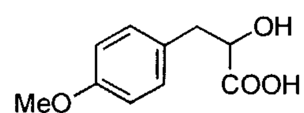
methoxy phenyl lactic acid
