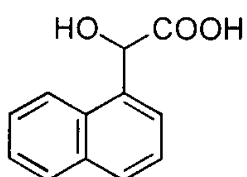
1-naphthyl glycolic acid
