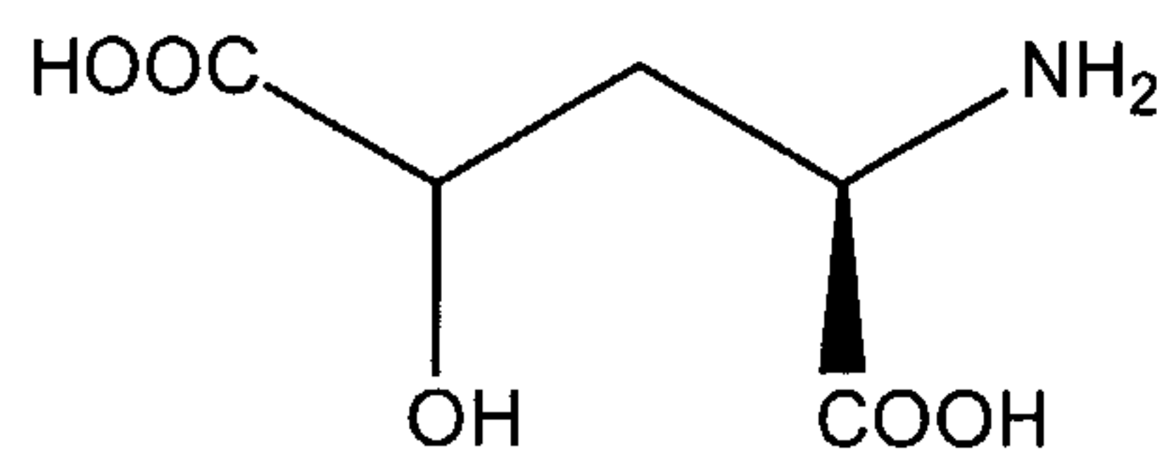
D-gamma-hydroxy glutamate
