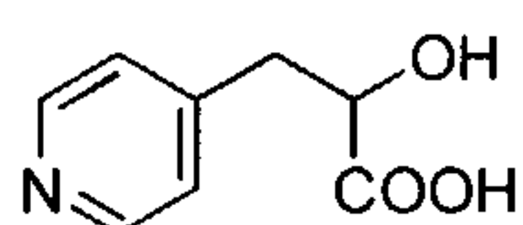
pyridyl acetic acid
