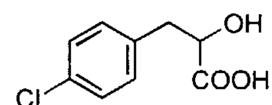
chlorophenyl lactic acid
