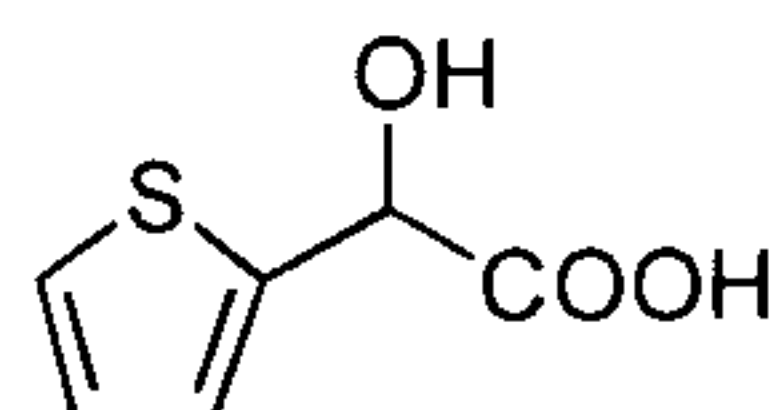
2-thienyl glycolic acid
