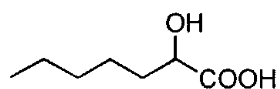
2-hydroxy heptanoic acid
