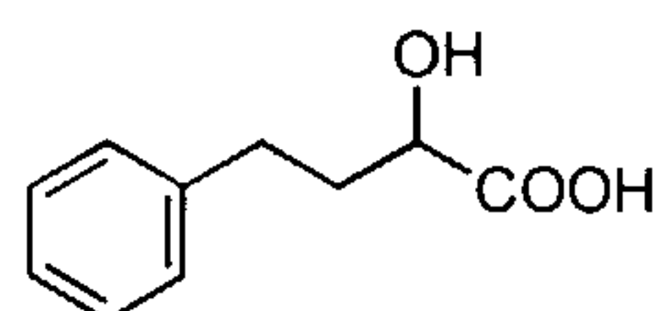
4-phenyl-2-hydroxyphenyl butanoic acid
