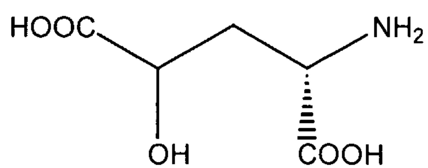
L-gamma-hydroxy glutamate
