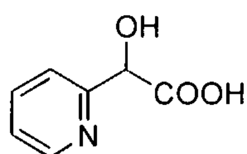
2-pyridyl glycolic acid
