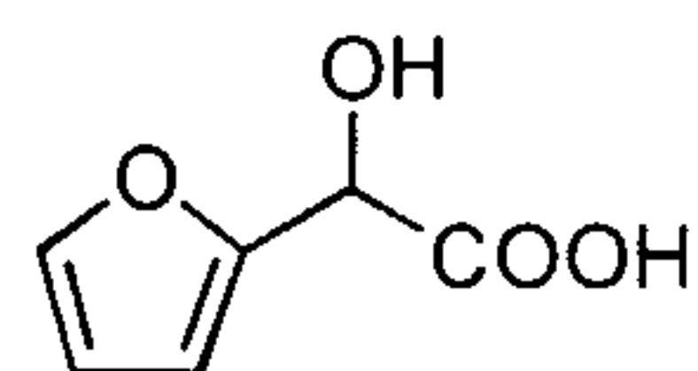
2-furanyl glycolic acid
