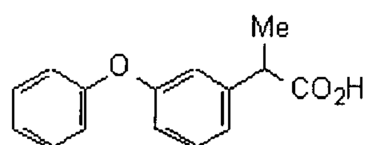
Fenoprofen
