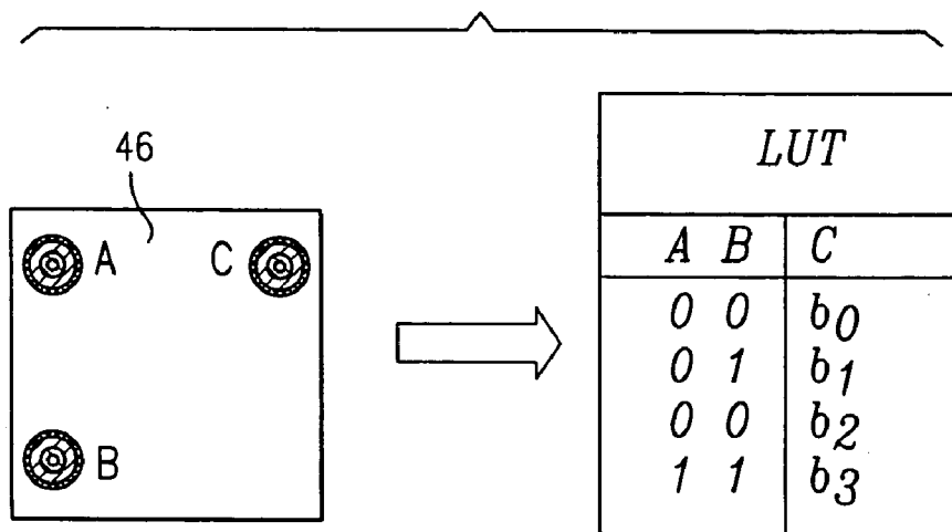
LOOK UP TABLE 2 INPUTS 1 OUTPUT
