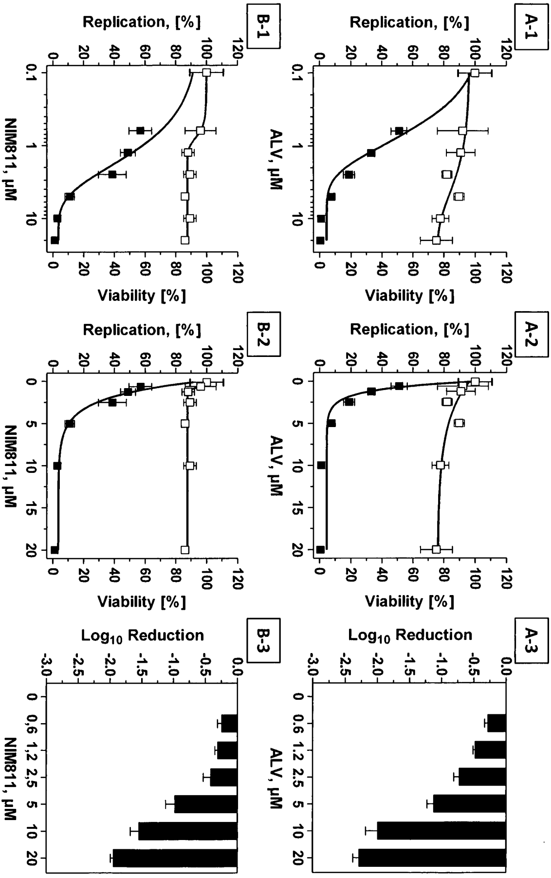
Inhibition of feline Coronavirus (FCoV-LUC) replication by ALV, NIM811
