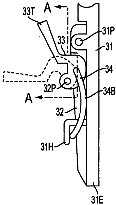
FIG. 5A (PRIOR ART)
