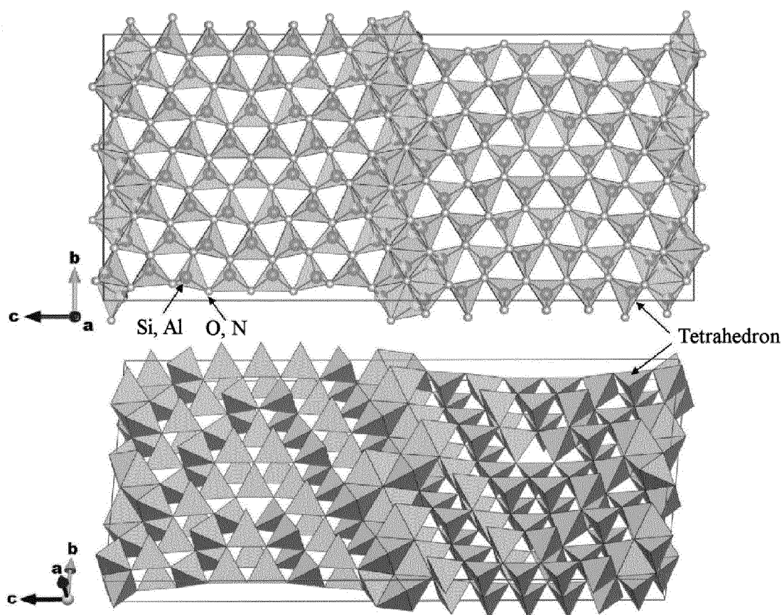
Crystal structure of \text{Si}_x\text{Al}_{14-x}\text{O}_{3-x}\text{N}_{12+x}
