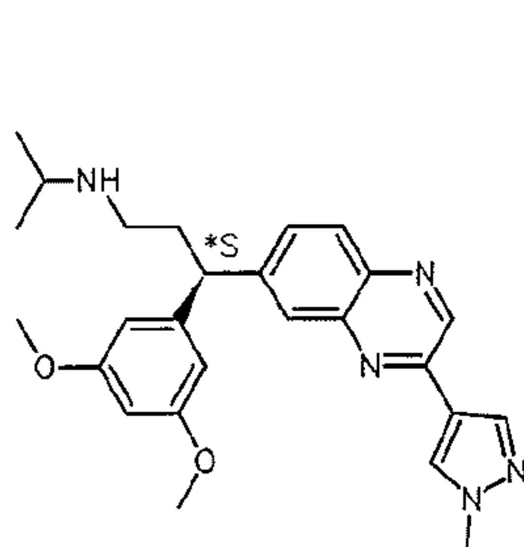
Compound 19
