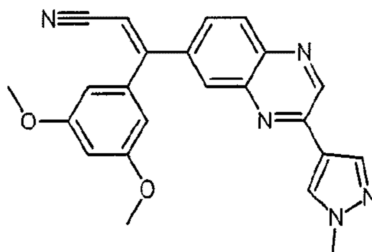
compound 4
