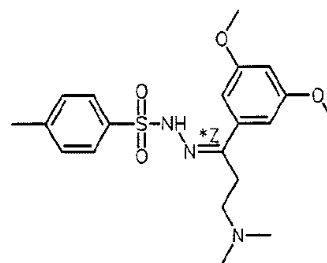
intermediate 12
