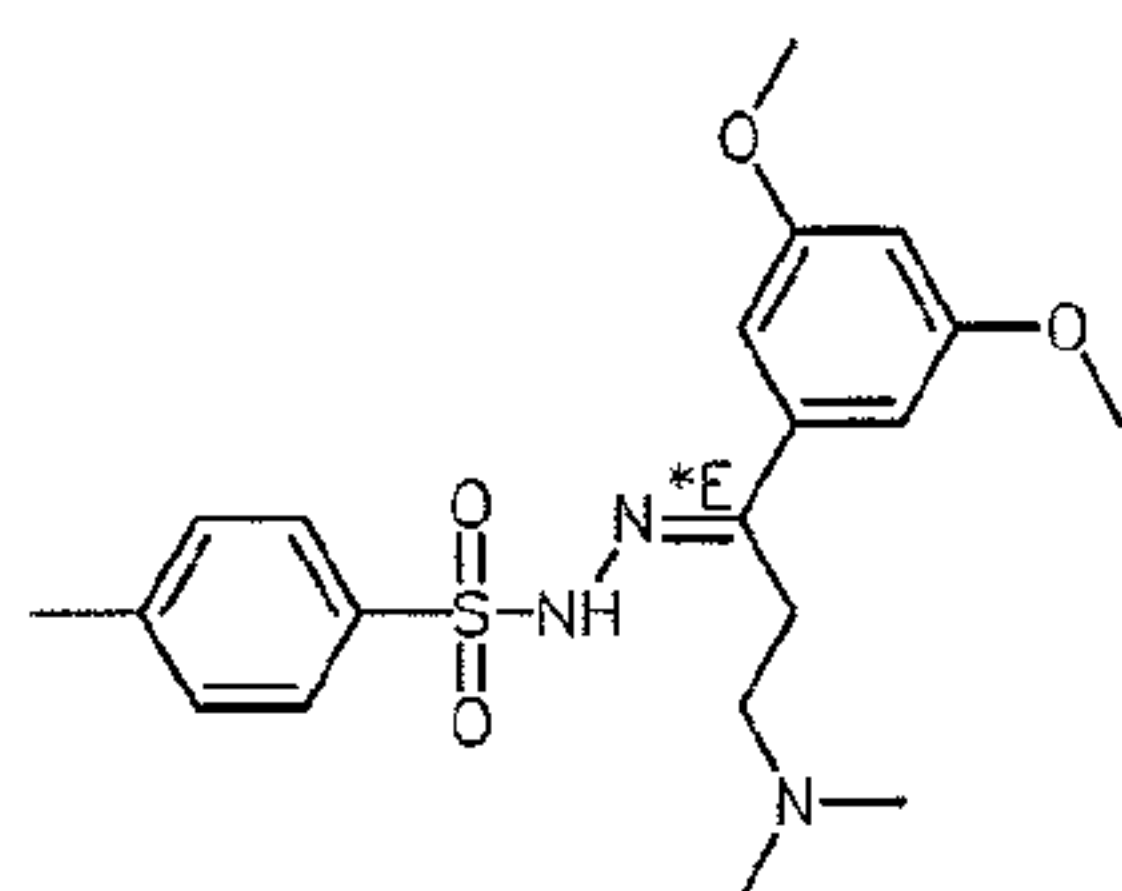
intermediate 11
