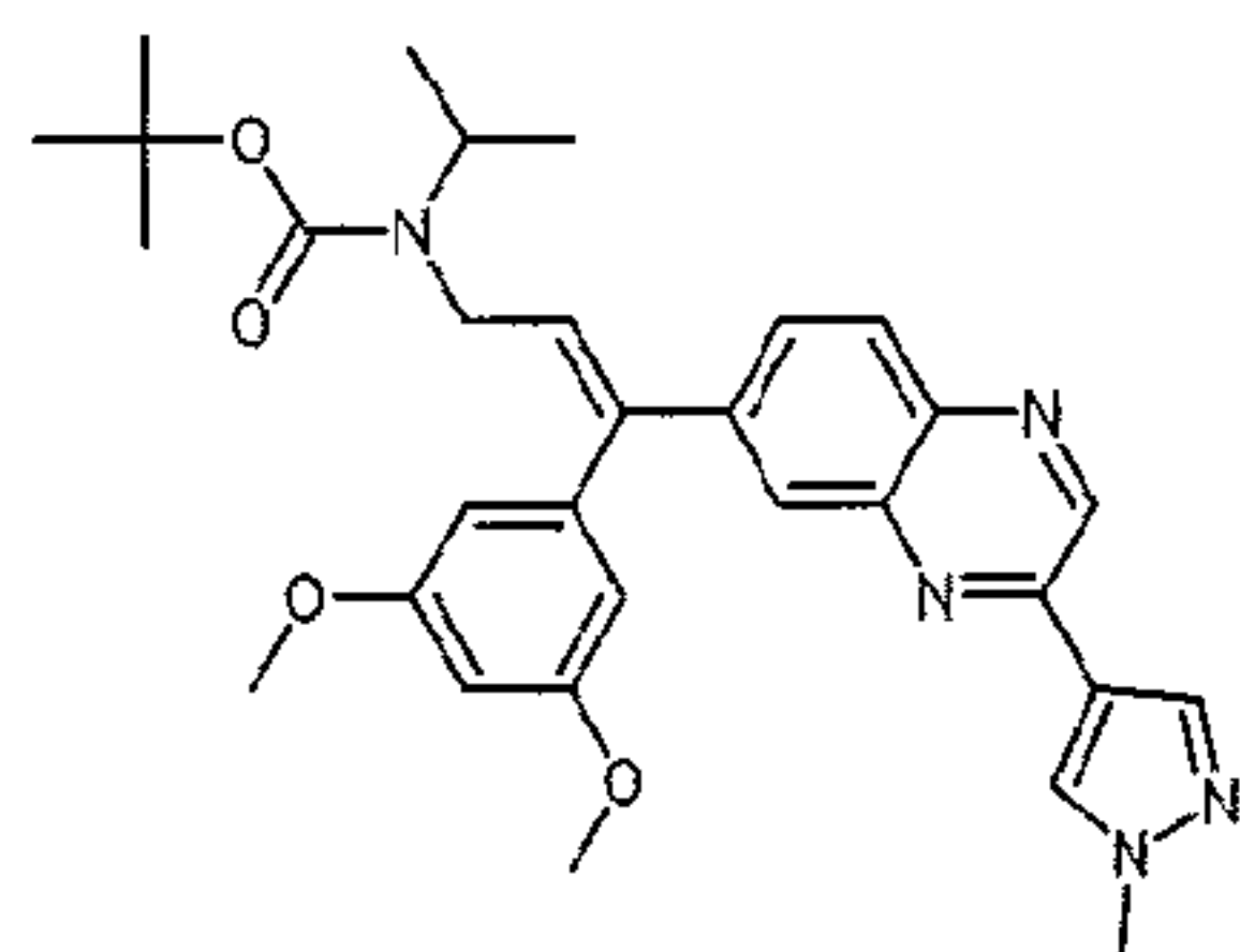
intermediate 9 (Z)
