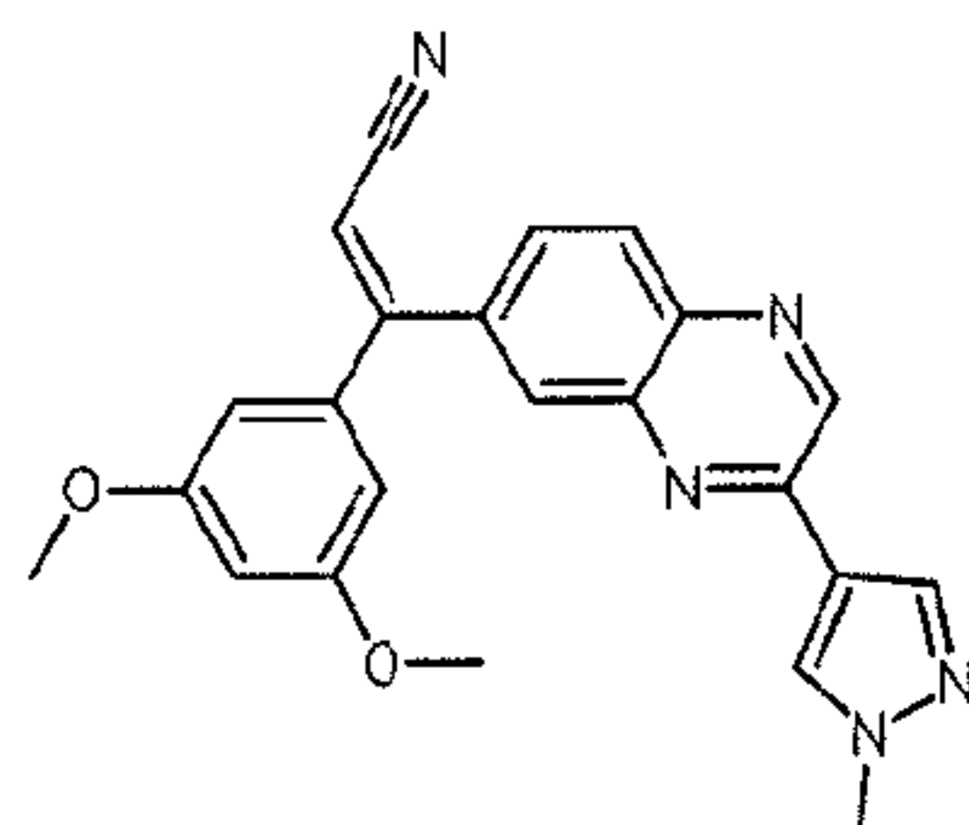
compound 3
