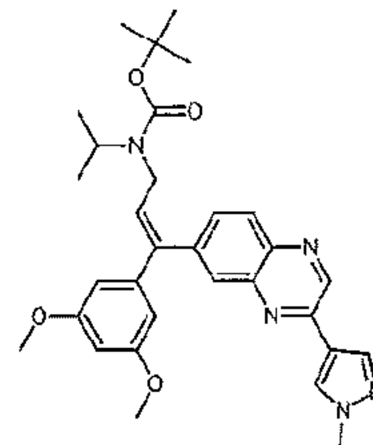
intermediate 10 (E)
