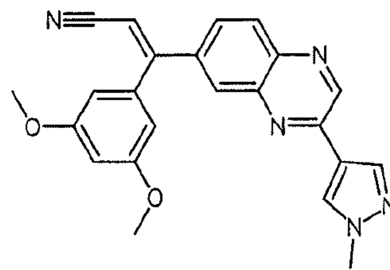
compound 4
