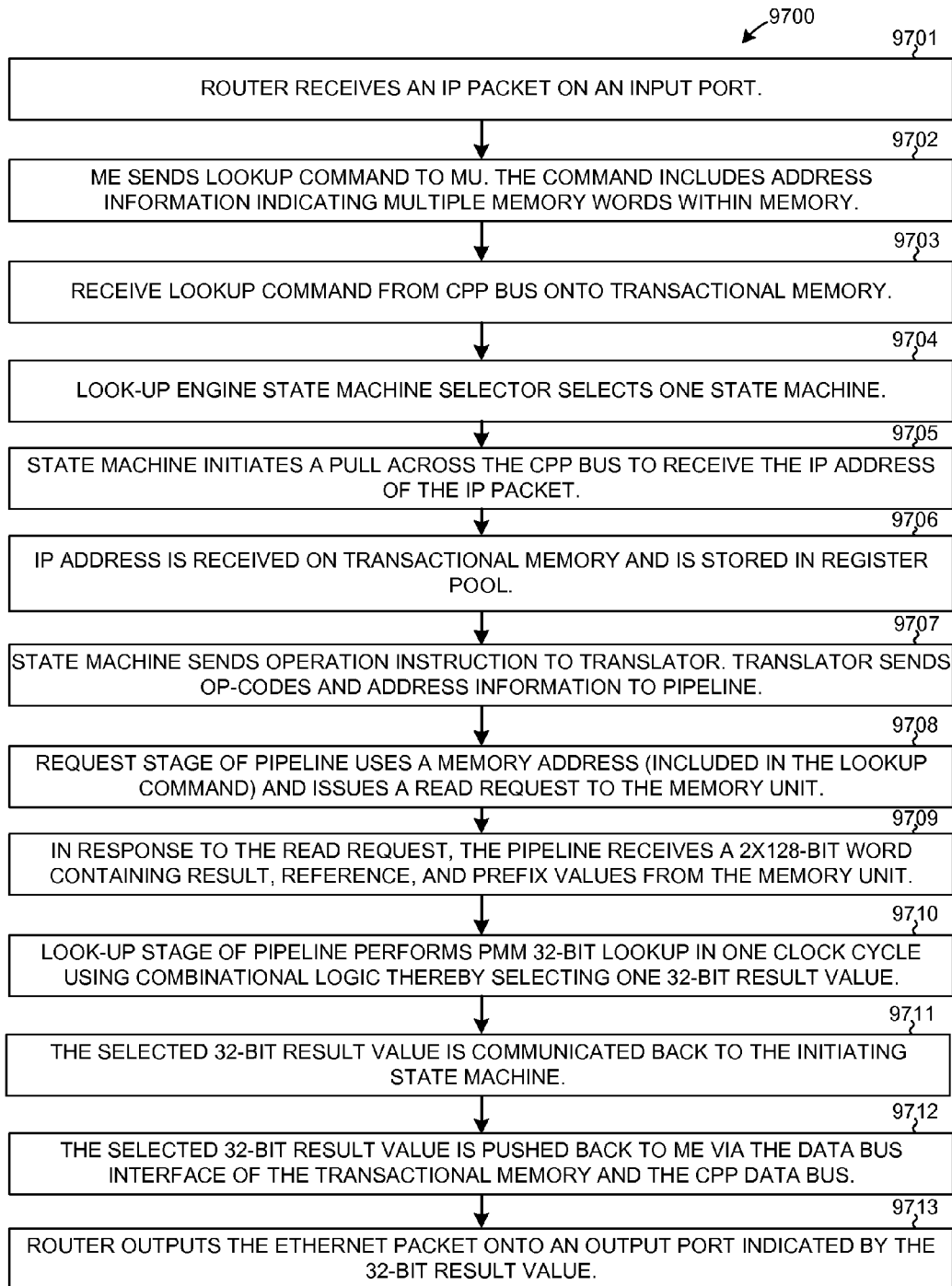
PMM 32-BIT LOOK-UP FLOWCHART FIG. 61
