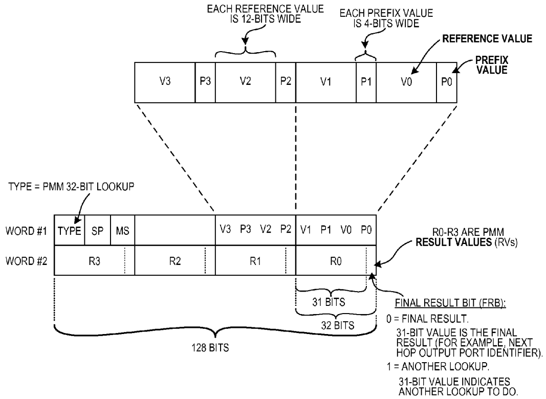
2X128 BITS READ OUT OF MEMORY UNIT
