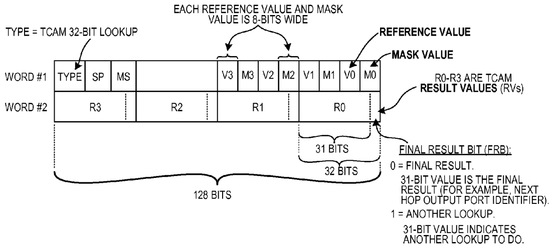
2X128 BITS READ OUT OF MEMORY UNIT FIG. 52
