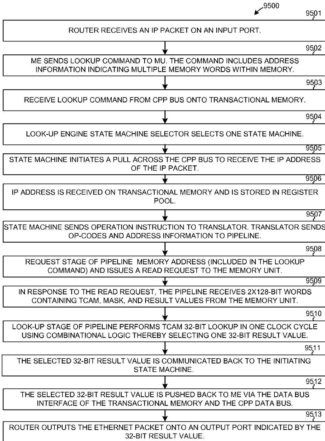
TCAM 32 BIT LOOK-UP FLOWCHART FIG. 55
