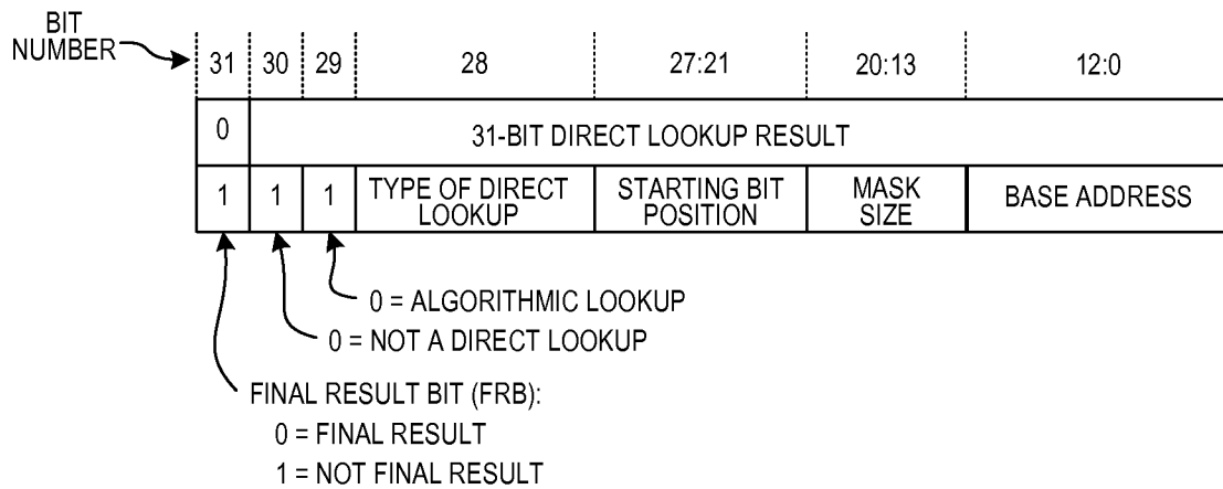
DIRECT RESULT VALUE FIG. 43
