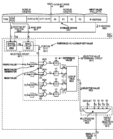
LOOKUP STAGE PERFORMING PPM 32-BIT LOOKUP
