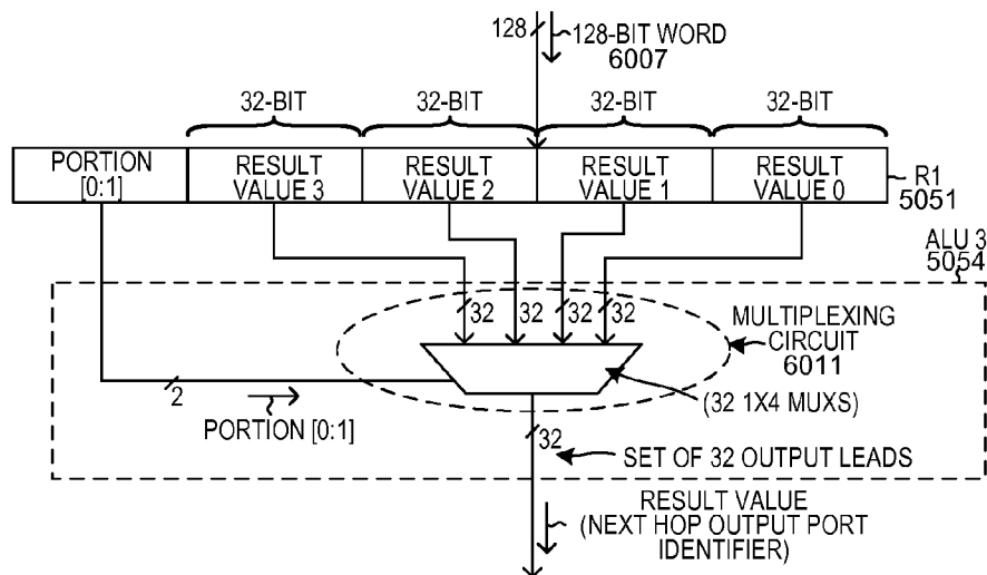
DIRECT 32-BIT LOOKUP STAGE FIG. 42
