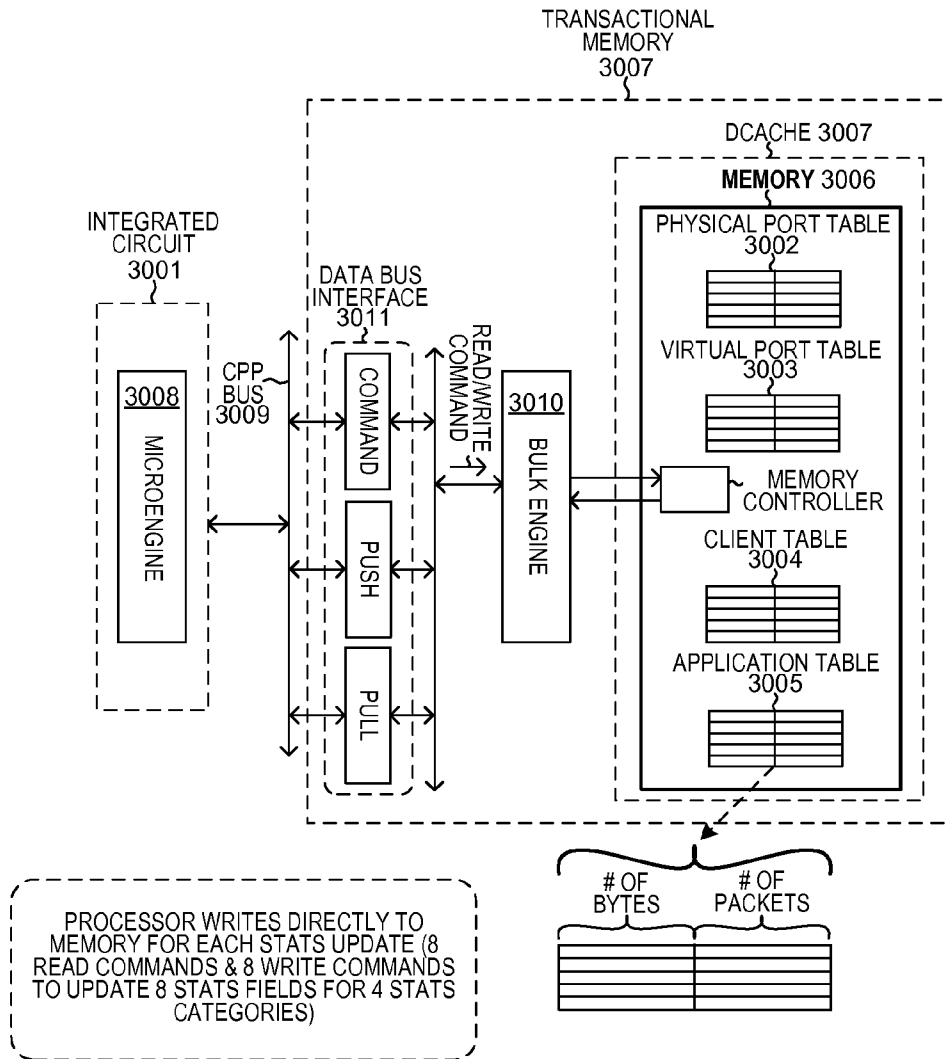
TRANSACTIONAL MEMORY PERFORMING COUNT UPDATE (PRIOR ART)
