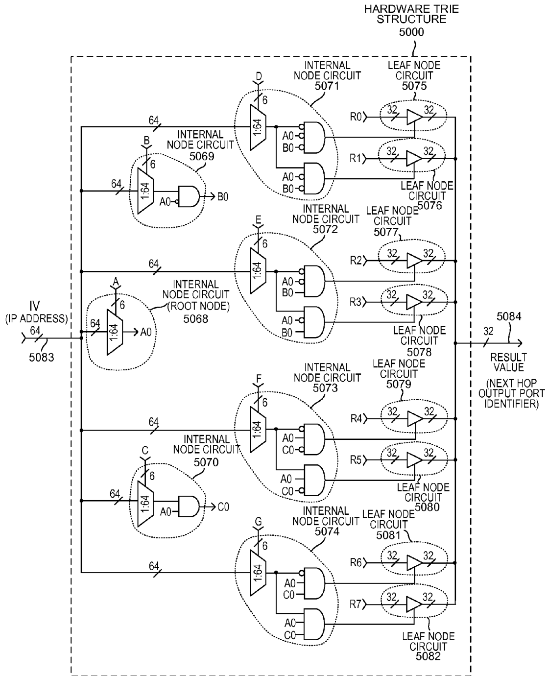
HARWARE TRIE STRUCTURE
