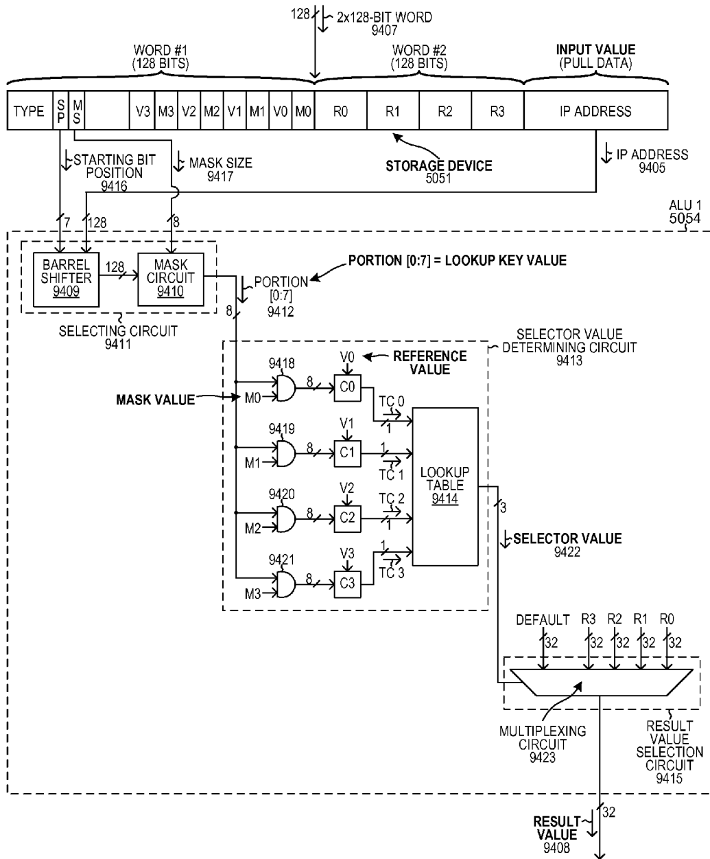
LOOKUP STAGE PERFORMING TCAM 32-BIT LOOKUP FIG. 53
