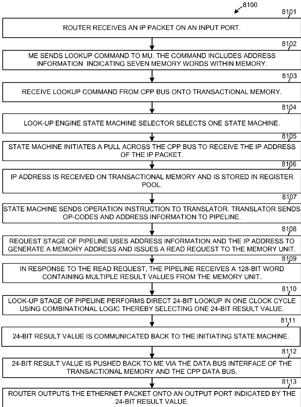
DIRECT 24-BIT LOOK-UP FLOWCHART FIG. 50
