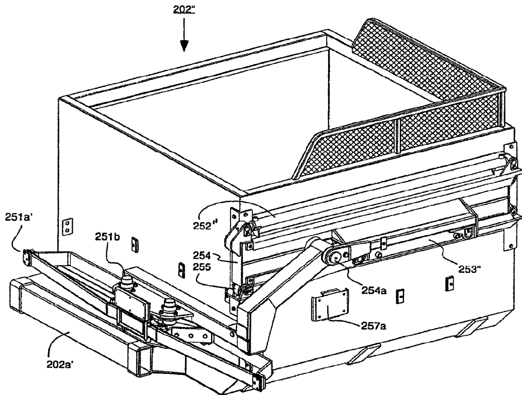
FIG. 2C (Prior Art)
