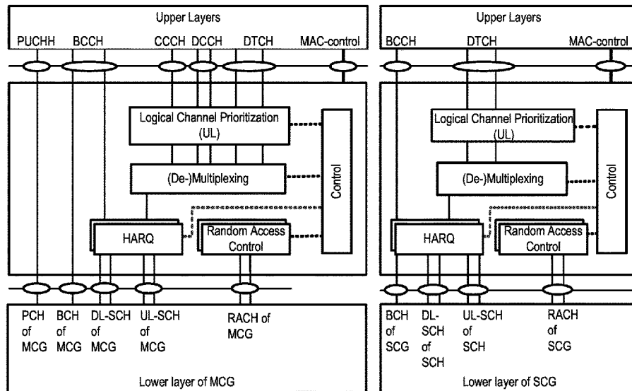
Dual-Connectivity- two MAC entities at UE side
