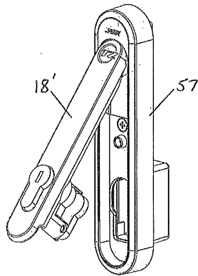
Step 2. Handle Raised
