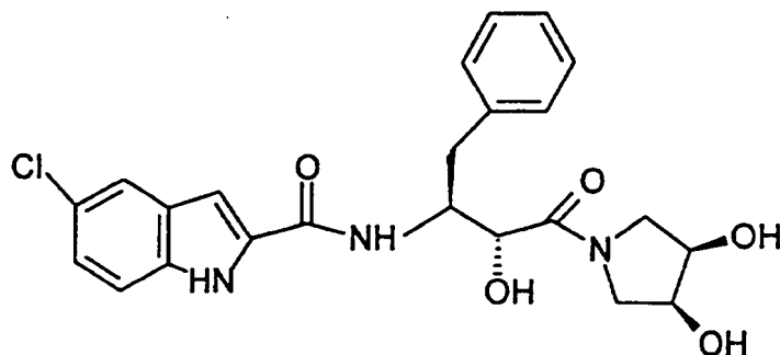
Compound 9
