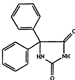
Compound 6
