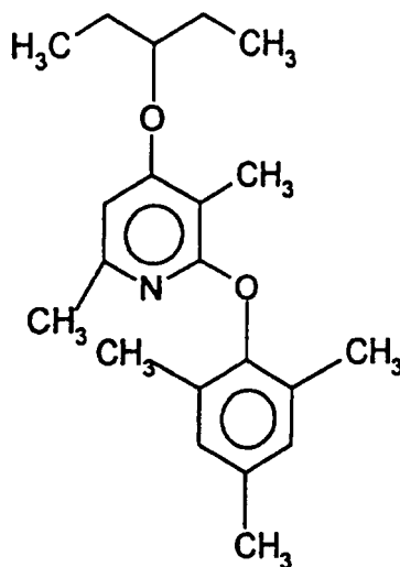
Compound 2
