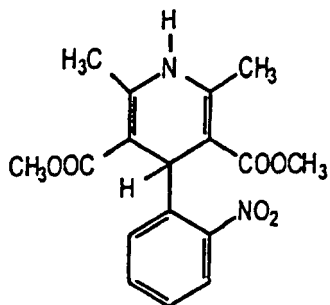
Compound 5
