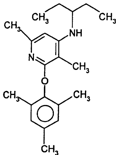
Compound 8
