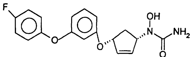
Compound 7
