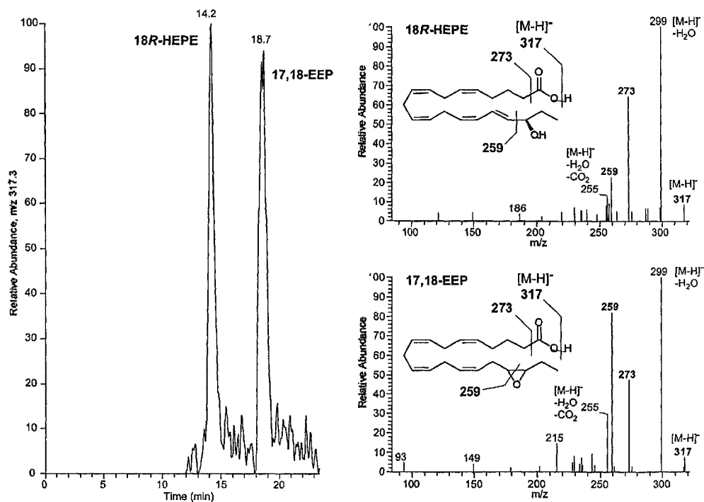
FIG. 3 Conversion of EPA by B. megaterium
