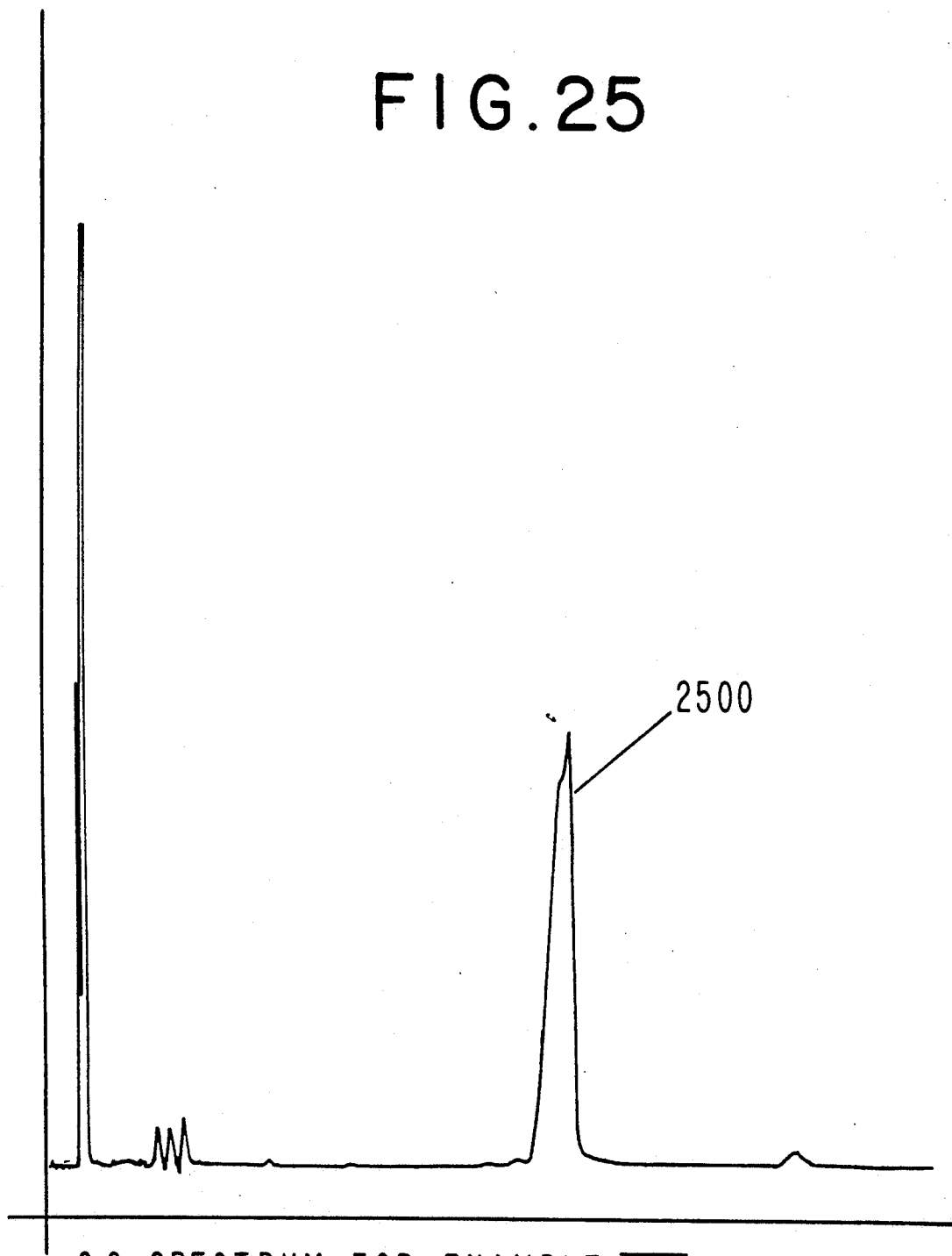
GC SPECTRUM FOR EXAMPLE VII .
