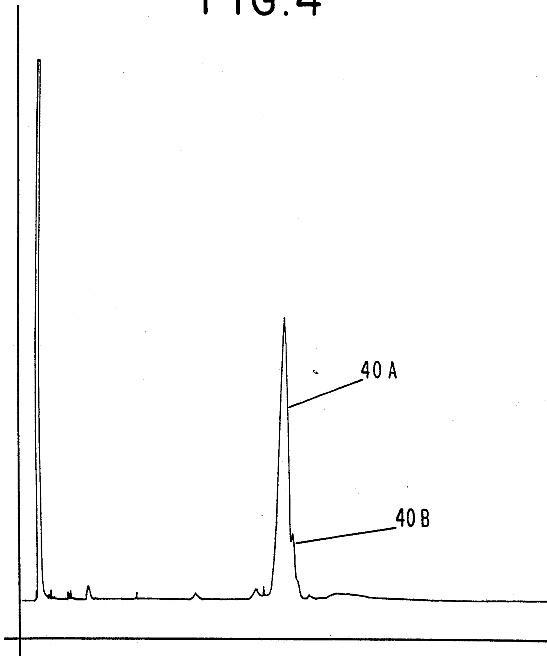
G C PROFILE FOR EXAMPLE II .
