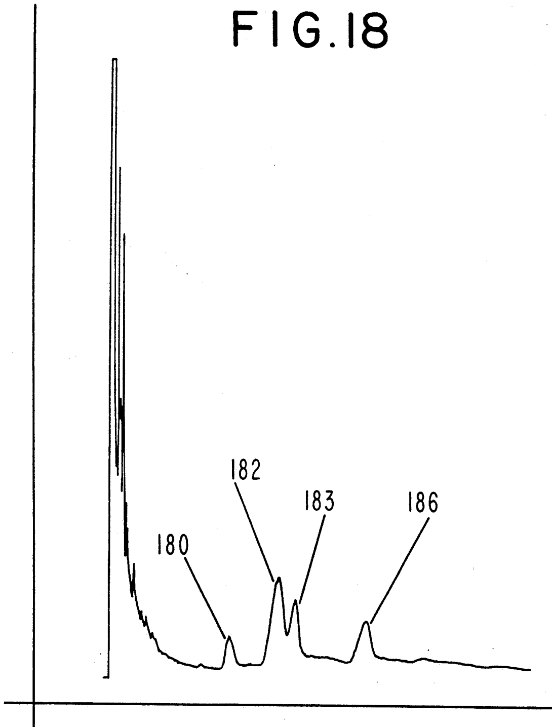
G. C. PROFILE FOR EXAMPLE VI .
