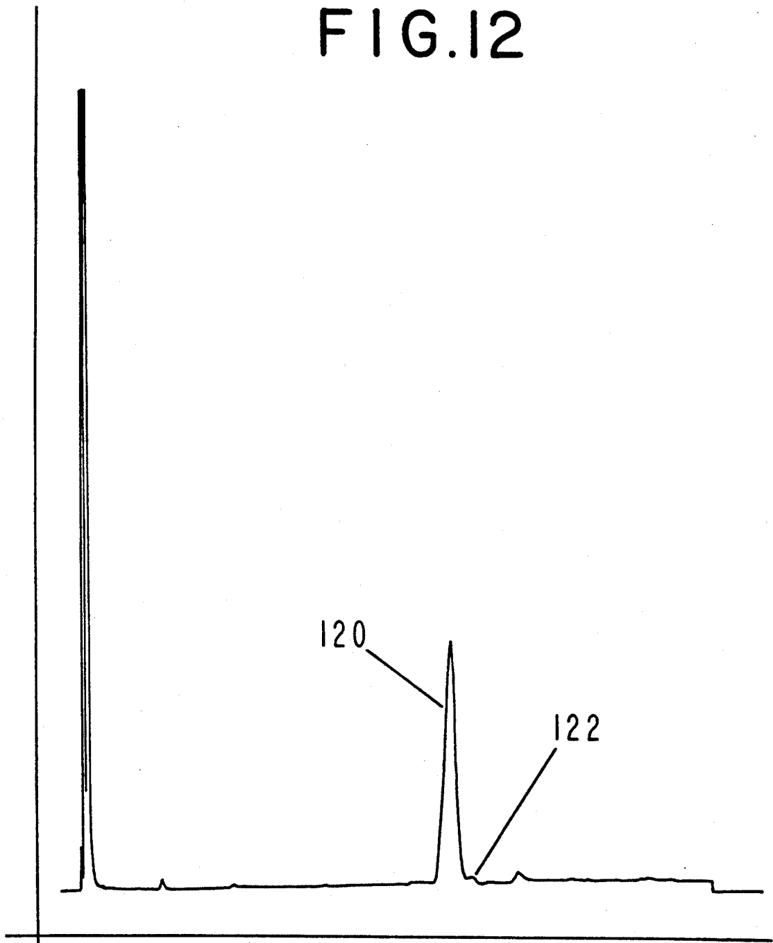
G C PROFILE FOR EXAMPLE IV .
