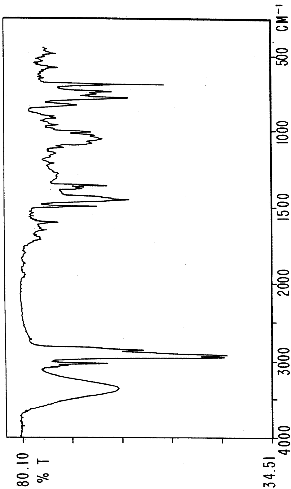
IR SPECTRUM FOR EXAMPLE V.
