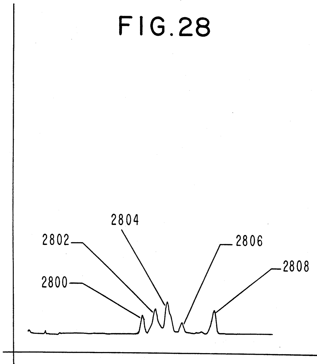
GC PROFILE FOR EXAMPLE VIII .
