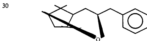
35 The peaks indicated by reference numerals 40A and 40B are for the compounds having the structures:
