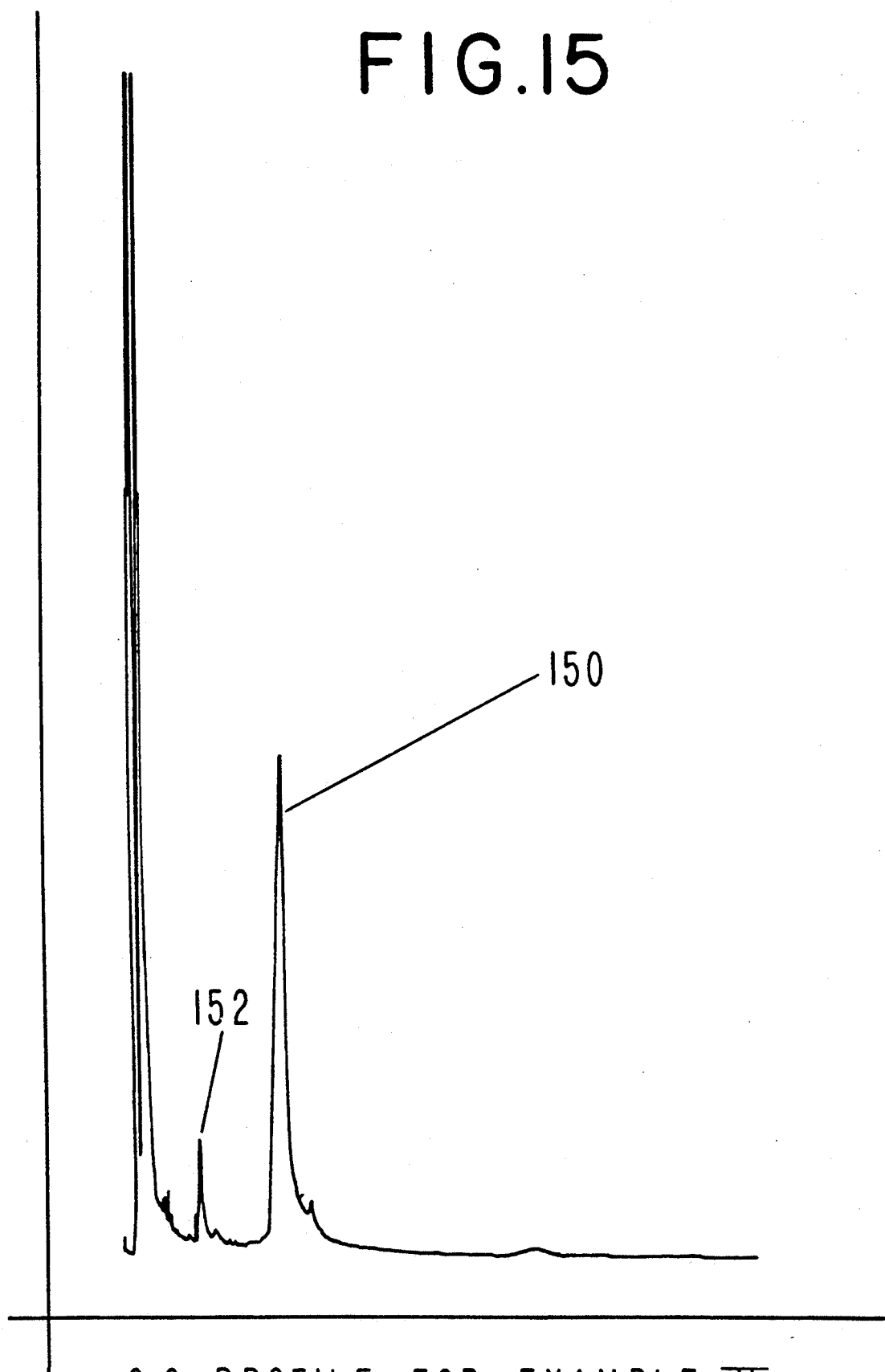
GC PROFILE FOR EXAMPLE V .
