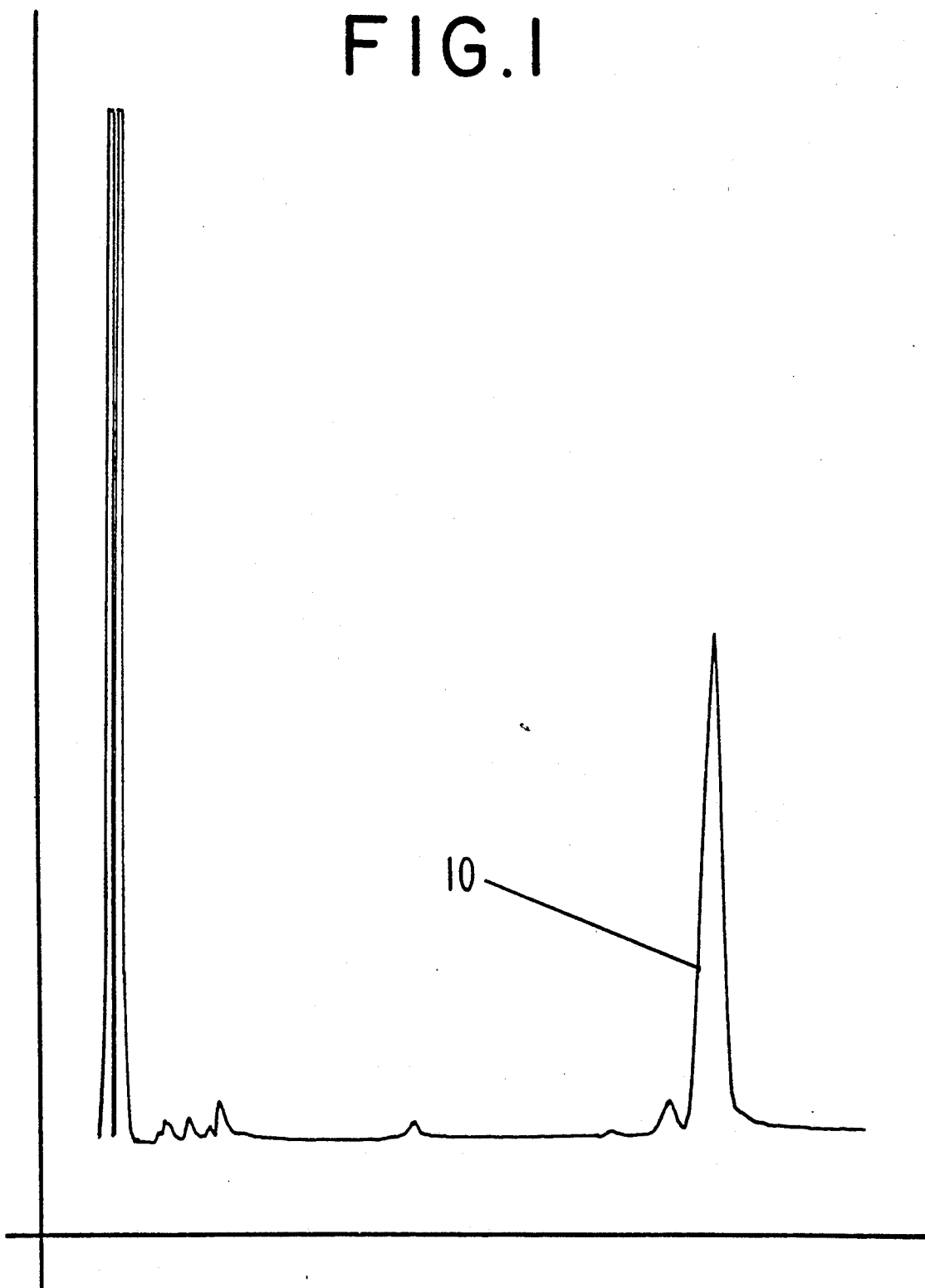
GC PROFILE FOR EXAMPLE I
