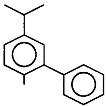
FIG. 30 is the NMR spectrum for the peak indicated by reference numeral 2802 of the GC spectrum of FIG. 28 for the compound having the structure:
