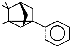
FIG. 32 is the infra-red spectrum for the peak indicated by reference numeral 2800 of the GC spectrum of FIG. 28 for the compound having the structure:
