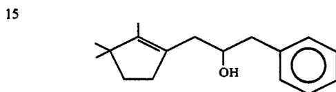
10 FIG. 4 is the GC profile for the reaction product of Example II containing the compounds having the structures:
