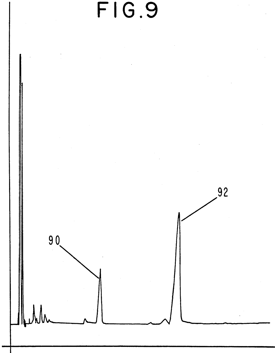
GC PROFILE FOR EXAMPLE III .
