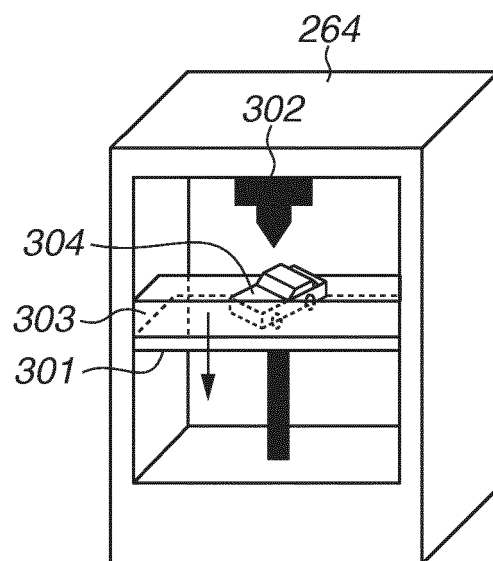
FIG.3B STEREOLITHOGRAPHY METHOD
