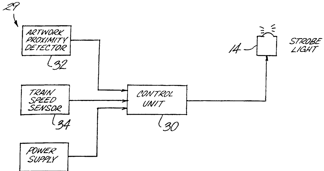
BLOCK DIAGRAM OF STROBE LIGHT CONTROL SYSTEM
